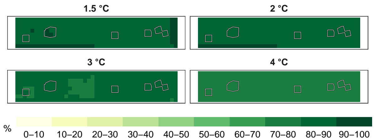
Figure 6: Percent reptiles remaining at 1 km resolution.
