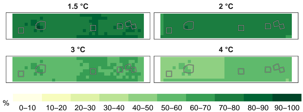
Figure 5: Percent mammals remaining at 1 km resolution.
