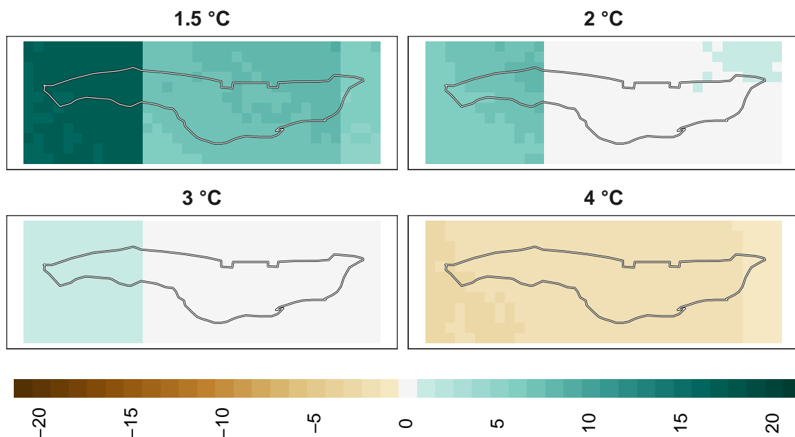
Figure 16: Adaptation effort for insects at 1 km resolution.
