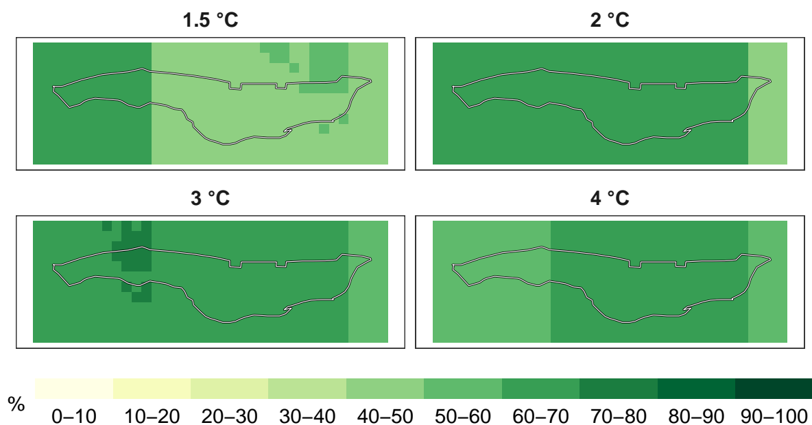
Figure 6: Percent timber species remaining at 1 km resolution.
