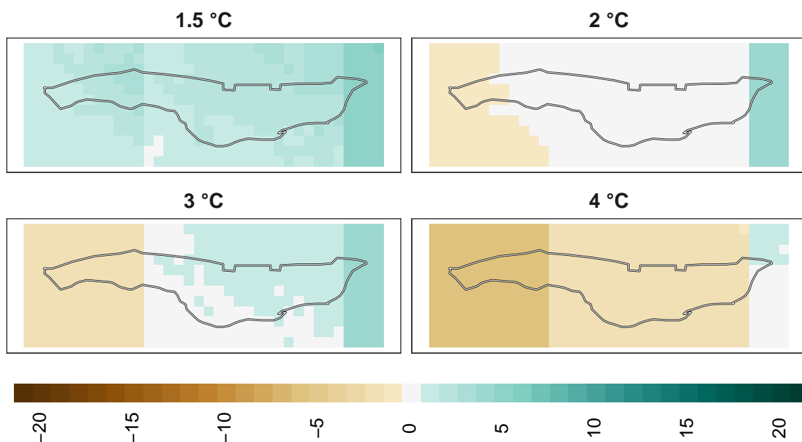
Figure 14: Adaptation effort for birds at 1 km resolution.
