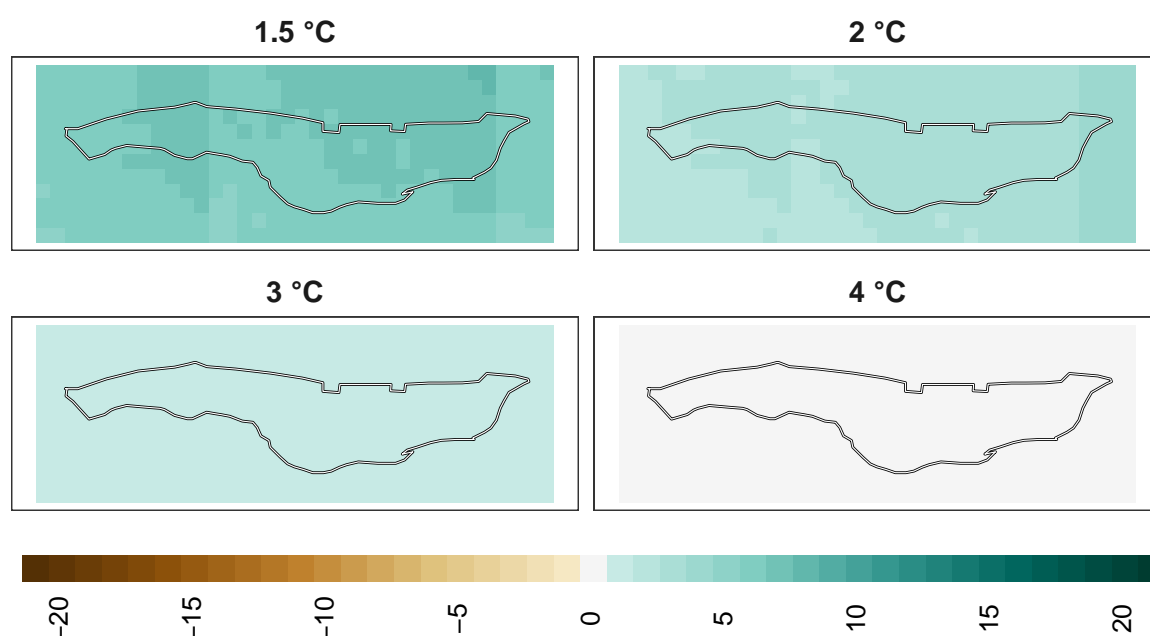
Figure 12: Adaptation effort for overall biodiversity at 1 km resolution.
