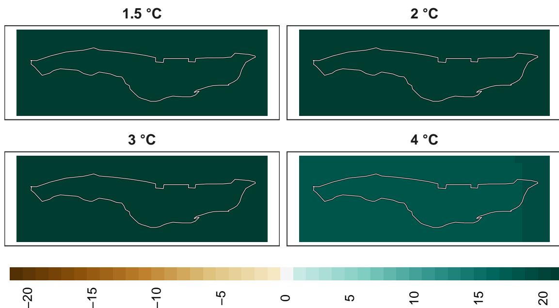
Figure 15: Adaptation effort for mammals at 1 km resolution.
