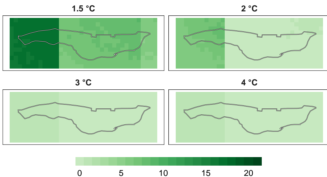
Figure 11: Number of models in agreement for insect refugia at 1 km resolution.
