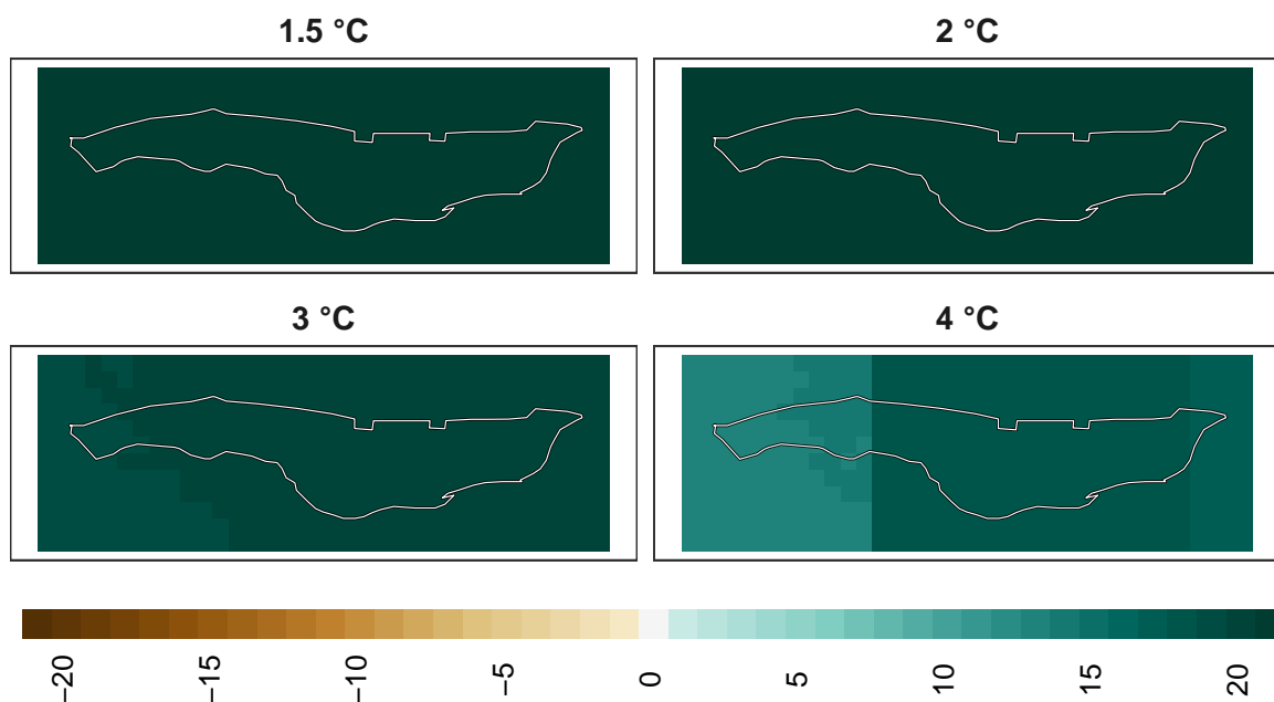
Figure 13: Adaptation effort for plants at 1 km resolution.
