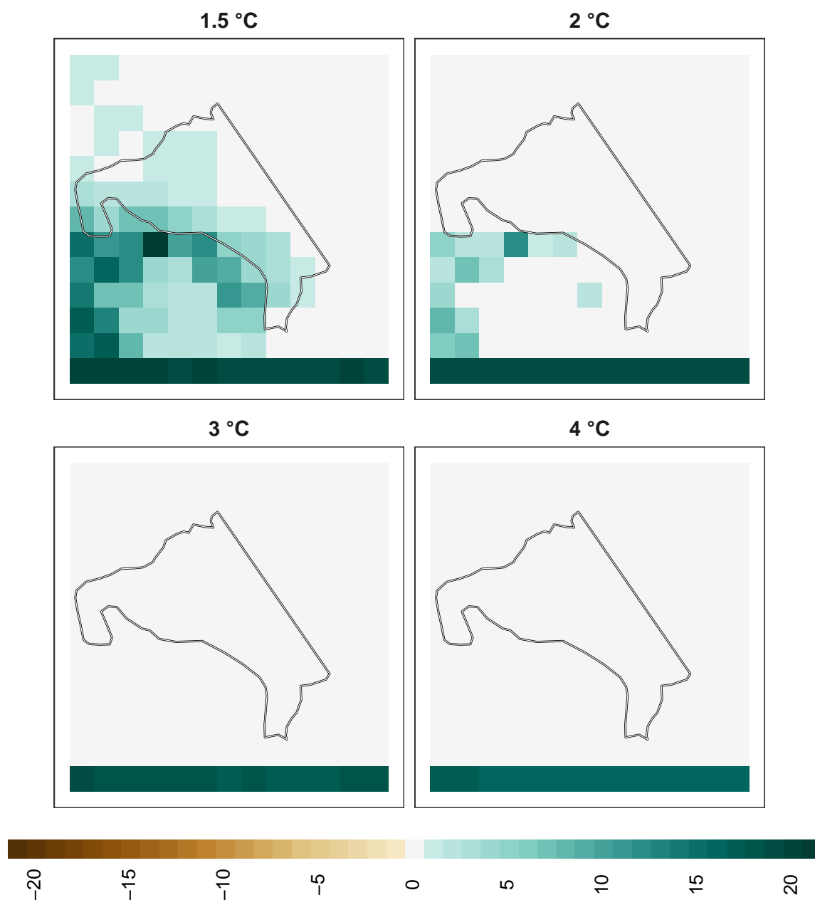
Figure 16: Adaptation effort for amphibians at 1 km resolution.
