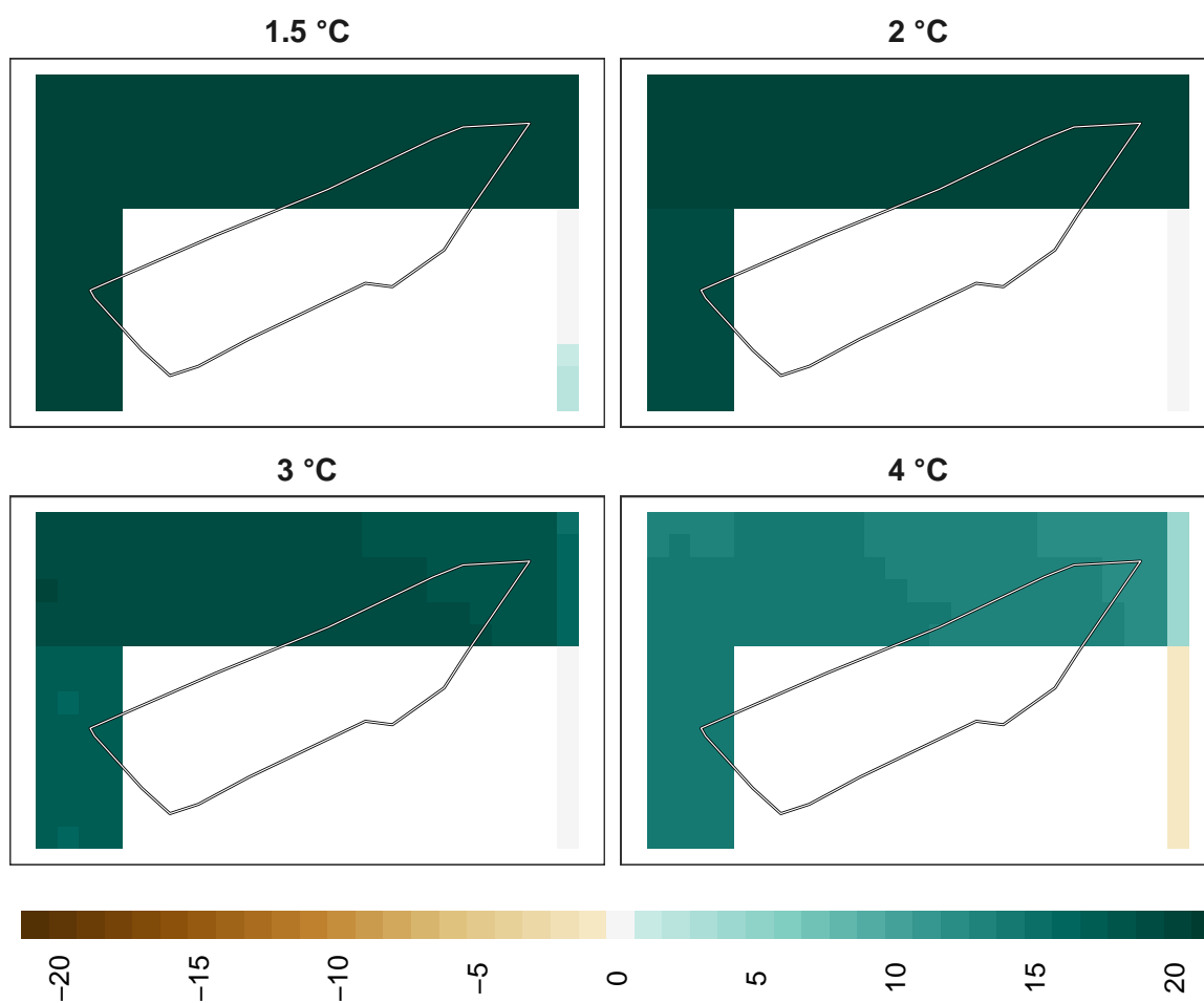
Figure 16: Adaptation effort for amphibians at 1 km resolution.
