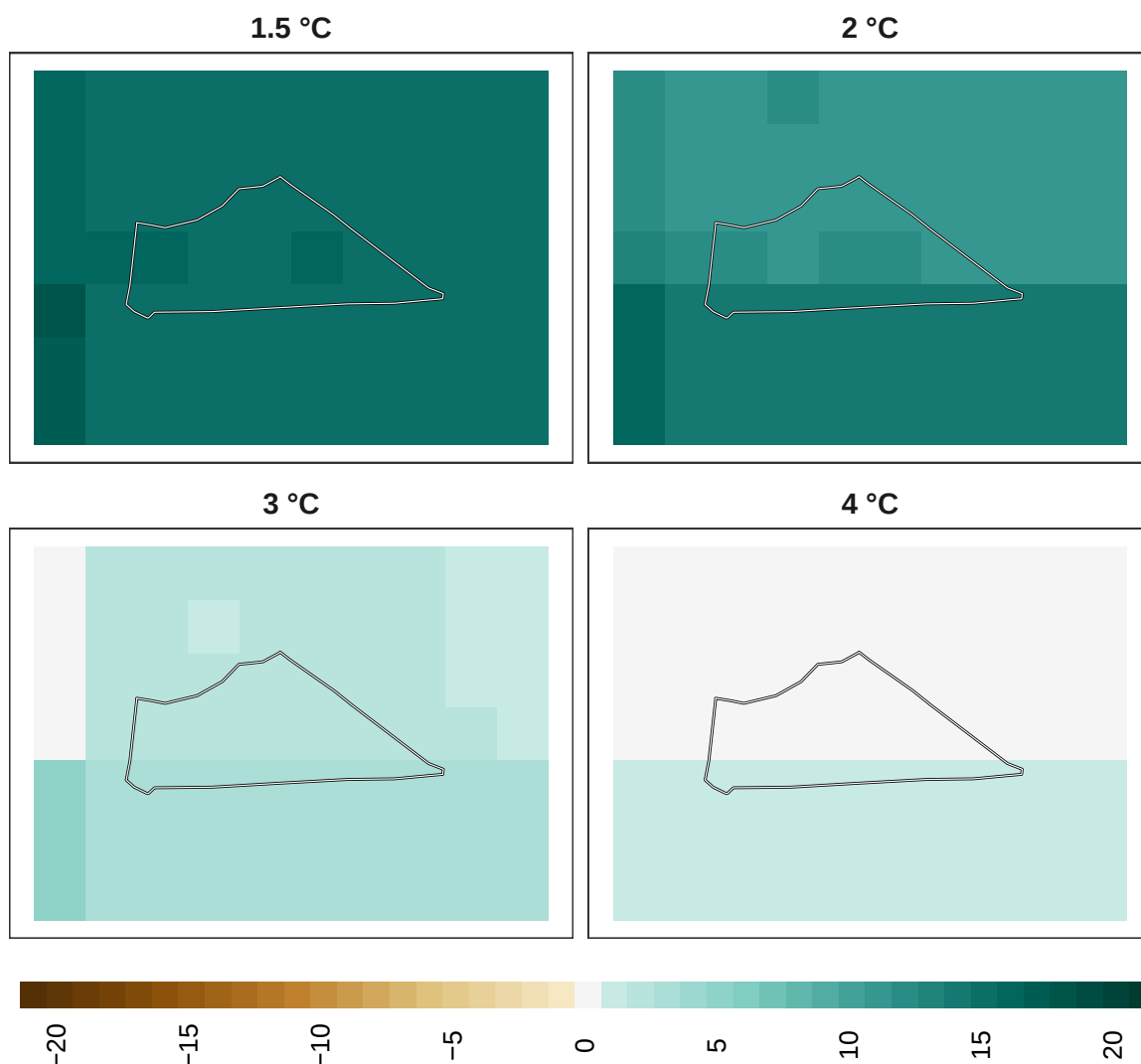
Figure 13: Adaptation effort for plants at 1 km resolution.
