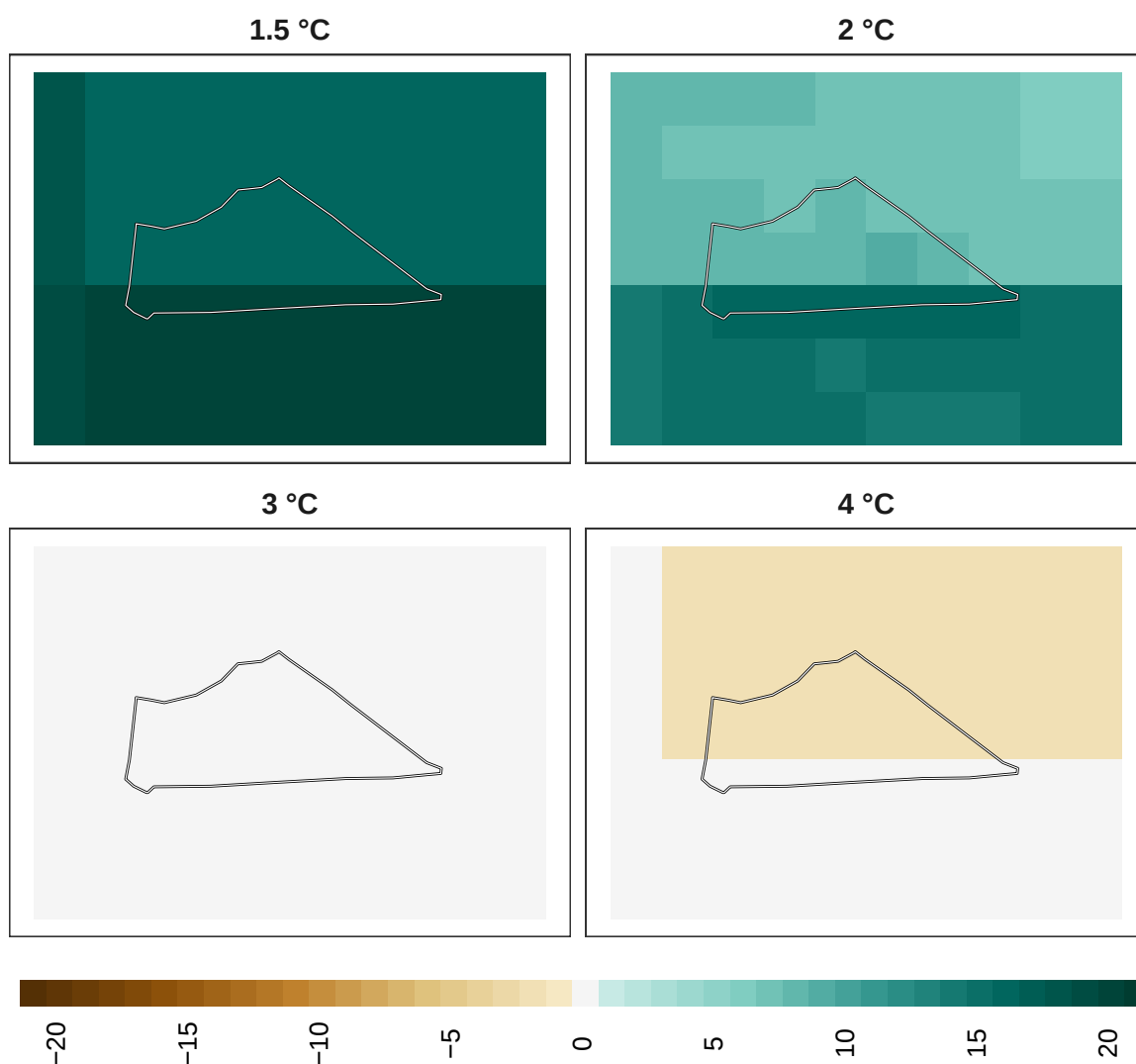
Figure 15: Adaptation effort for mammals at 1 km resolution.
