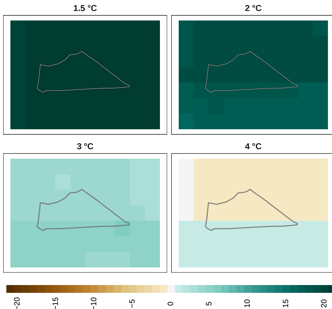
Figure 16: Adaptation effort for insects at 1 km resolution.
