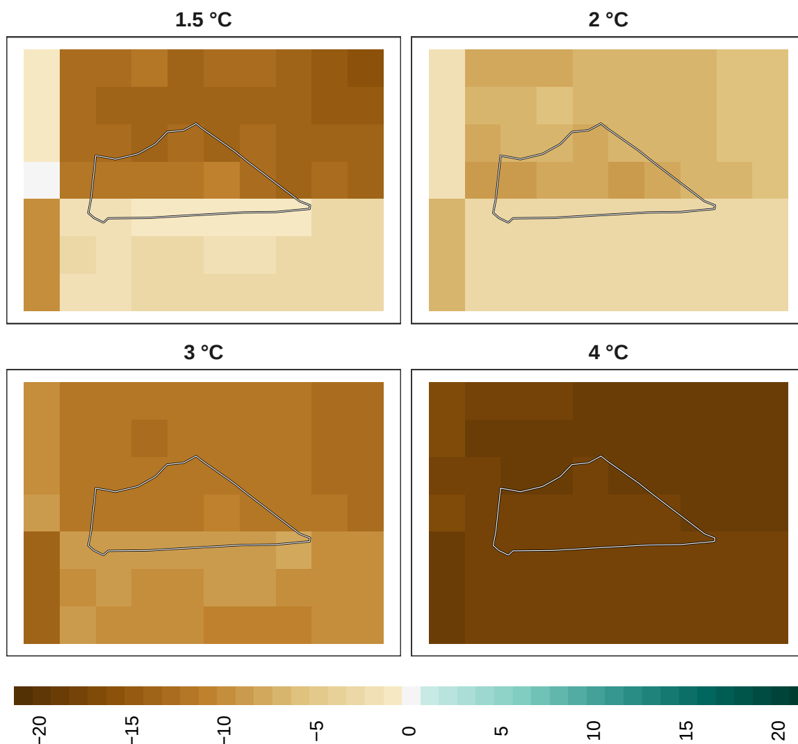
Figure 14: Adaptation effort for birds at 1 km resolution.
