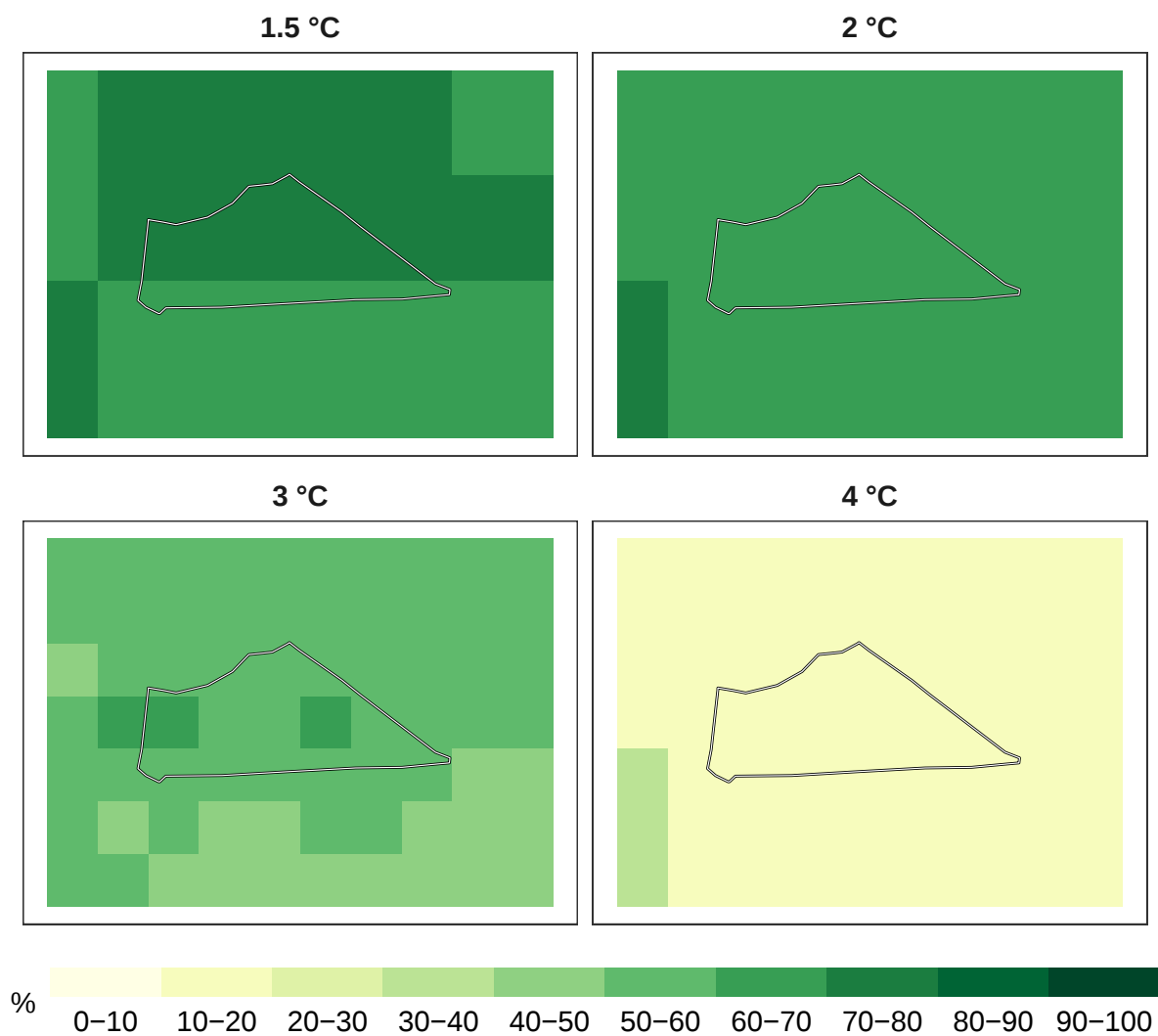
Figure 6: Percent timber species remaining at 1 km resolution.
