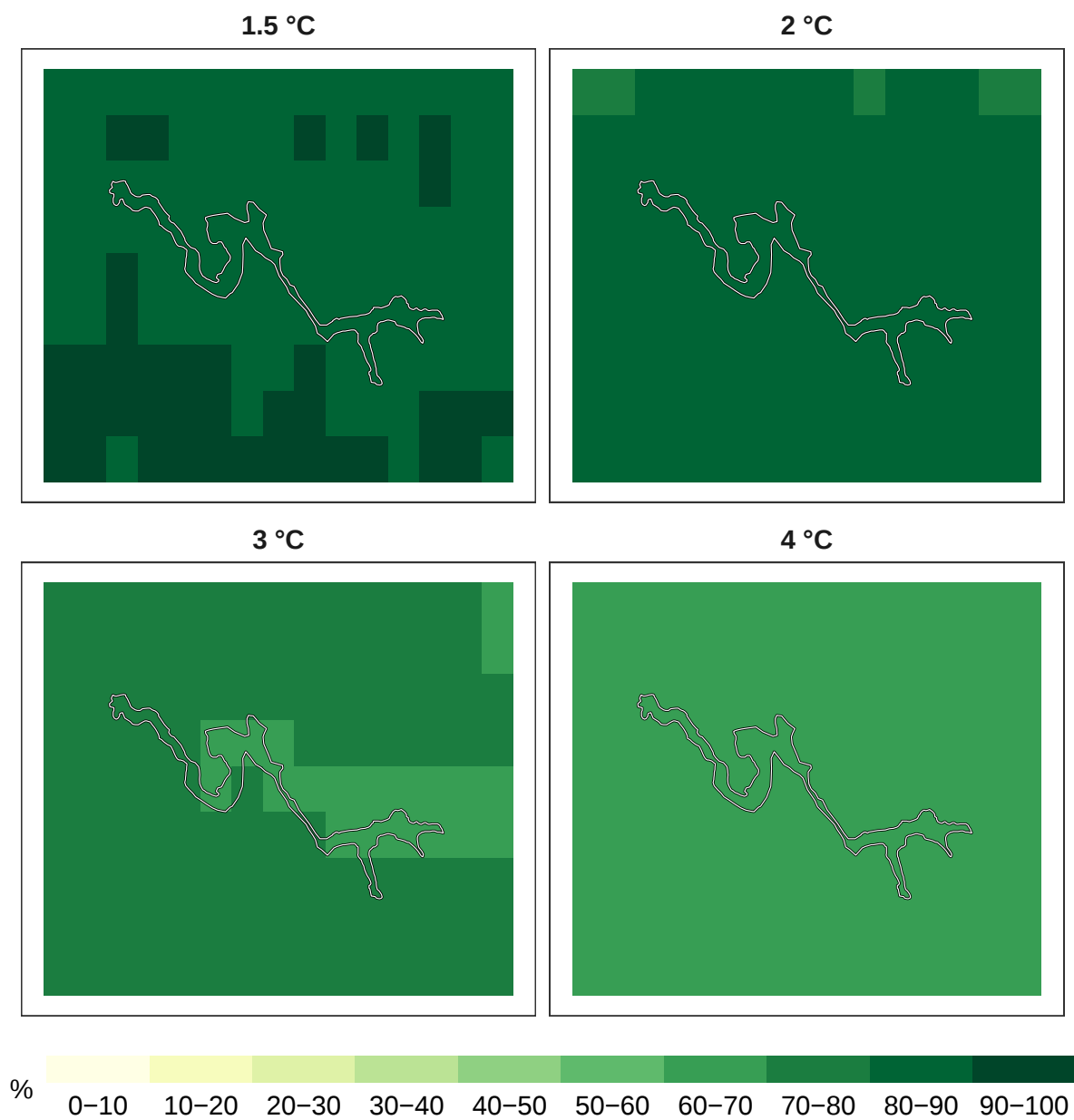
Figure 6: Percent reptiles remaining at 1 km resolution.
