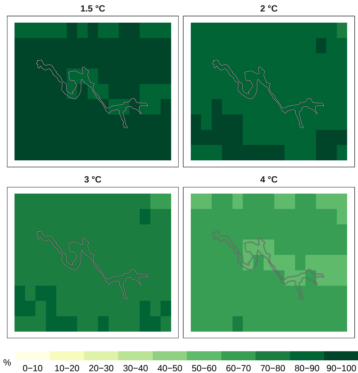
Figure 4: Percent birds remaining at 1 km resolution.
