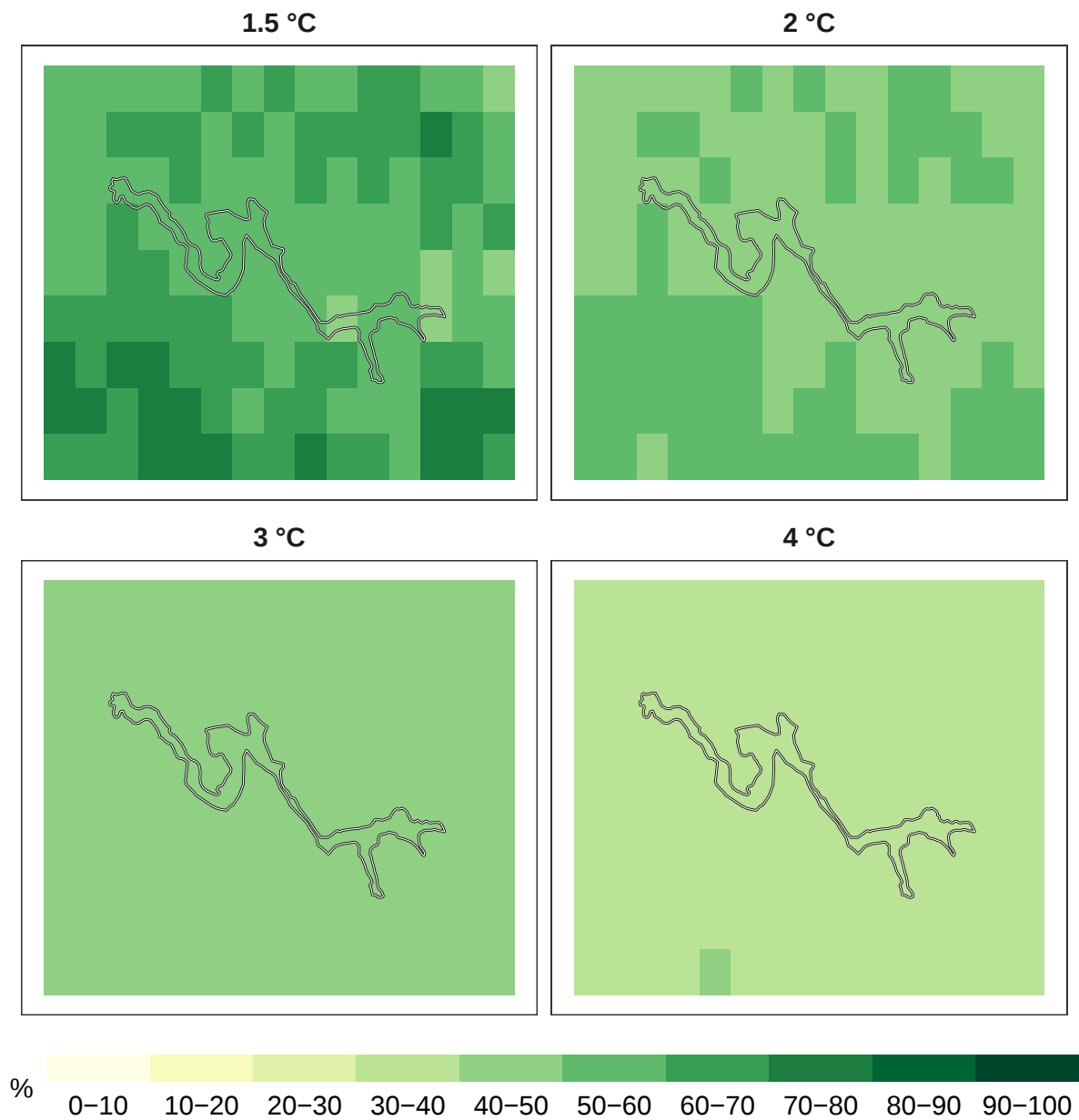
Figure 8: Percent pollinators remaining at 1 km resolution.
