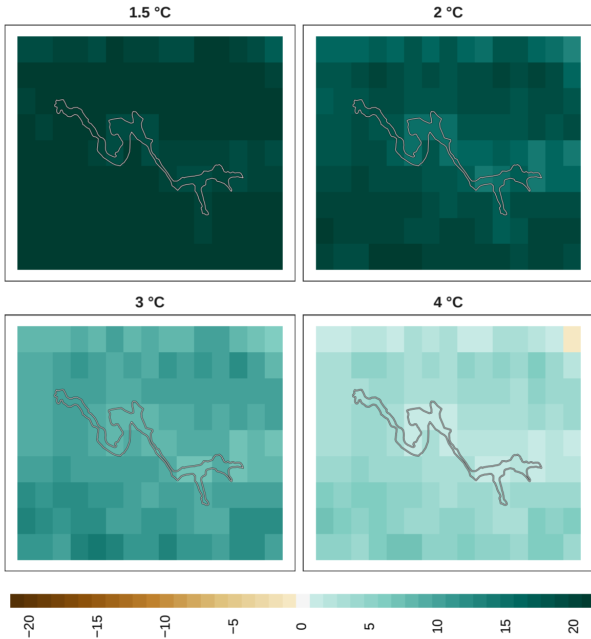
Figure 21: Adaptation effort for birds at 1 km resolution.
