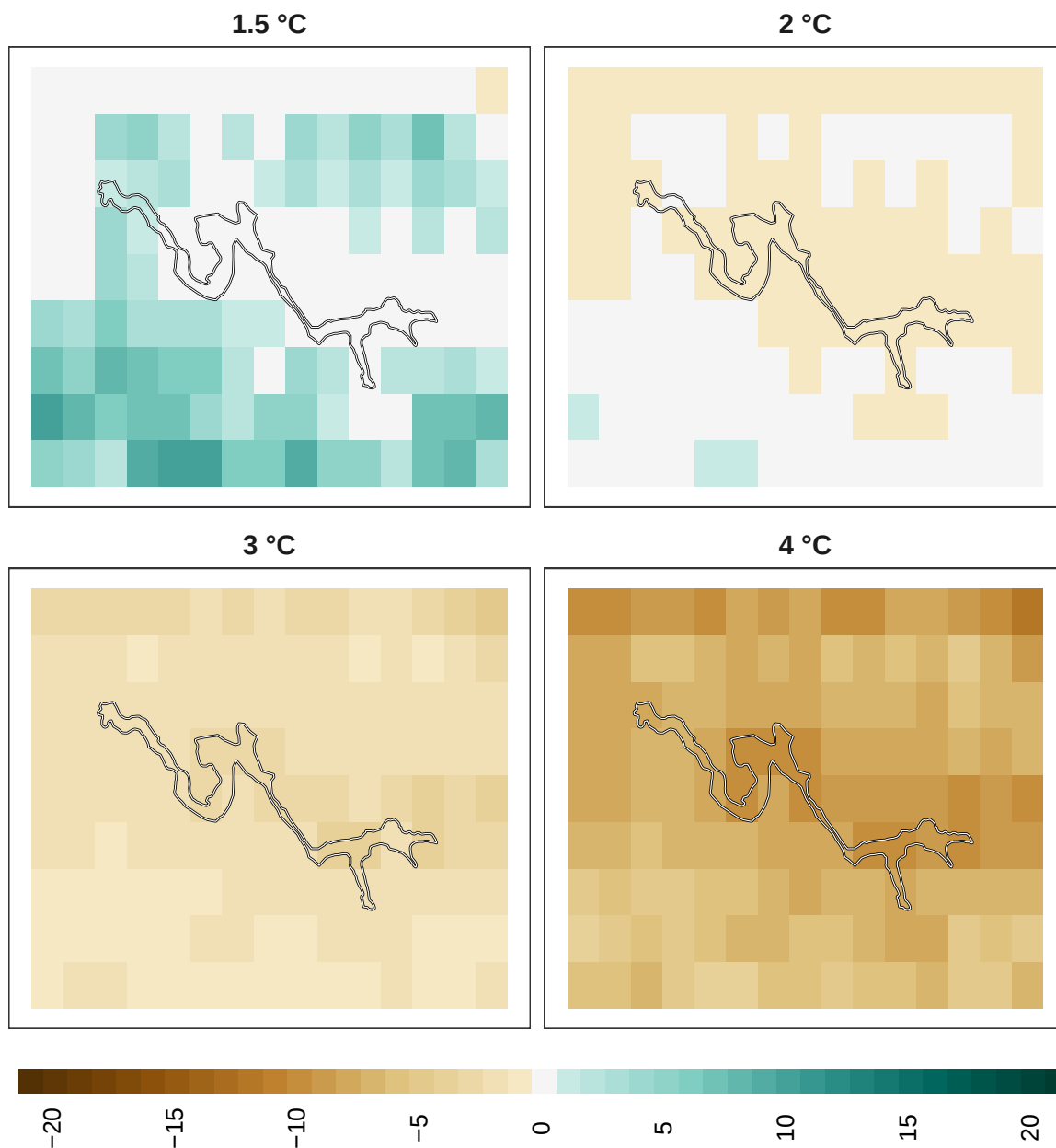
Figure 18: Adaptation effort for overall biodiversity at 1 km resolution.
