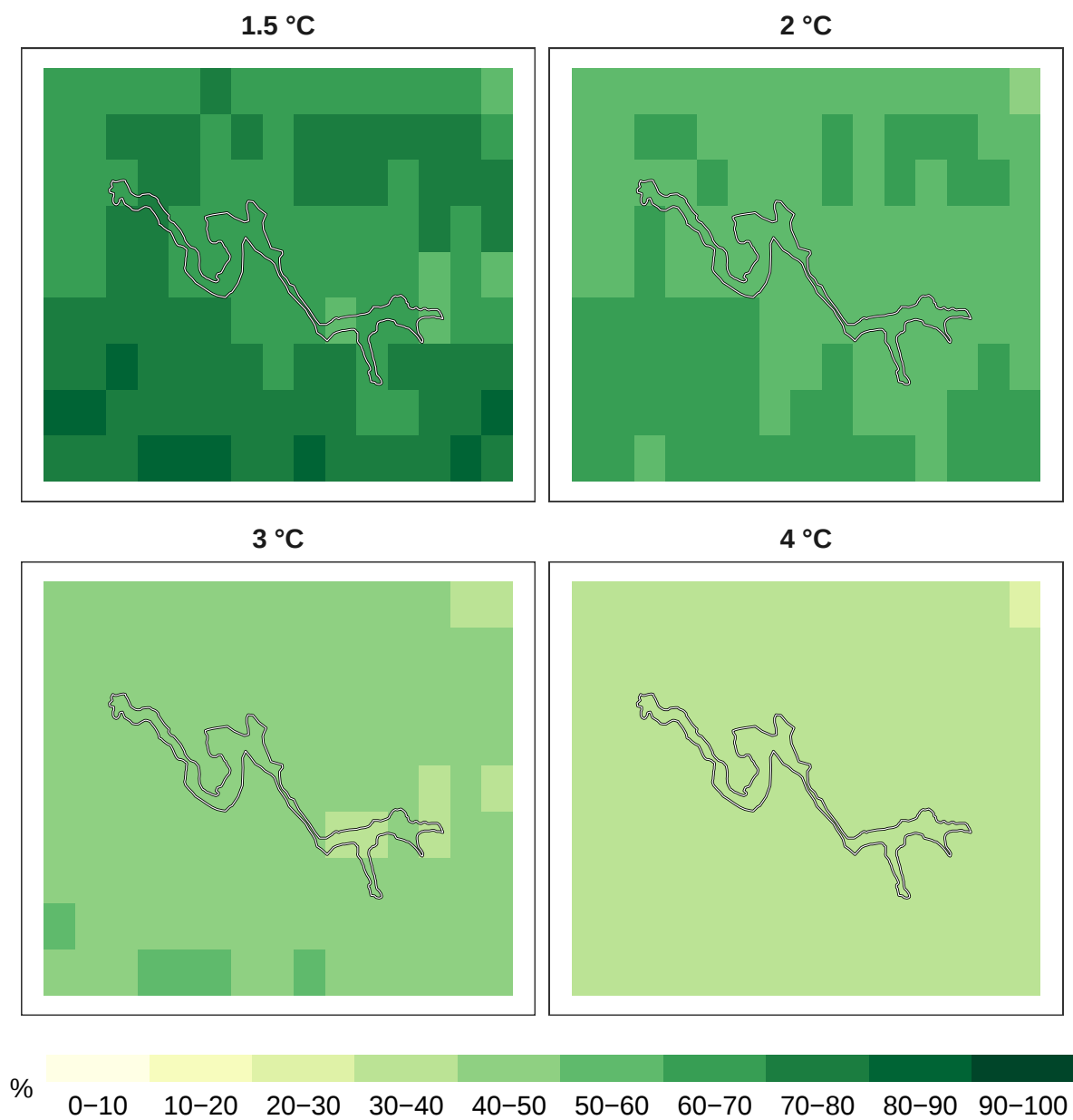
Figure 2: Percent plants remaining at 1 km resolution.
