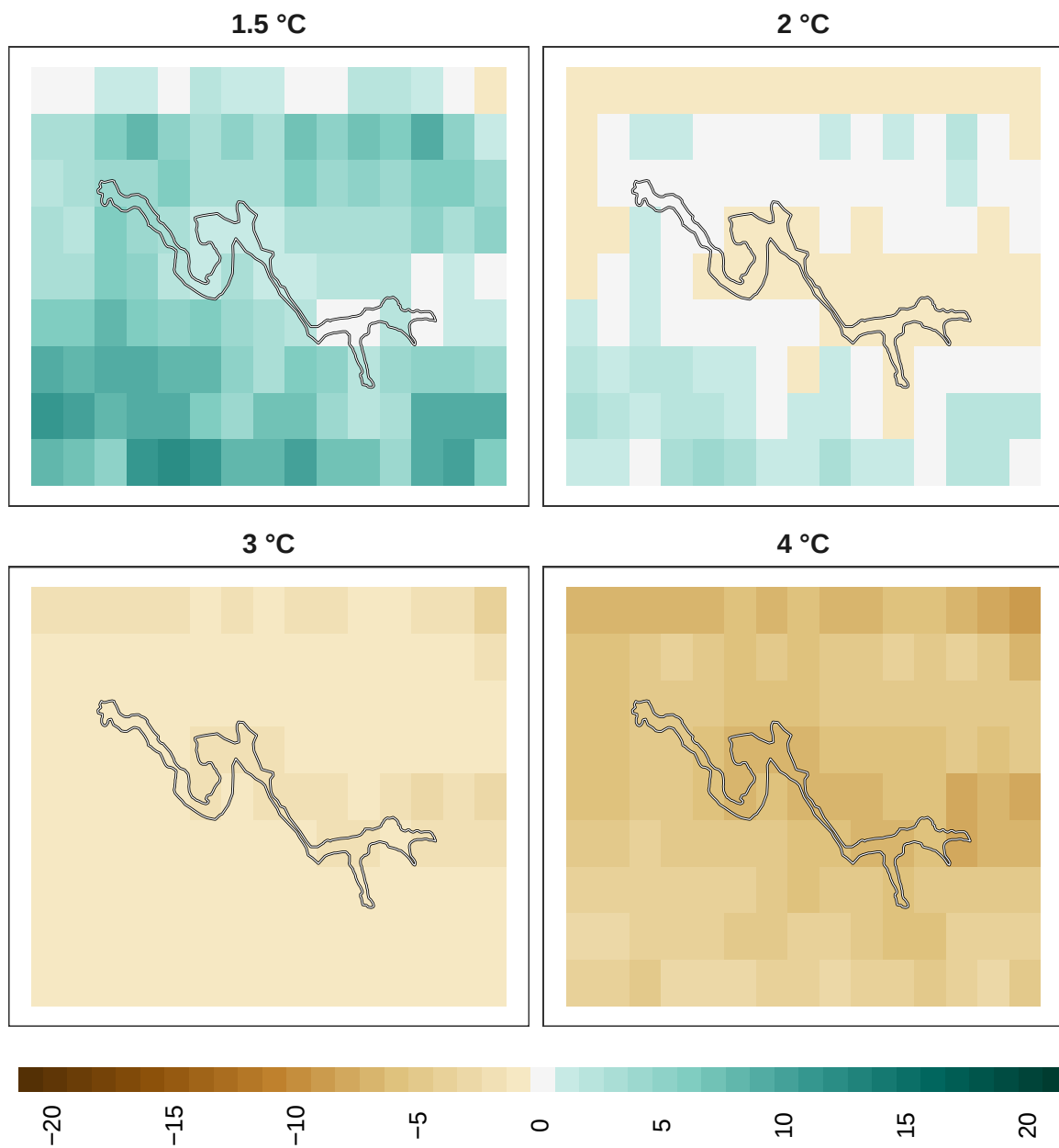
Figure 19: Adaptation effort for plants at 1 km resolution.
