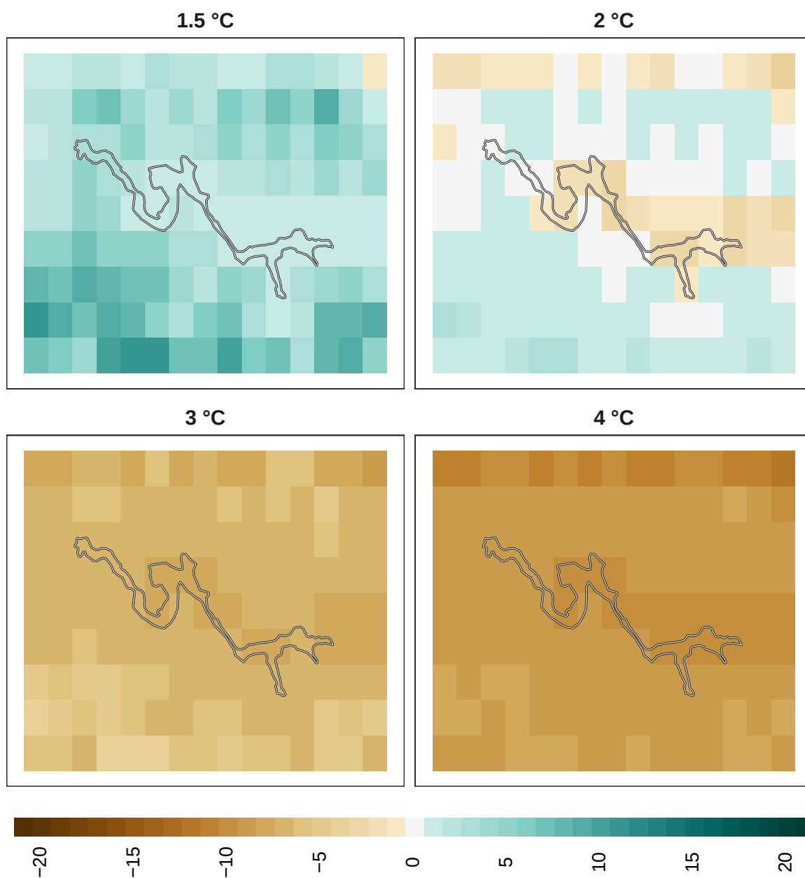
Figure 22: Adaptation effort for mammals at 1 km resolution.
