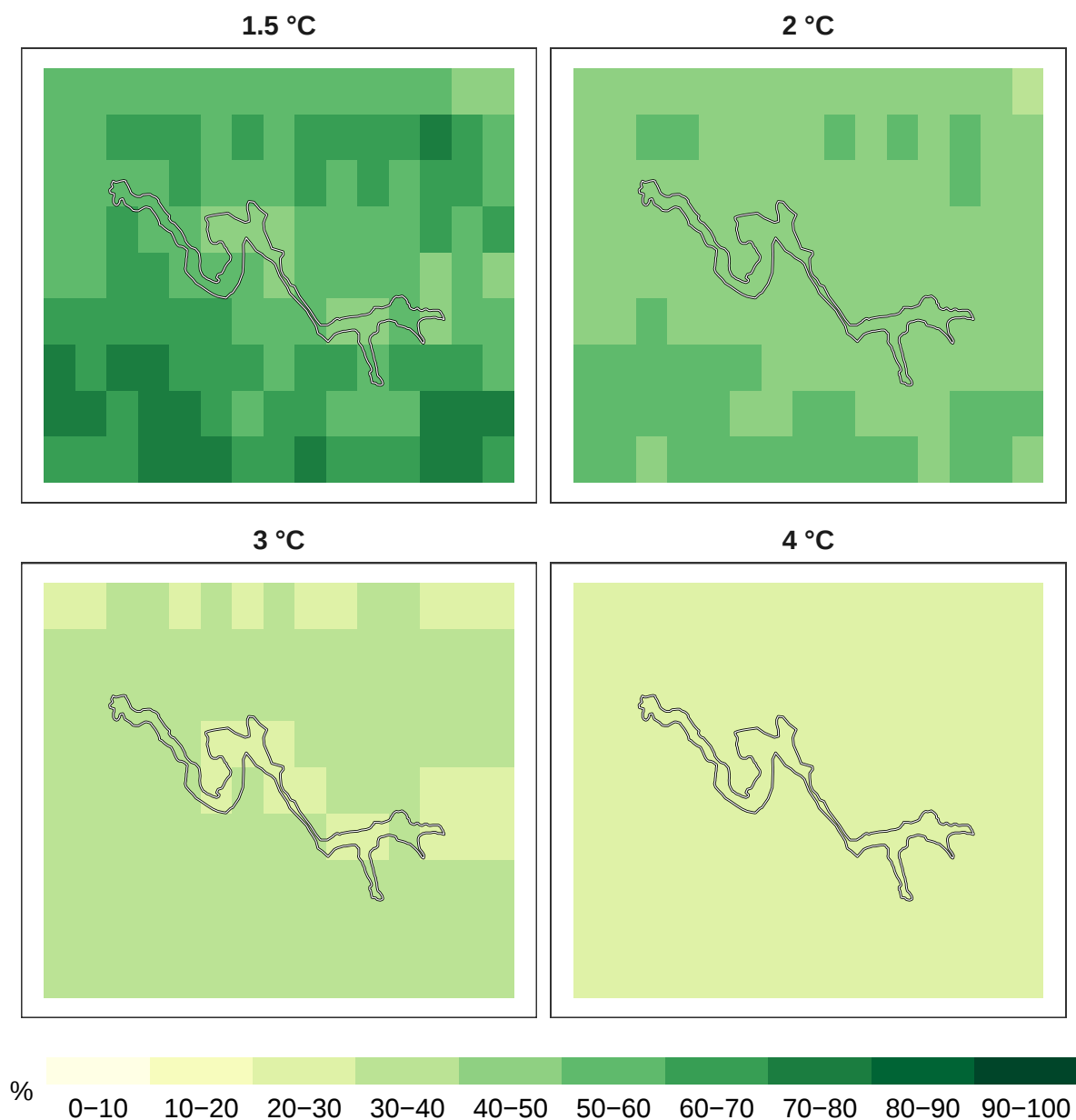
Figure ES1: Percent overall biodiversity remaining at 1 km resolution.
