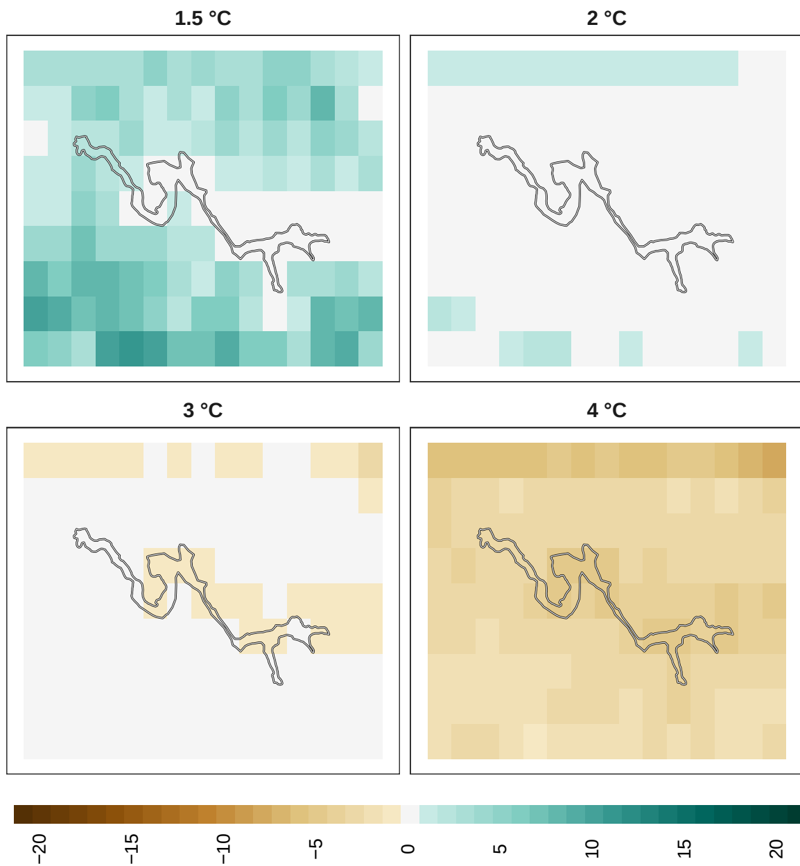
Figure 25: Adaptation effort for pollinators at 1 km resolution.
