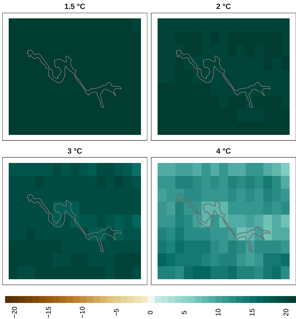
Figure 20: Adaptation effort for amphibians at 1 km resolution.
