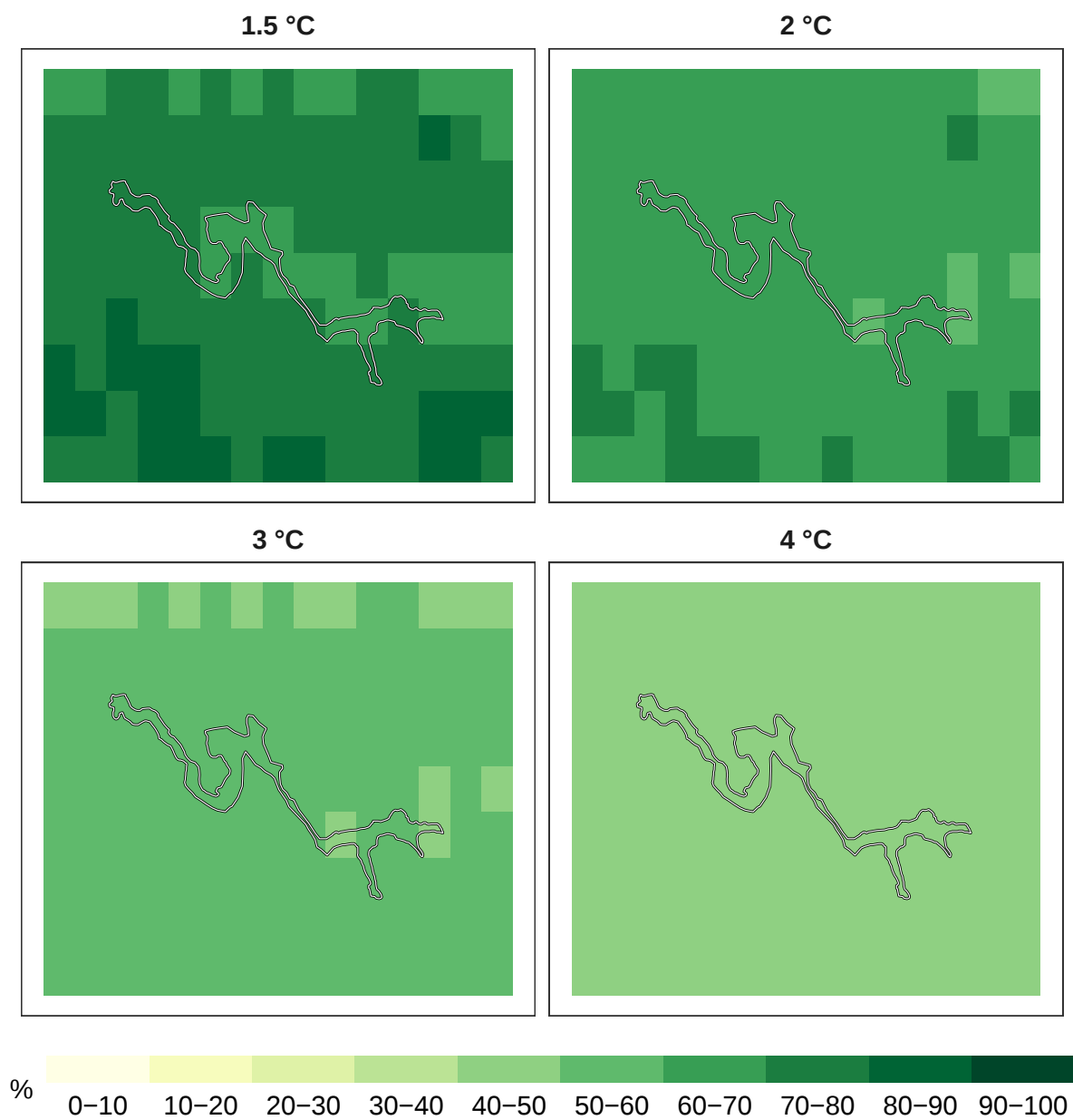
Figure 9: Percent timber species remaining at 1 km resolution.
