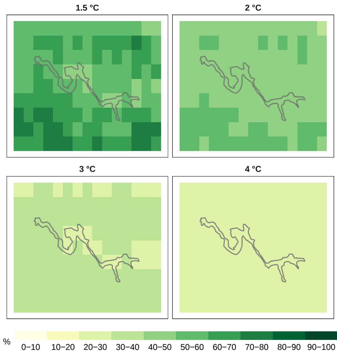
Figure 1: Percent overall biodiversity remaining at 1 km resolution.
