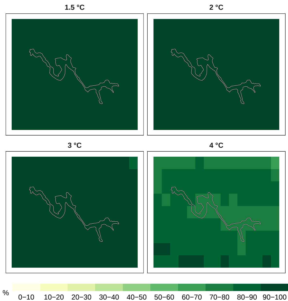
Figure 3: Percent amphibians remaining at 1 km resolution.
