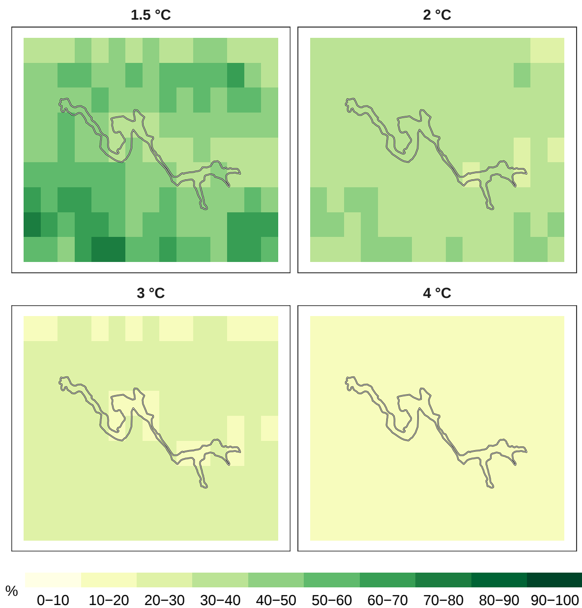
Figure 7: Percent insects remaining at 1 km resolution.
