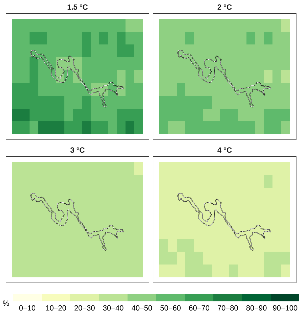
Figure 5: Percent mammals remaining at 1 km resolution.
