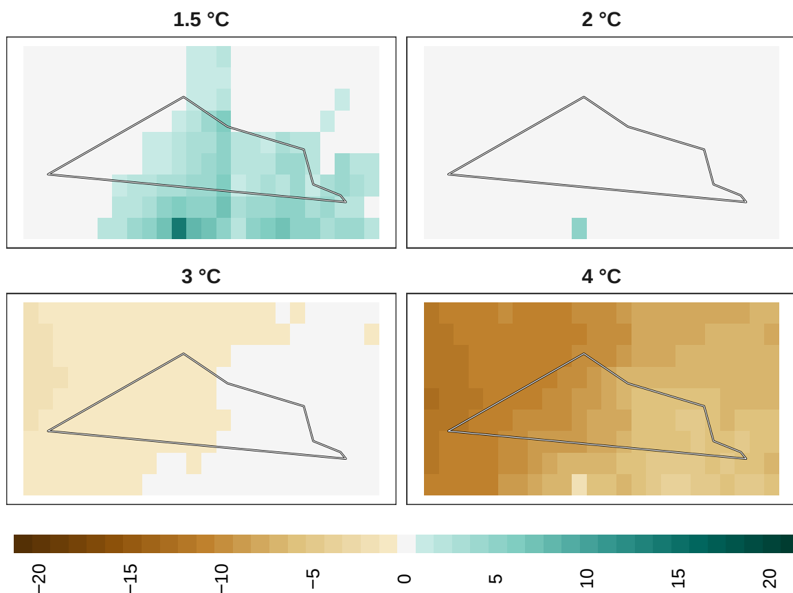
Figure 13: Adaptation effort for overall biodiversity at 1 km resolution.
