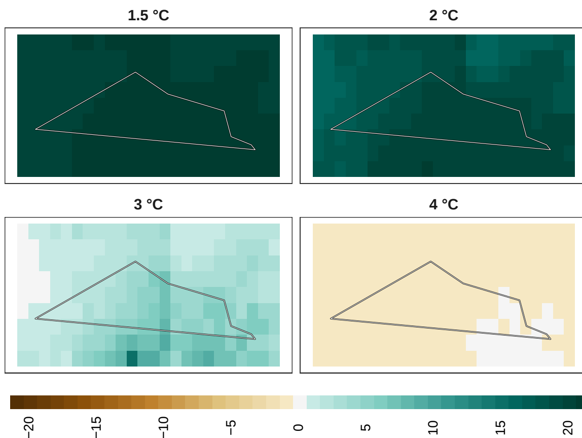
Figure 16: Adaptation effort for mammals at 1 km resolution.
