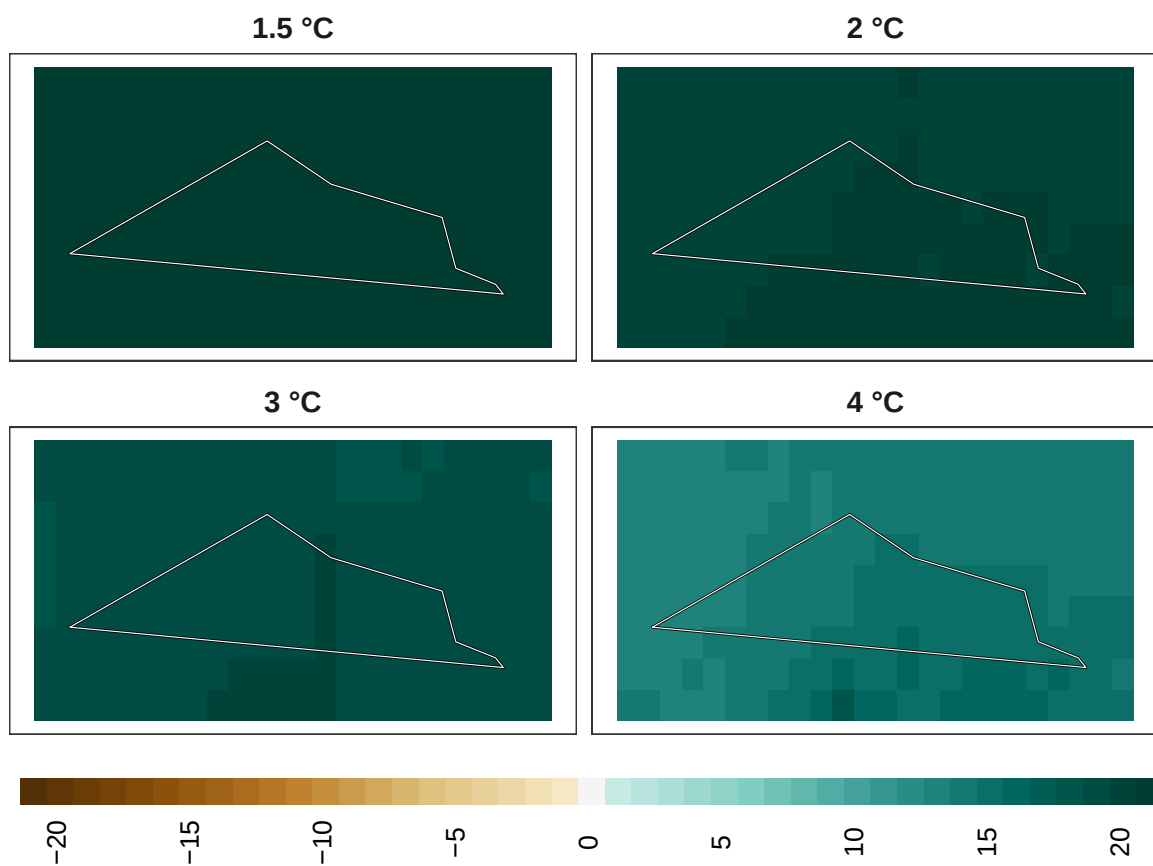
Figure 17: Adaptation effort for reptiles at 1 km resolution.
