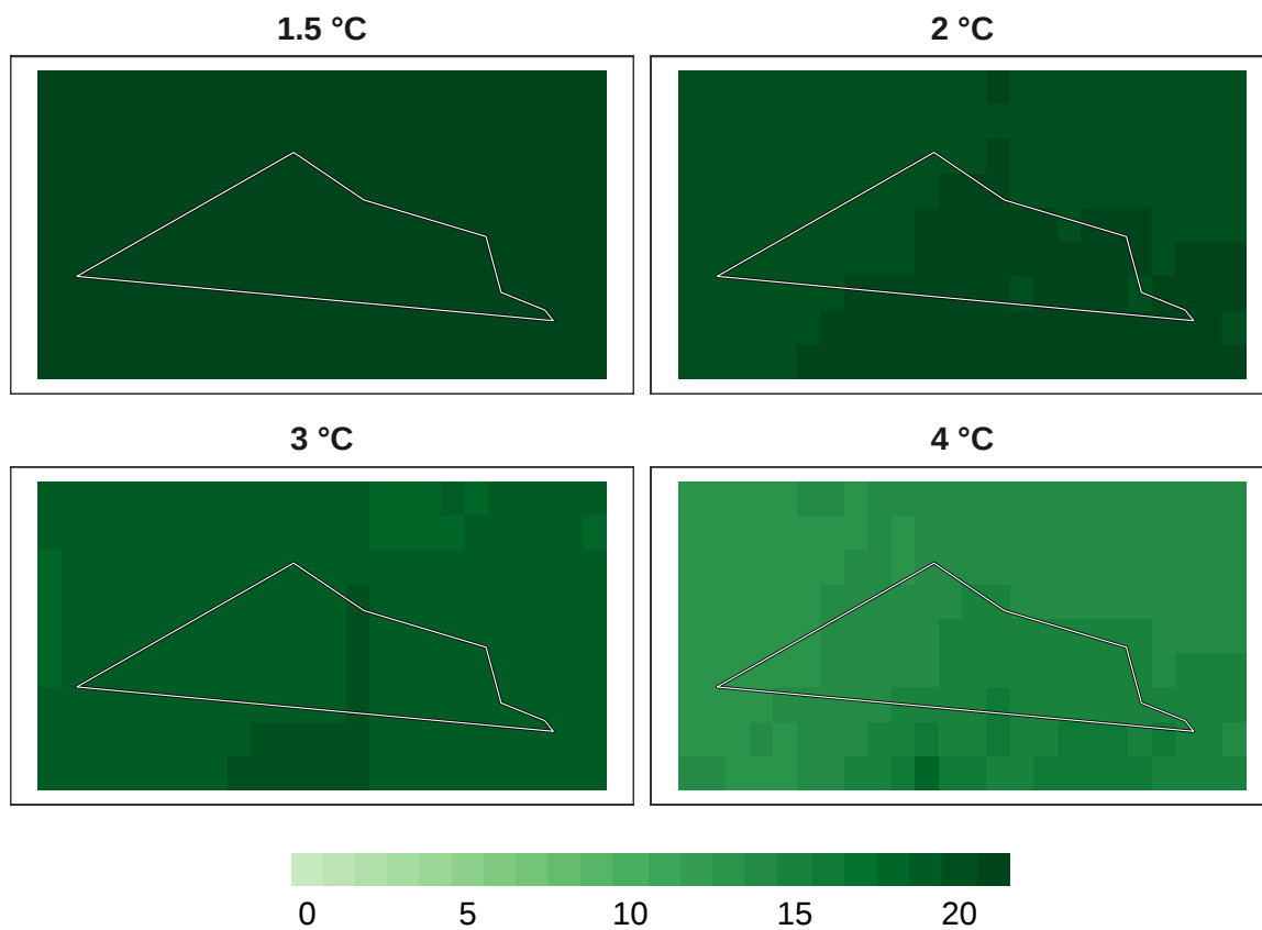
Figure 11: Number of models in agreement for reptile refugia at 1 km resolution.
