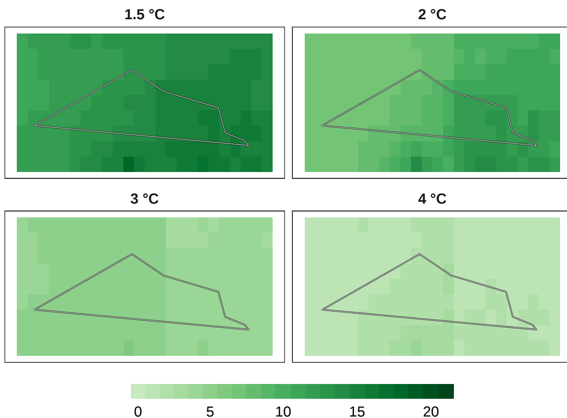
Figure 9: Number of models in agreement for bird refugia.
