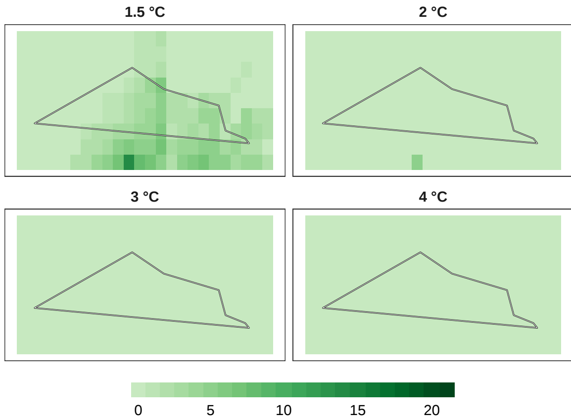
Figure 8: Number of models in agreement for plant refugia at 1 km resolution.
