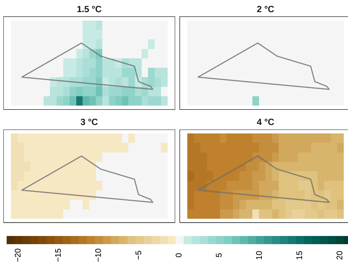
Figure 14: Adaptation effort for plants at 1 km resolution.
