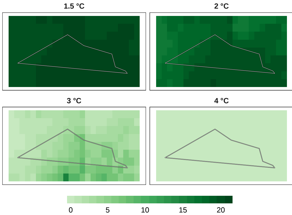
Figure 10: Number of models in agreement for mammal refugia at 1 km resolution.
