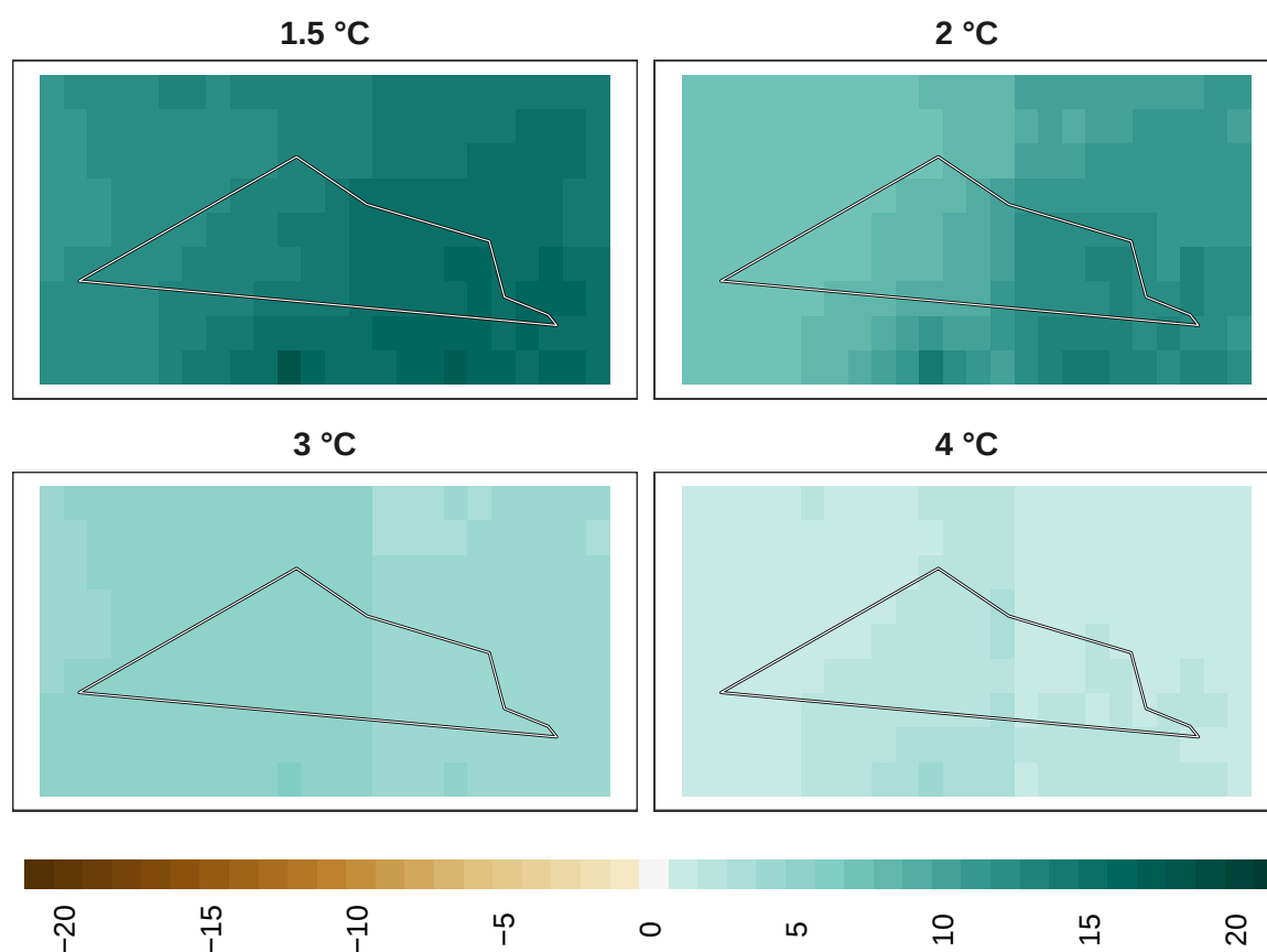
Figure 15: Adaptation effort for birds at 1 km resolution.
