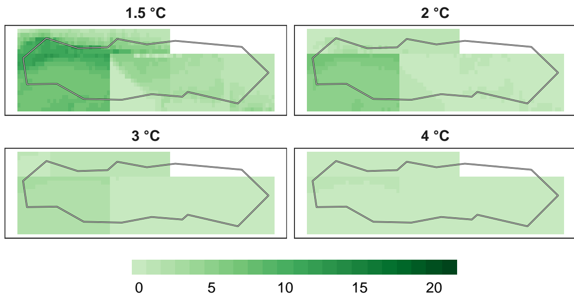
Figure 10: Number of models in agreement for amphibian refugia at 1 km resolution.
