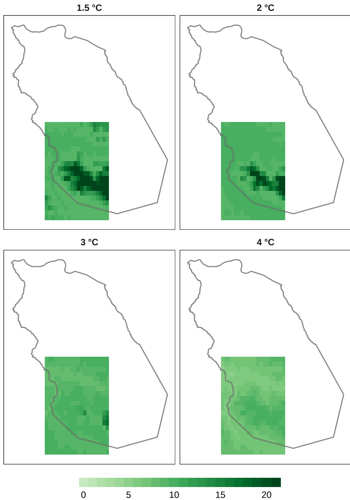
Figure 10: Number of models in agreement for amphibian refugia at 1 km resolution.
