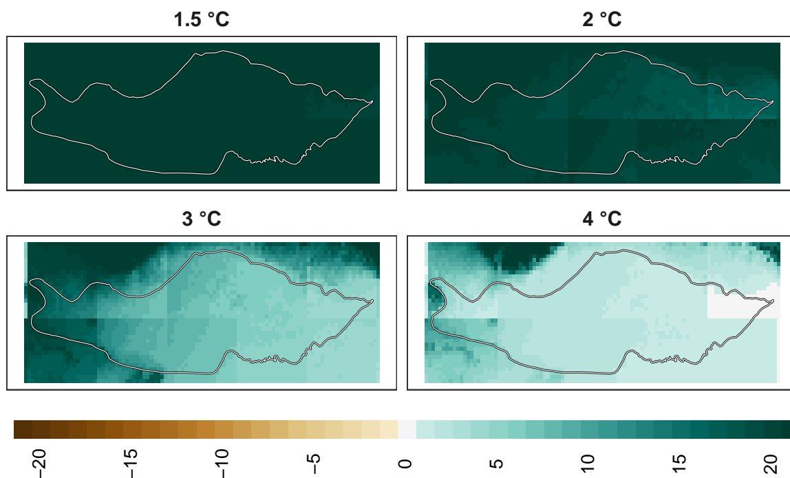
Figure 17: Adaptation effort for reptiles at 1 km resolution.
