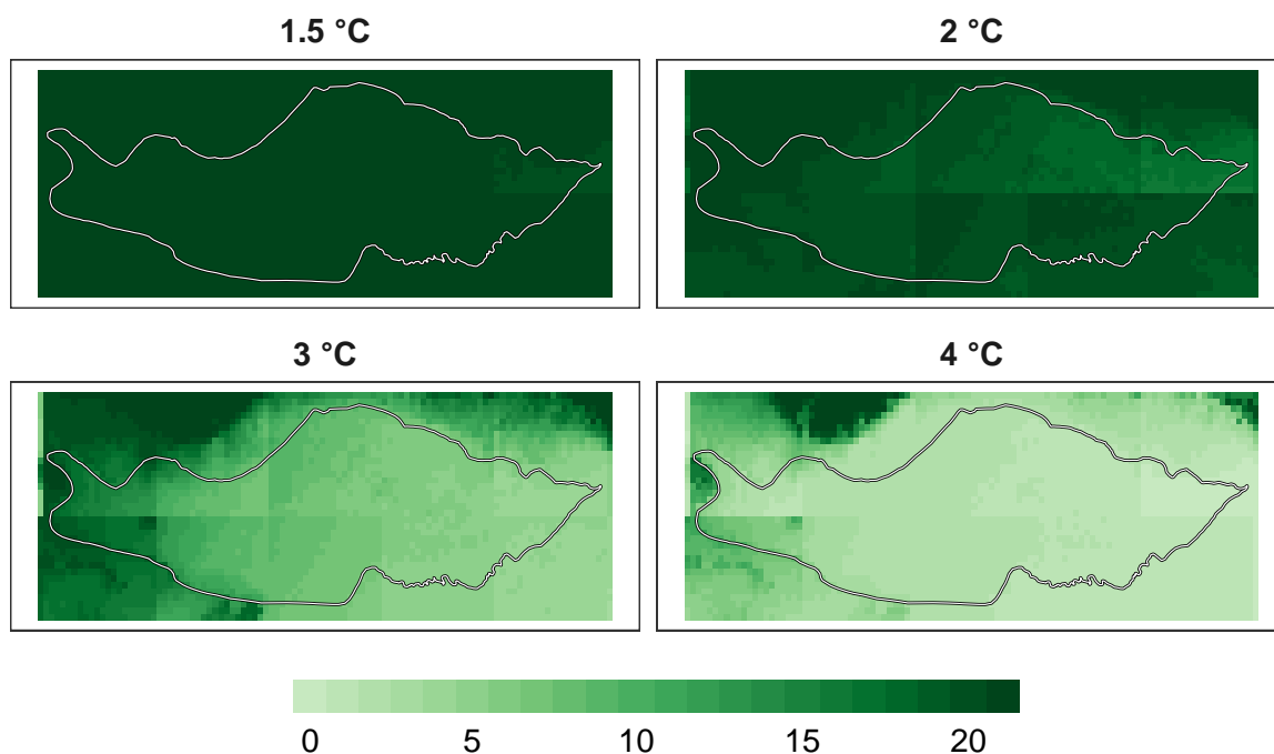
Figure 11: Number of models in agreement for reptile refugia at 1 km resolution.
