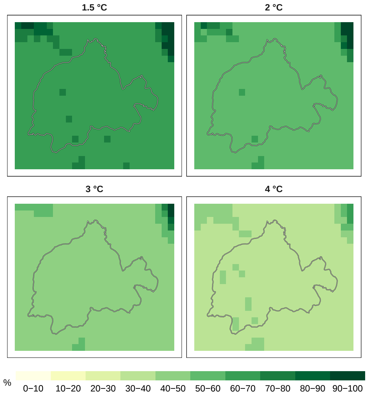
Figure 5: Percent mammals remaining at 1 km resolution.
