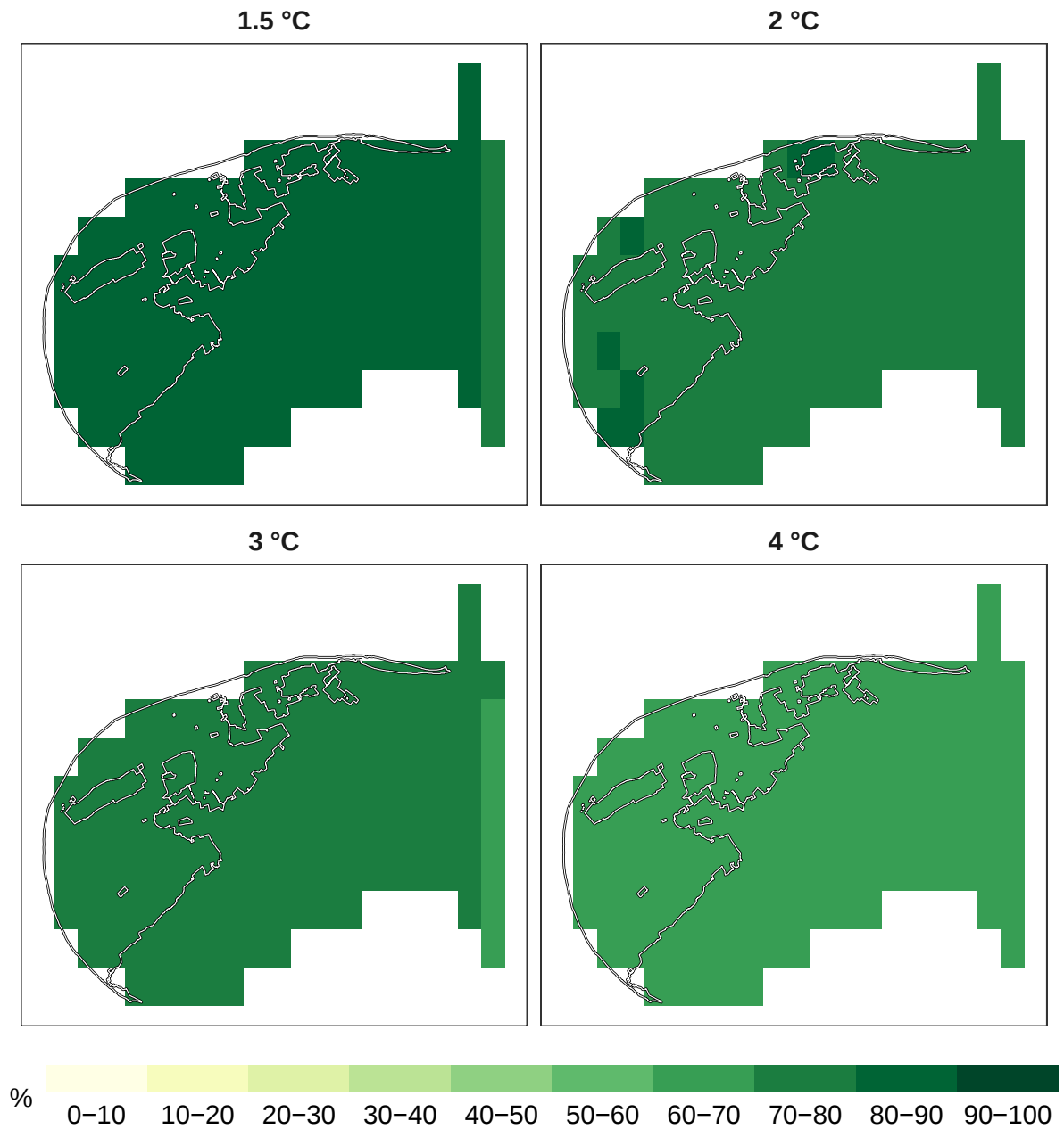
Figure 3: Percent amphibians remaining at 1 km resolution.
