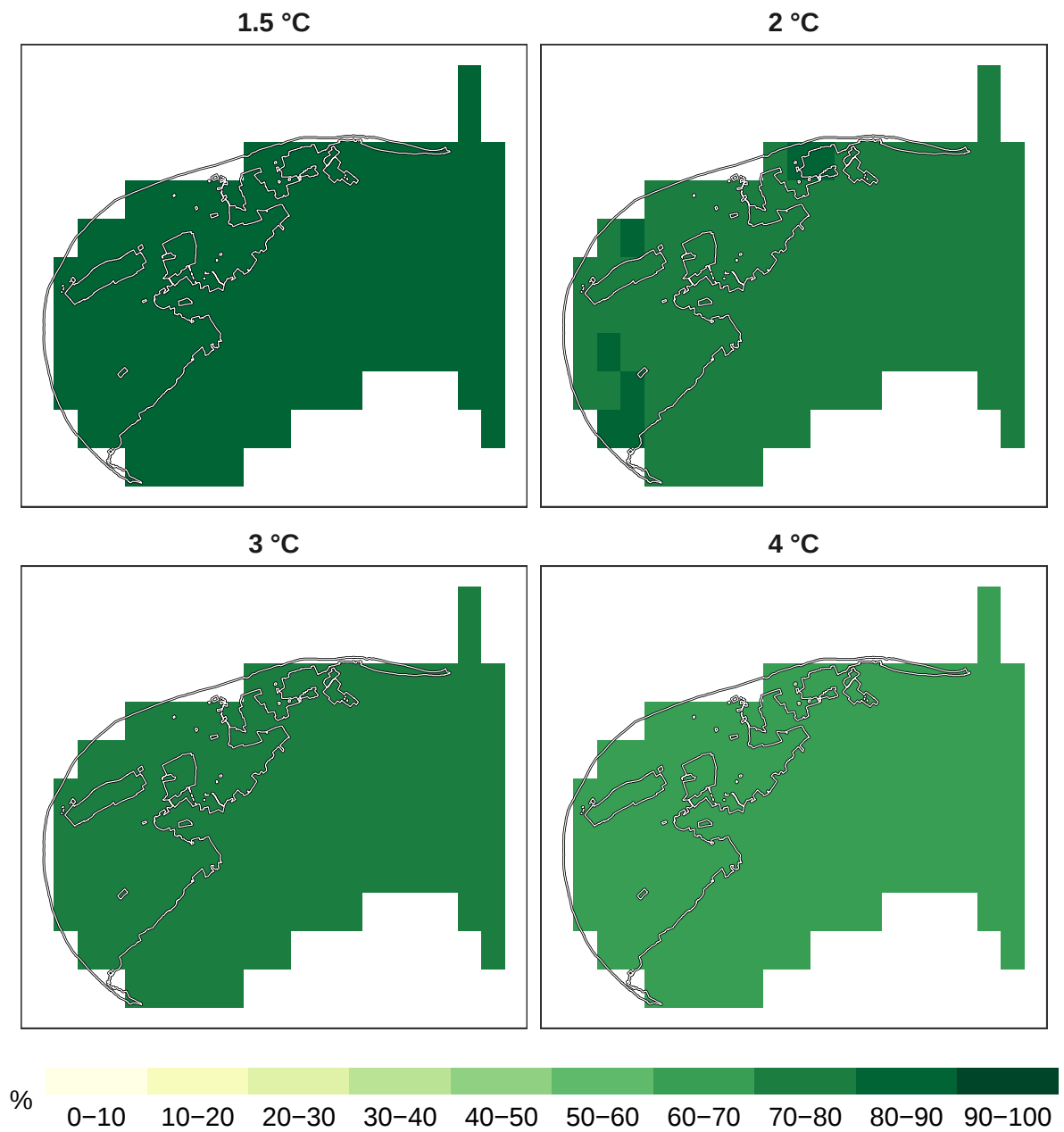
Figure 2: Percent plants remaining at 1 km resolution.
