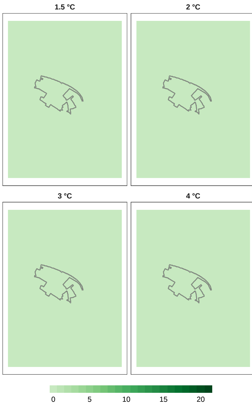
Figure 17: Number of models in agreement for pollinator refugia at 1 km resolution.
