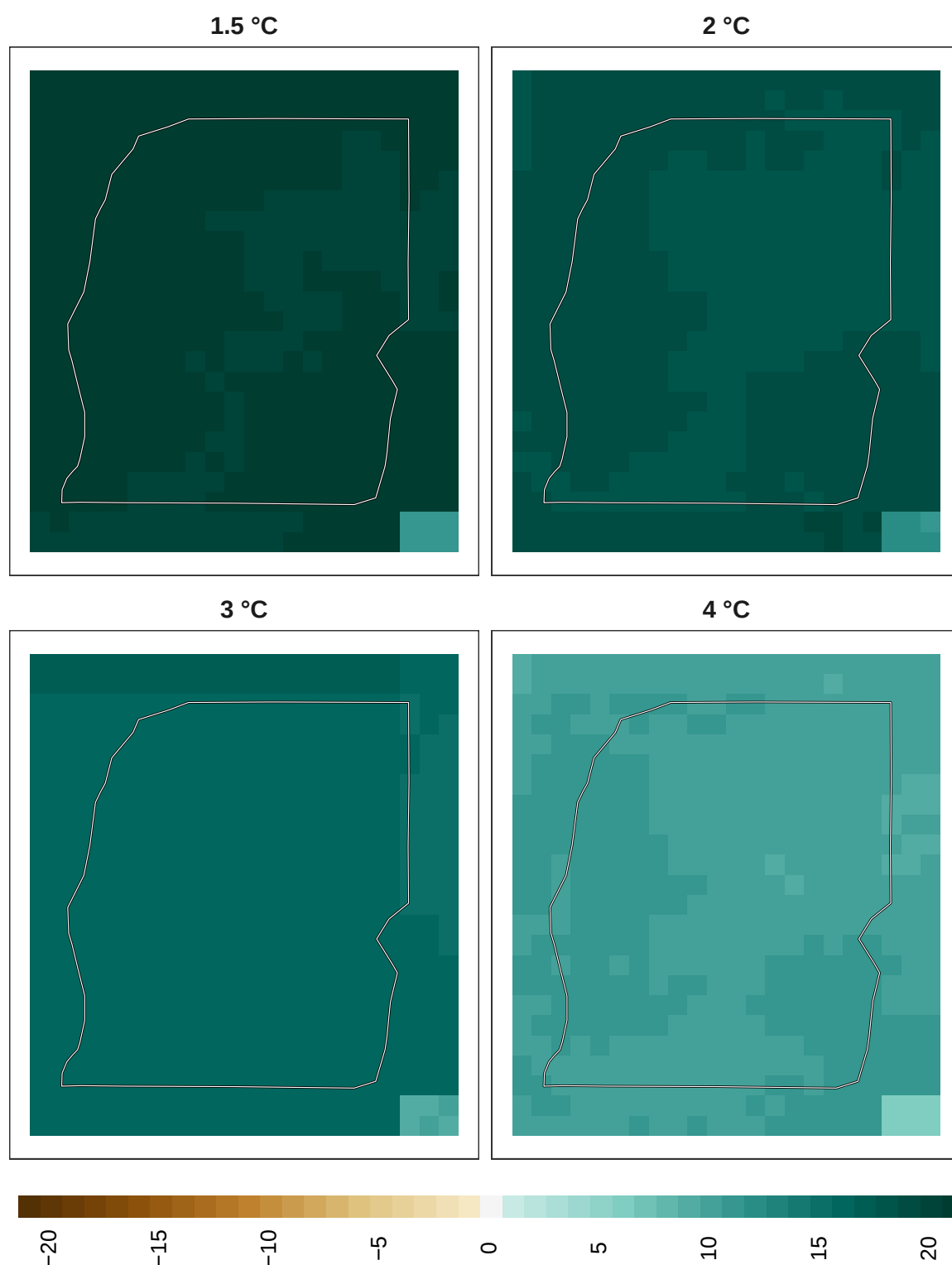
Figure 19: Adaptation effort for insects at 1 km resolution.
