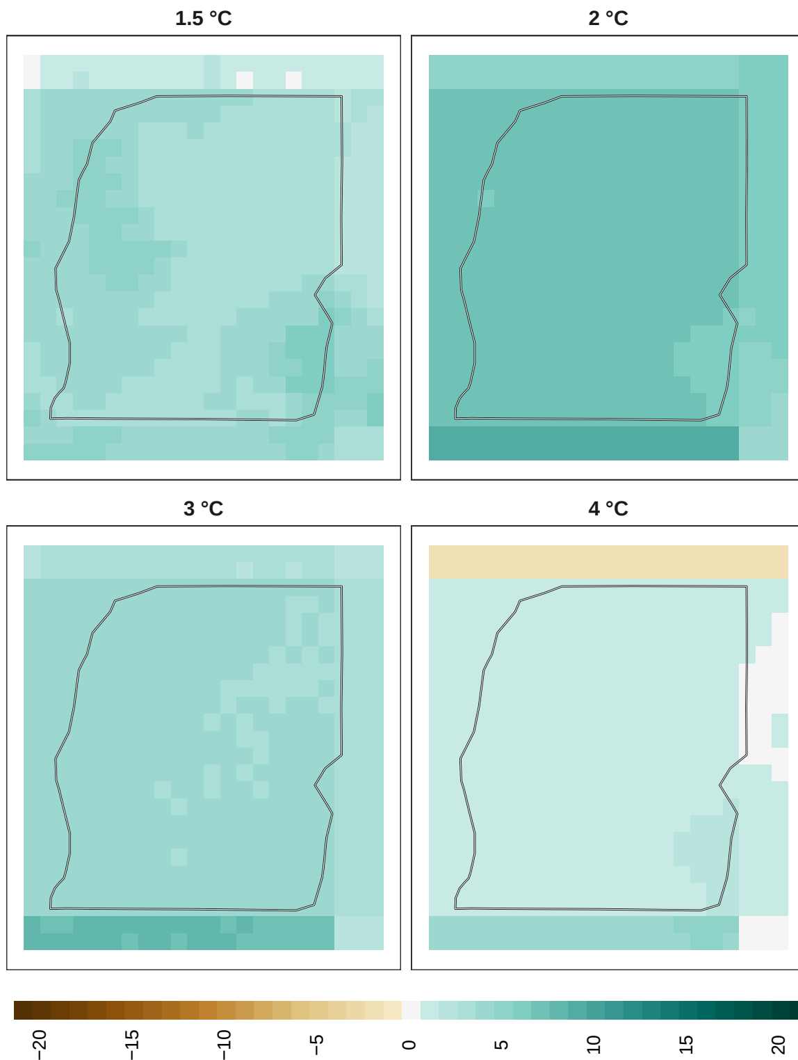
Figure 18: Adaptation effort for reptiles at 1 km resolution.
