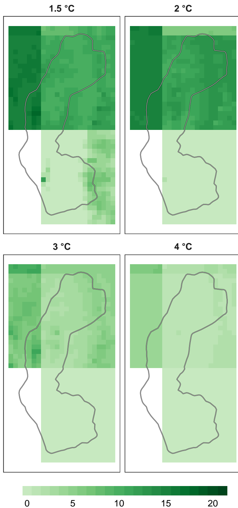
Figure 12: Number of models in agreement for reptile refugia at 1 km resolution.
