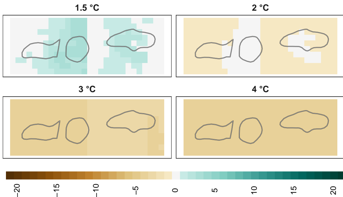
Figure 14: Adaptation effort for birds at 1 km resolution.
