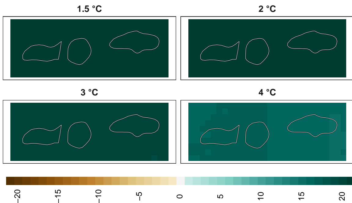
Figure 13: Adaptation effort for plants at 1 km resolution.
