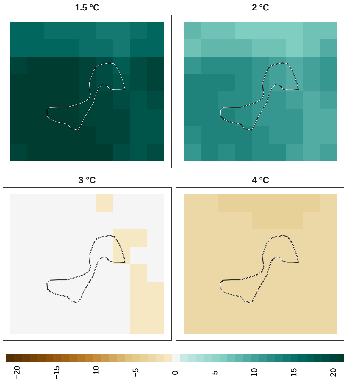
Figure 19: Adaptation effort for insects at 1 km resolution.
