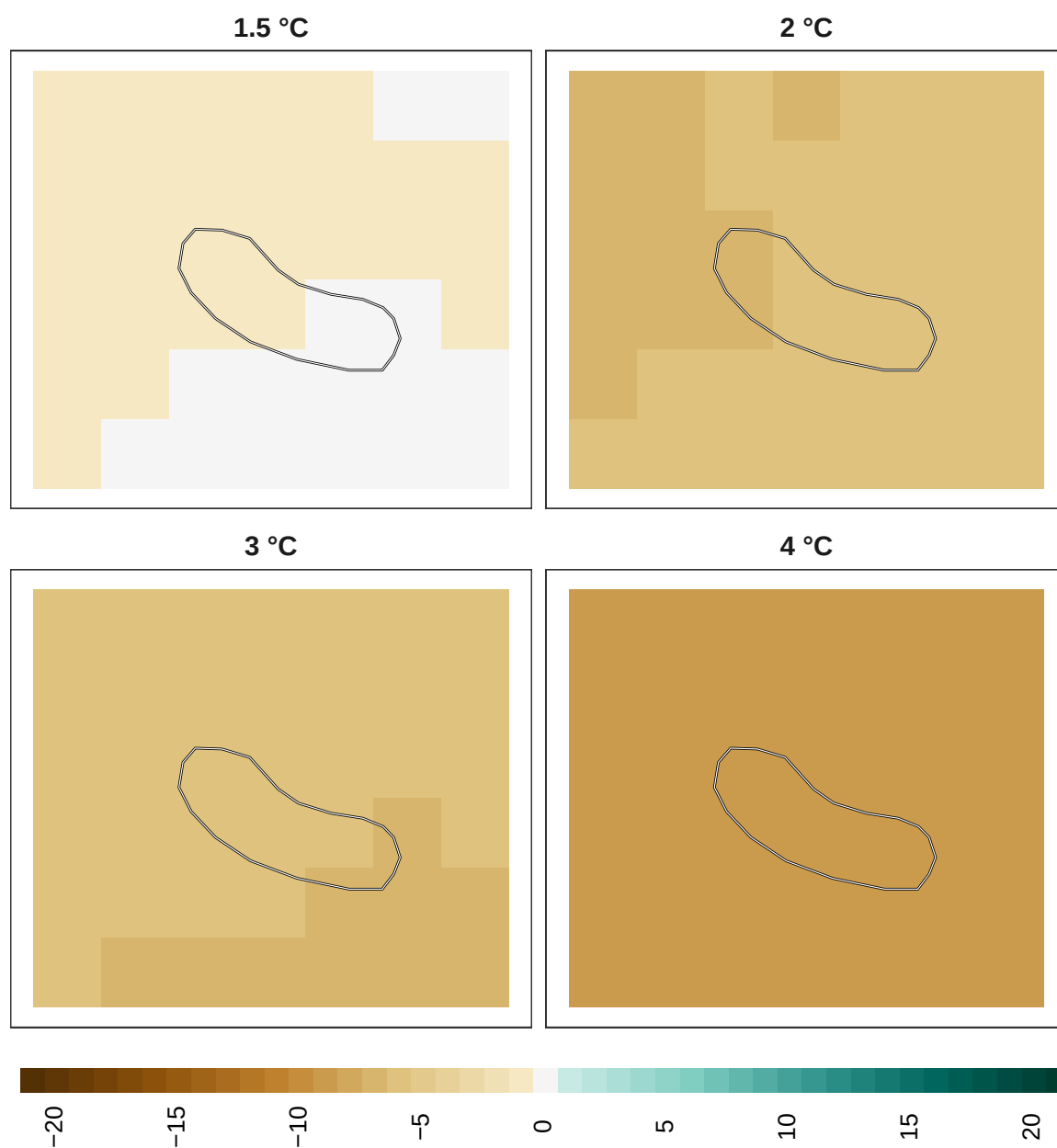
Figure 14: Adaptation effort for birds at 1 km resolution.
