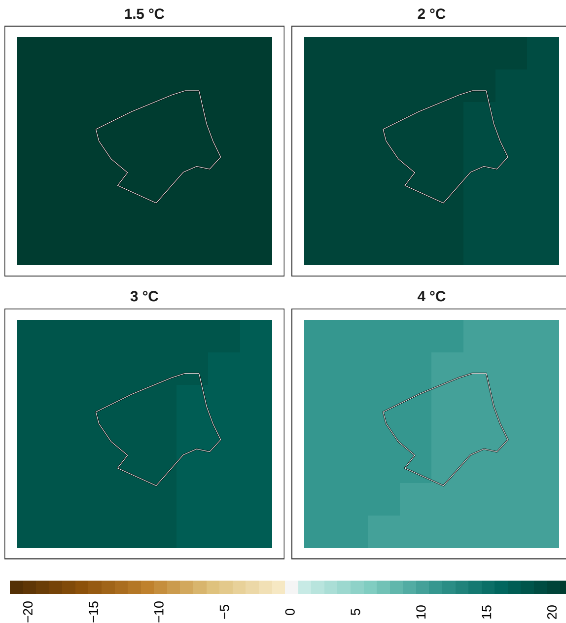
Figure 16: Adaptation effort for insects at 1 km resolution.
