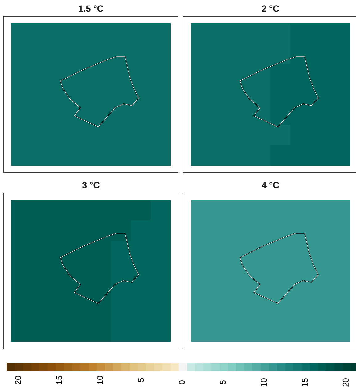
Figure 15: Adaptation effort for mammals at 1 km resolution.
