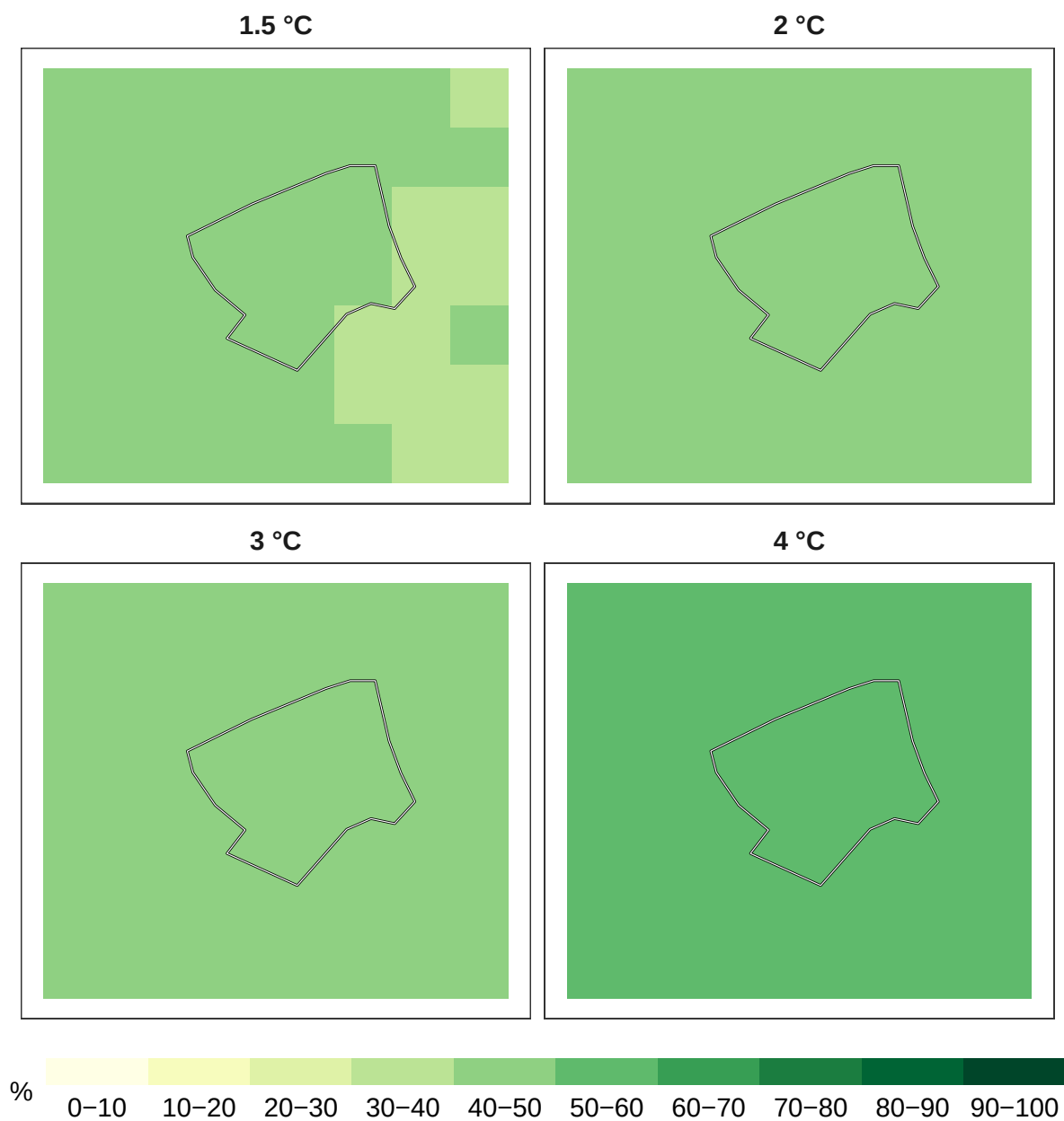
Figure 6: Percent timber species remaining at 1 km resolution.
