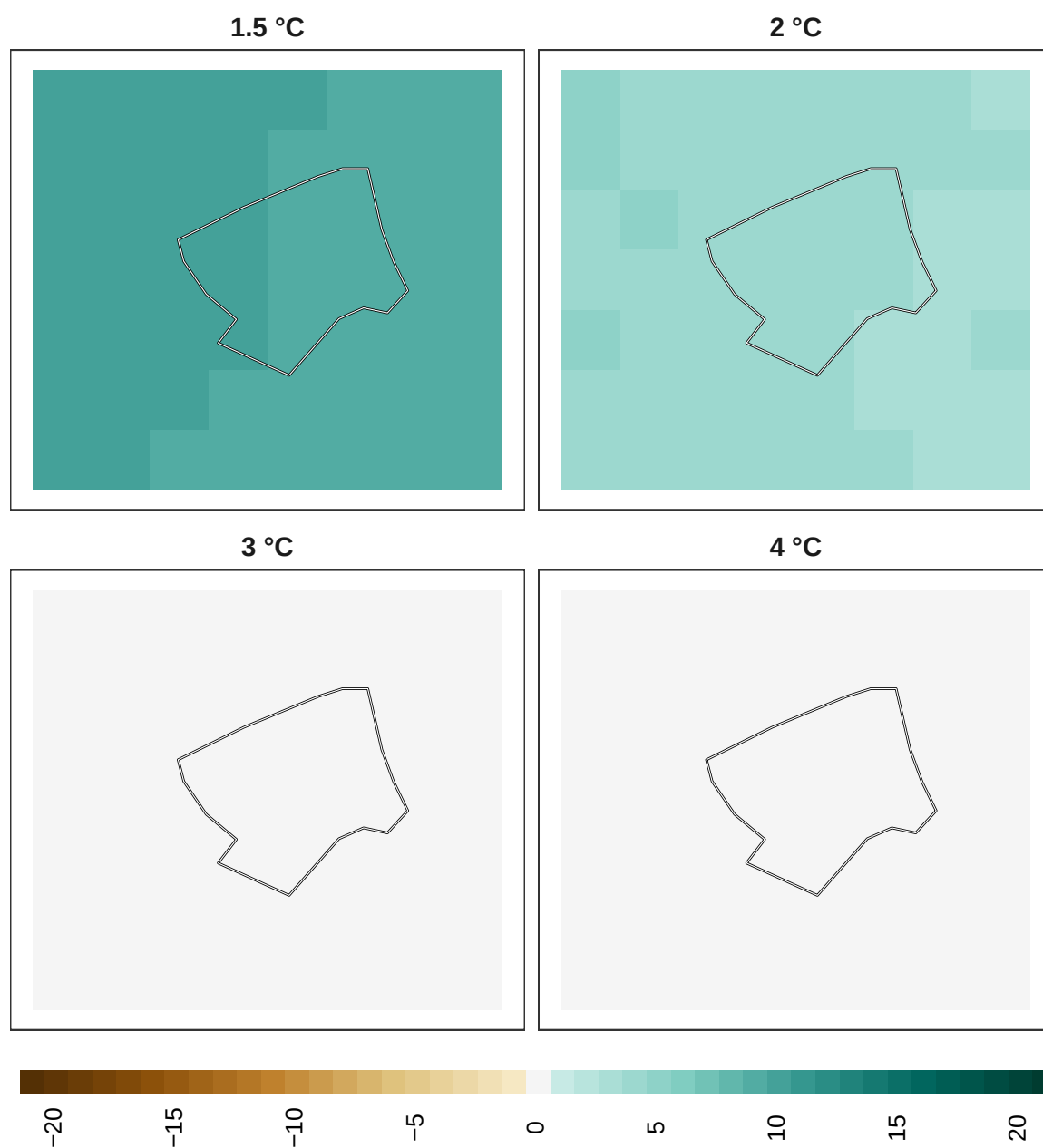
Figure 13: Adaptation effort for plants at 1 km resolution.
