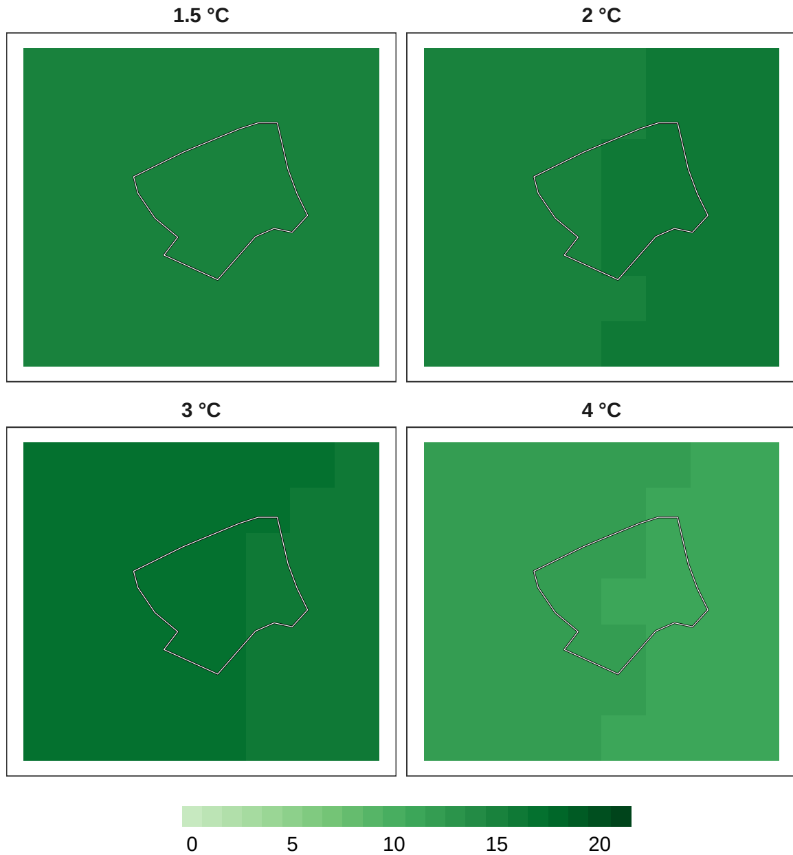
Figure 10: Number of models in agreement for mammal refugia at 1 km resolution.
