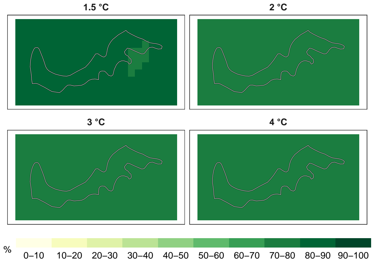
Figure 4: Percent mammals remaining at 1 km resolution.
