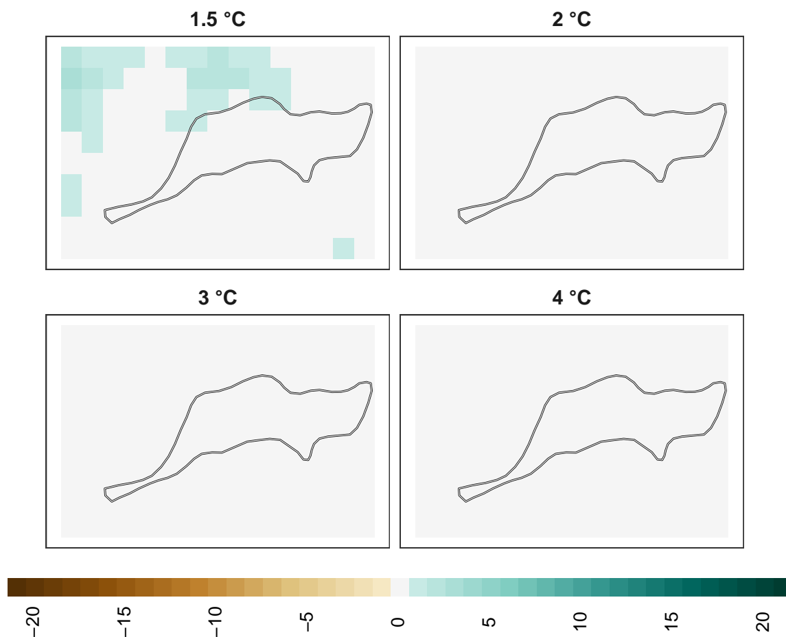
Figure 18: Adaptation effort for reptiles at 1 km resolution.
