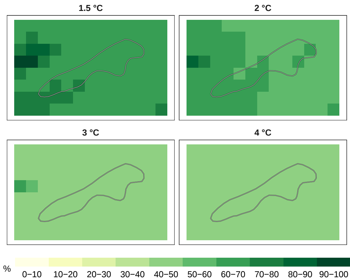
Figure 6: Percent timber species remaining at 1 km resolution.
