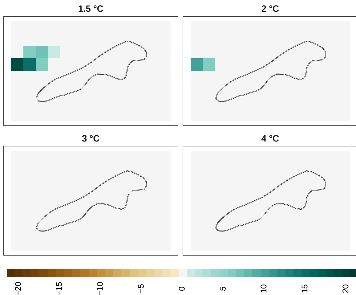
Figure 12: Adaptation effort for overall biodiversity at 1 km resolution.
