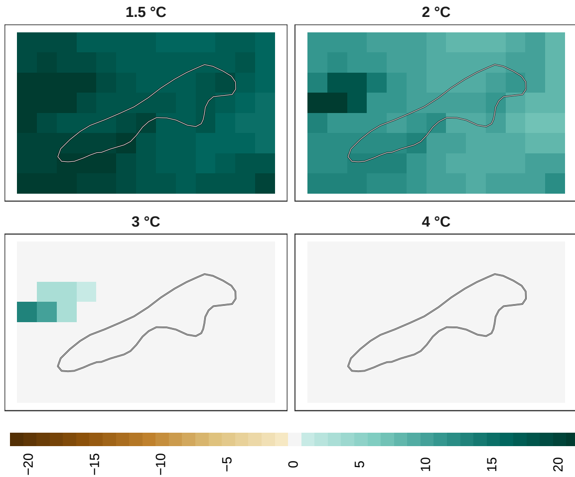
Figure 13: Adaptation effort for plants at 1 km resolution.
