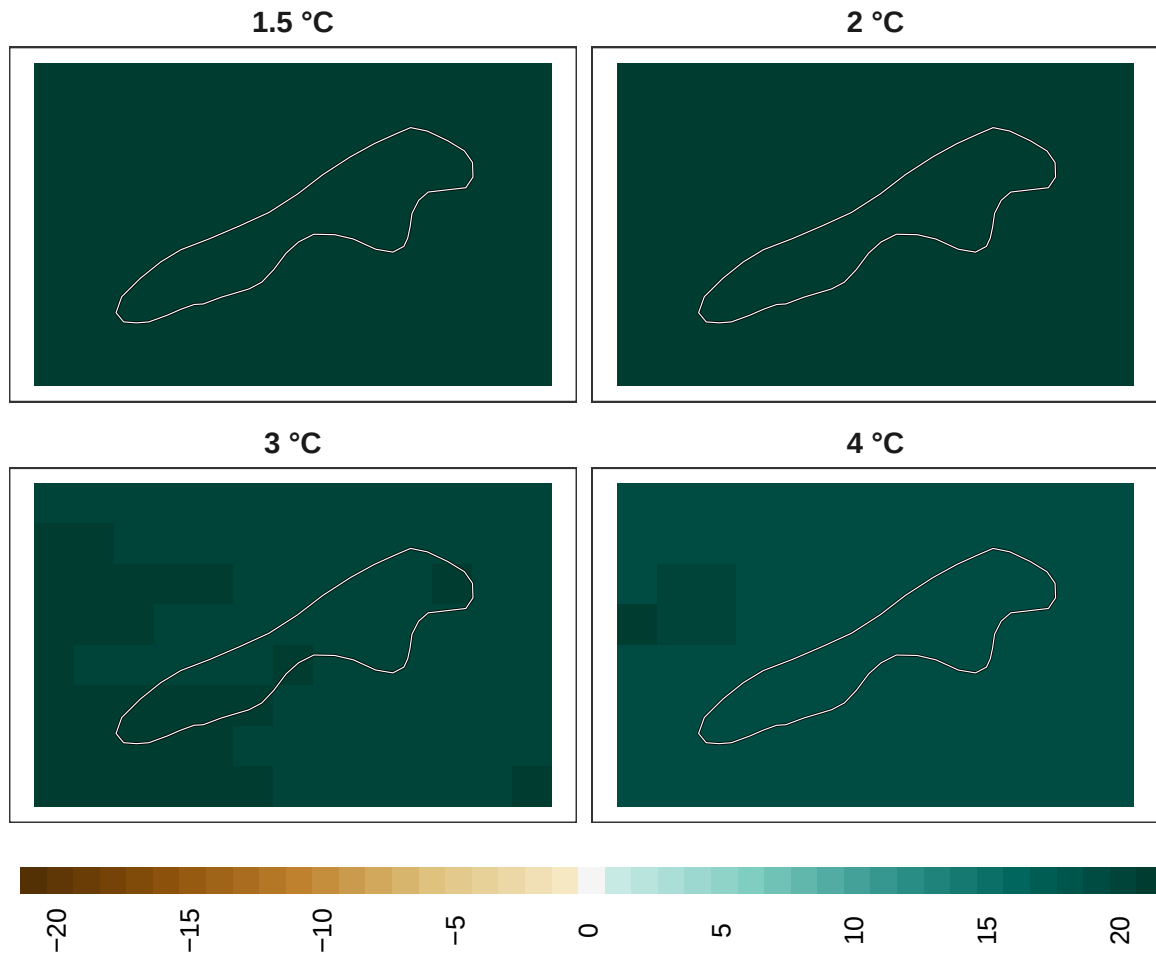
Figure 15: Adaptation effort for mammals at 1 km resolution.
