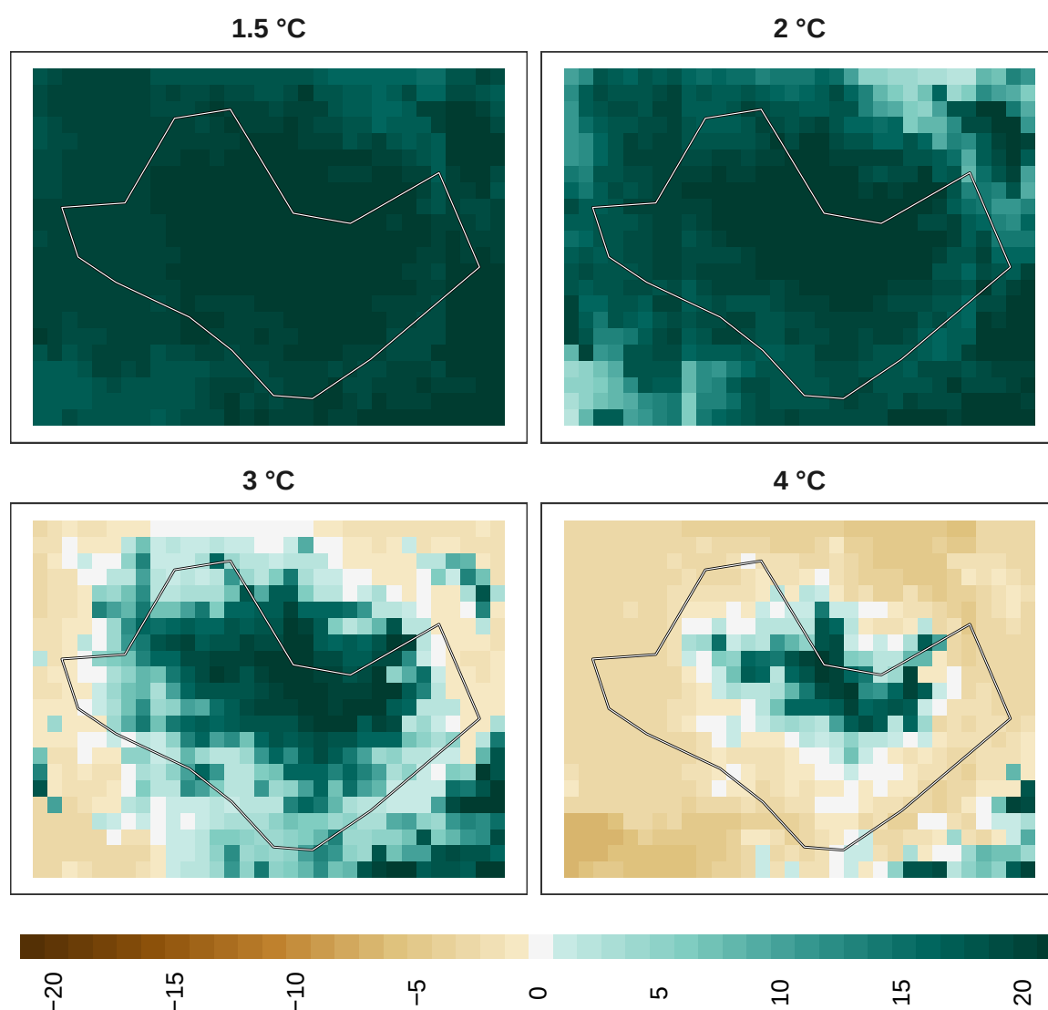
Figure 17: Adaptation effort for birds at 1 km resolution.
