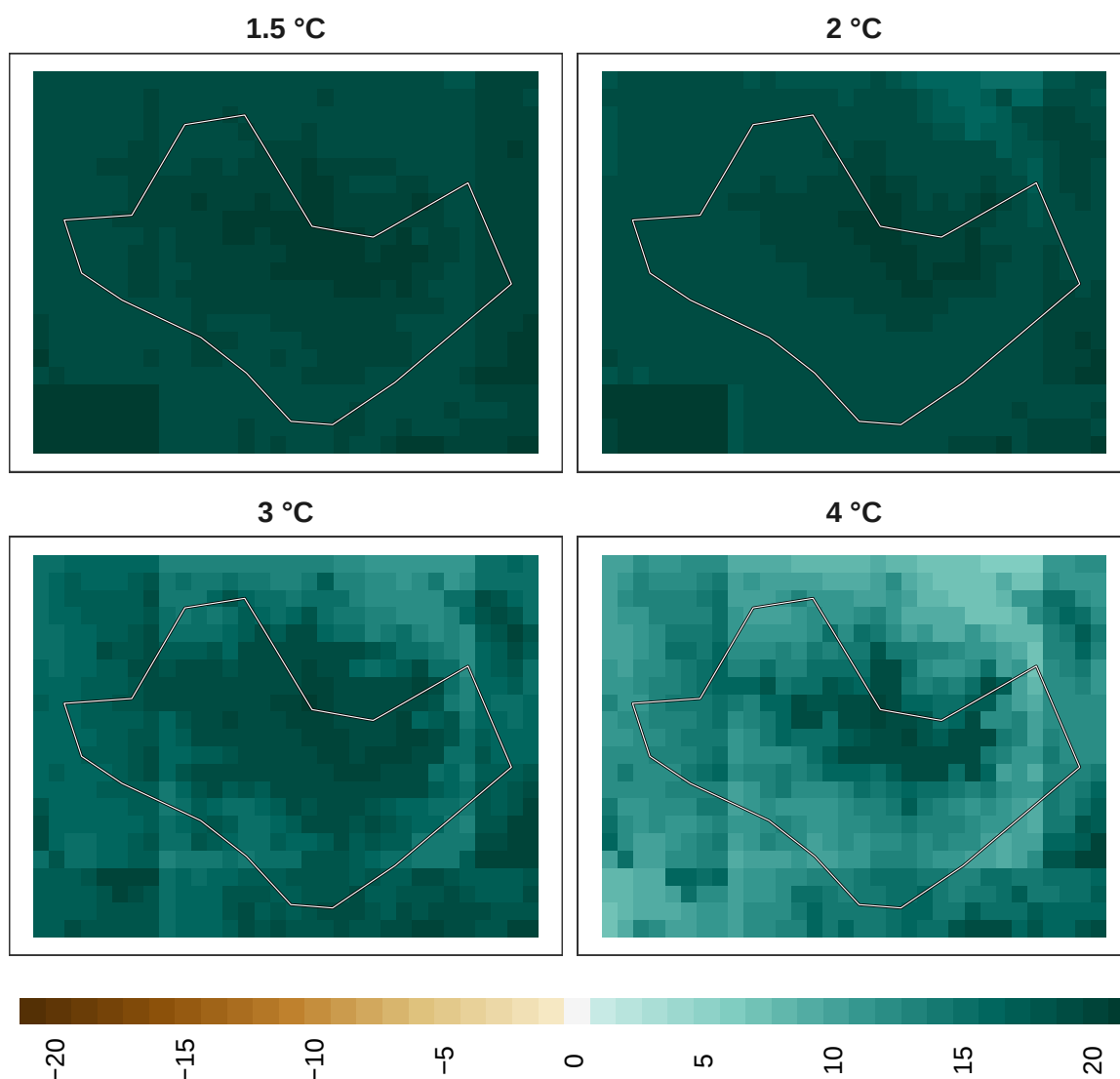
Figure 18: Adaptation effort for mammals at 1 km resolution.
