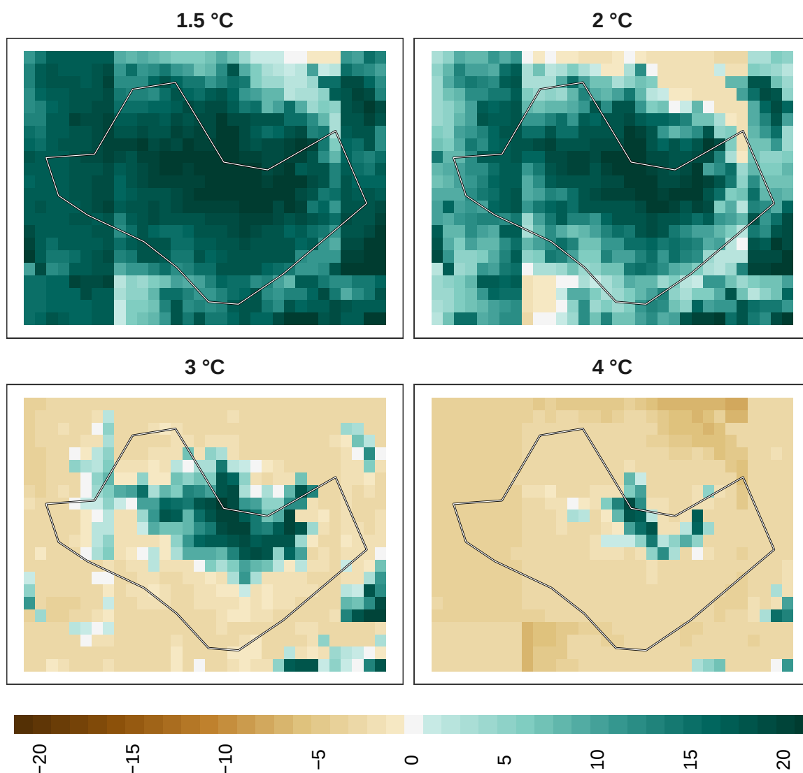
Figure 16: Adaptation effort for plants at 1 km resolution.
