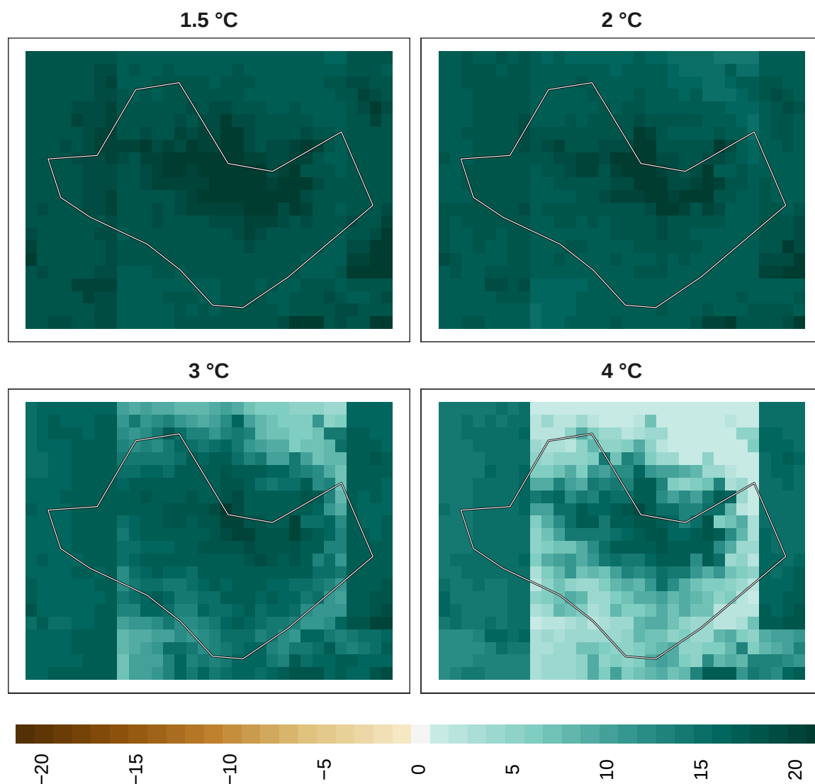
Figure 19: Adaptation effort for reptiles at 1 km resolution.
