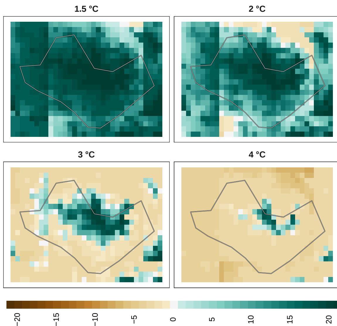
Figure 15: Adaptation effort for overall biodiversity at 1 km resolution.
