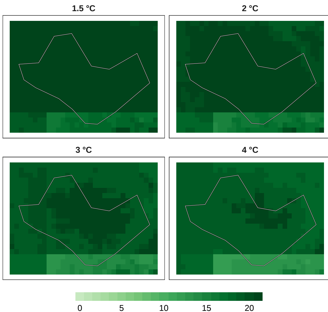
Figure 14: Number of models in agreement for pollinator refugia at 1 km resolution.
