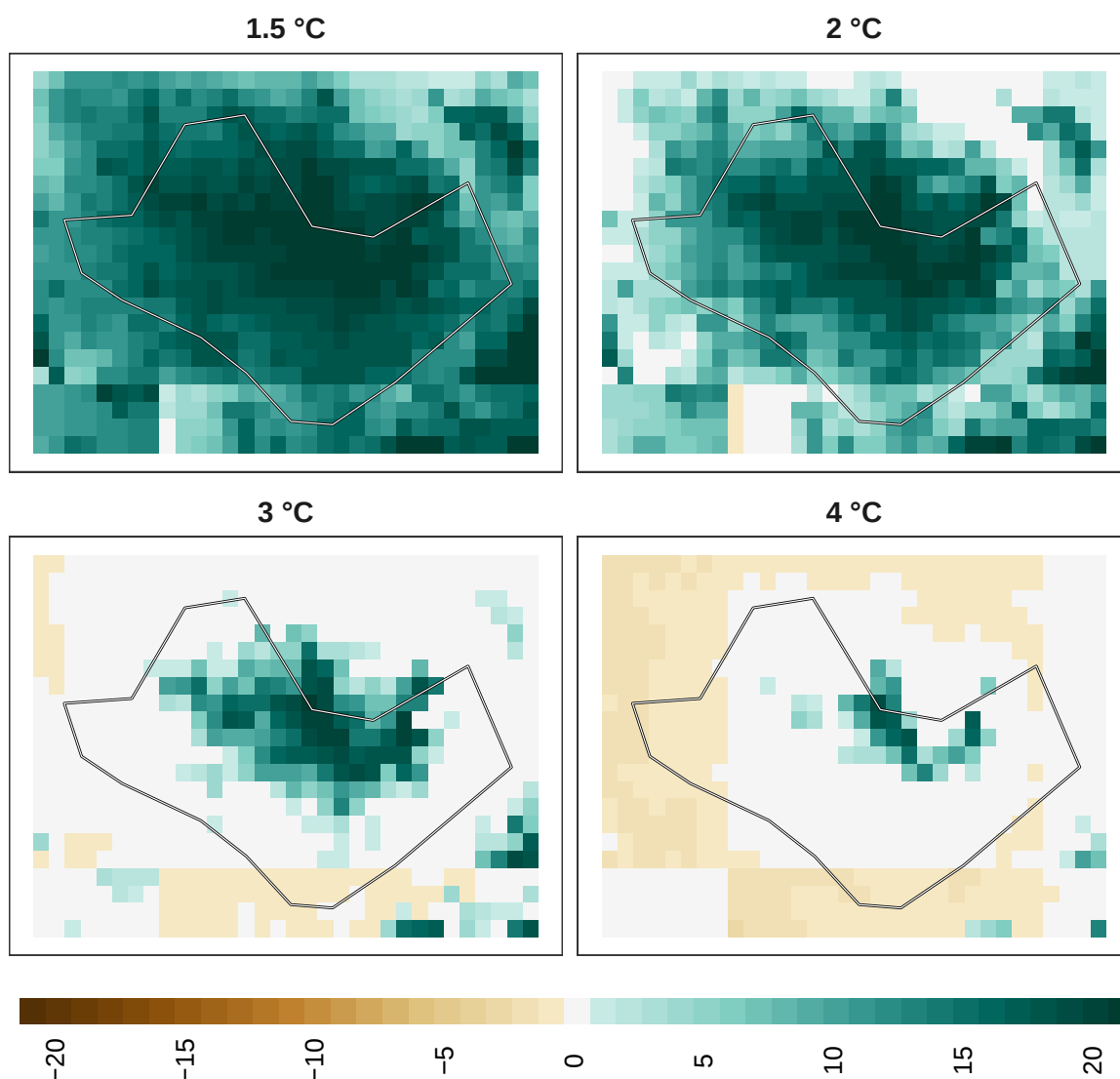
Figure 20: Adaptation effort for insects at 1 km resolution.
