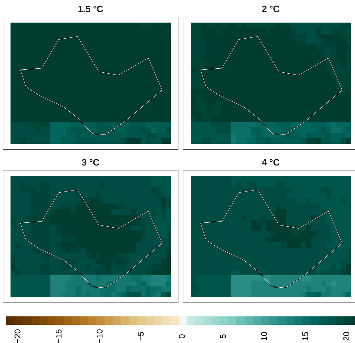
Figure 21: Adaptation effort for pollinators at 1 km resolution.
