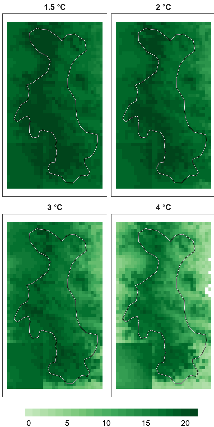
Figure 12: Number of models in agreement for reptile refugia at 1 km resolution.
