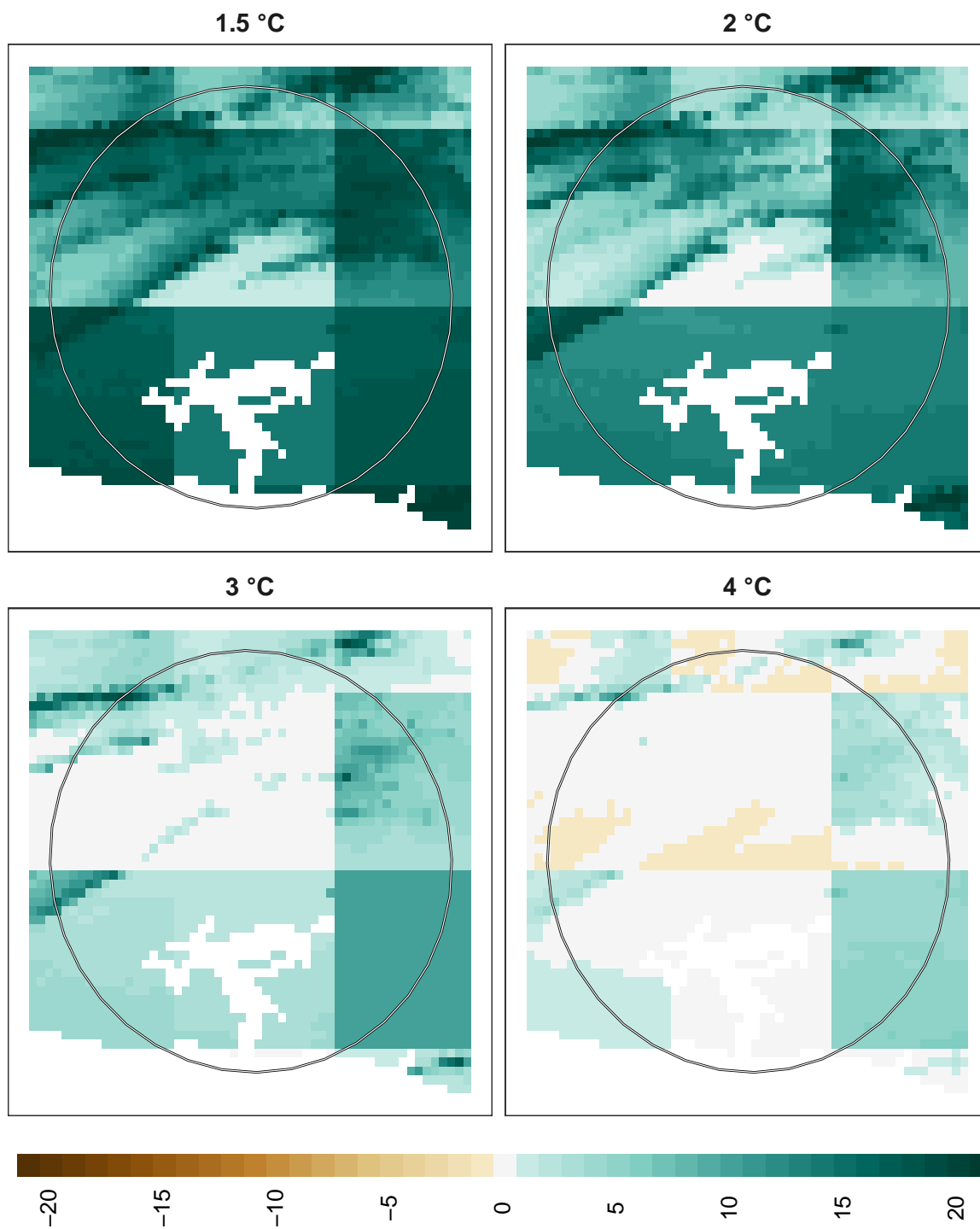
Figure 19: Adaptation effort for reptiles at 1 km resolution.
