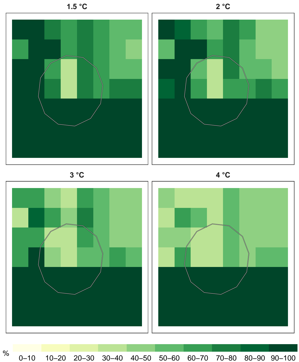
Figure 6: Percent pollinators remaining at 1 km resolution.
