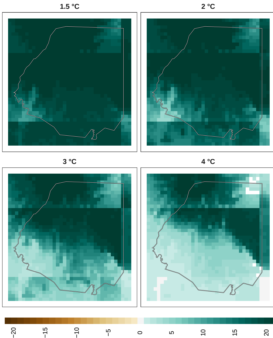
Figure 21: Adaptation effort for reptiles at 1 km resolution.
