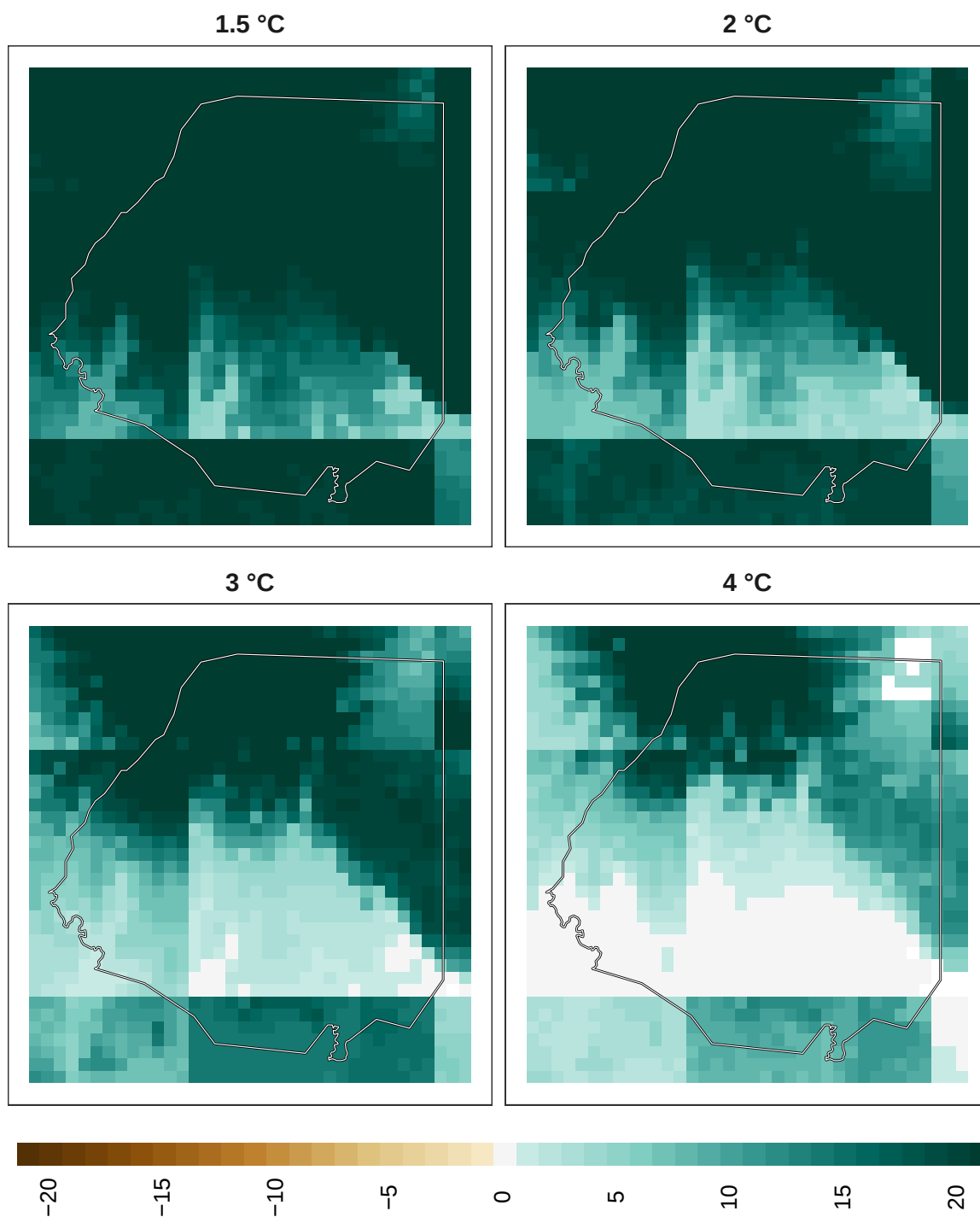
Figure 22: Adaptation effort for insects at 1 km resolution.
