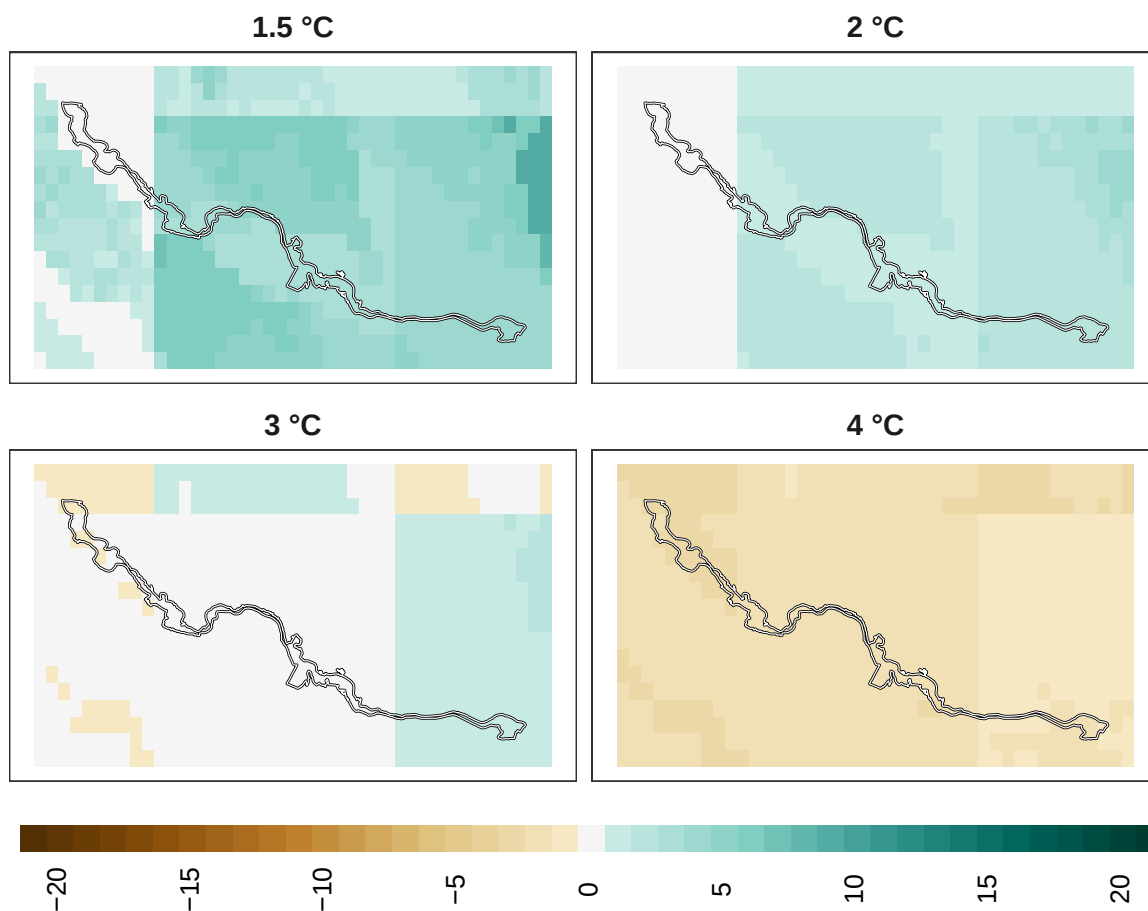
Figure 25: Adaptation effort for pollinators at 1 km resolution.
