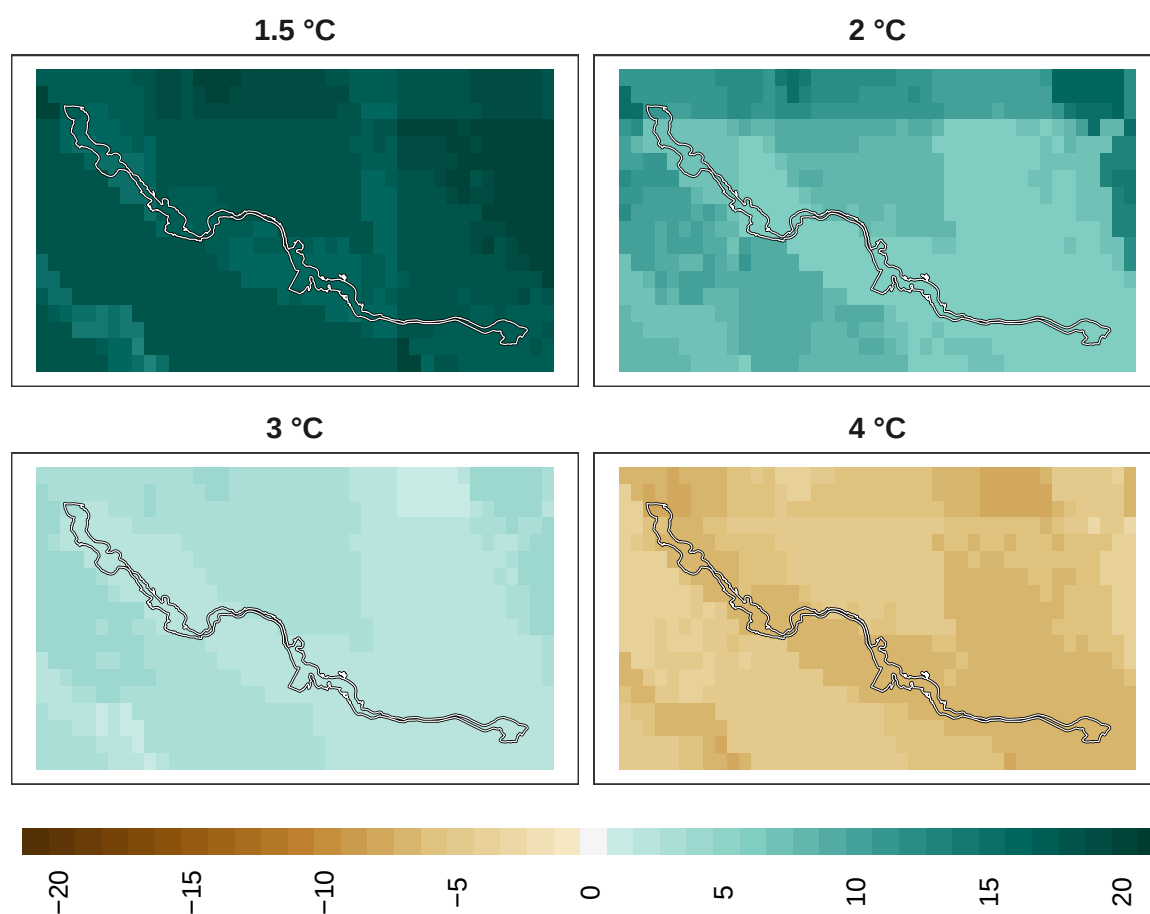
Figure 21: Adaptation effort for birds at 1 km resolution.
