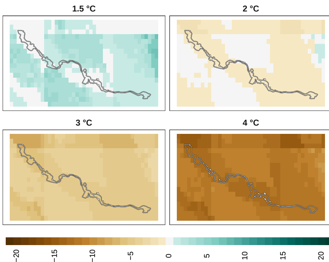
Figure 24: Adaptation effort for insects at 1 km resolution.
