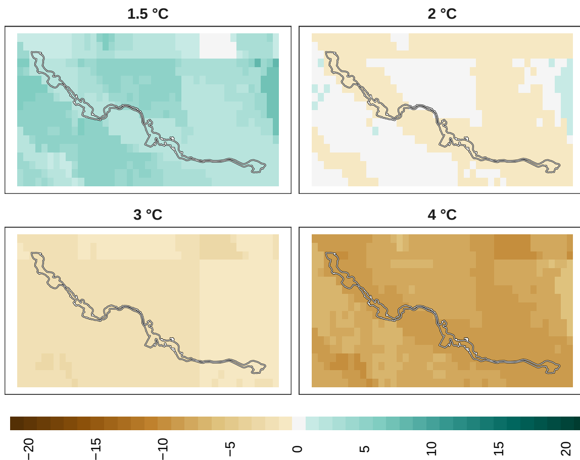
Figure 19: Adaptation effort for plants at 1 km resolution.
