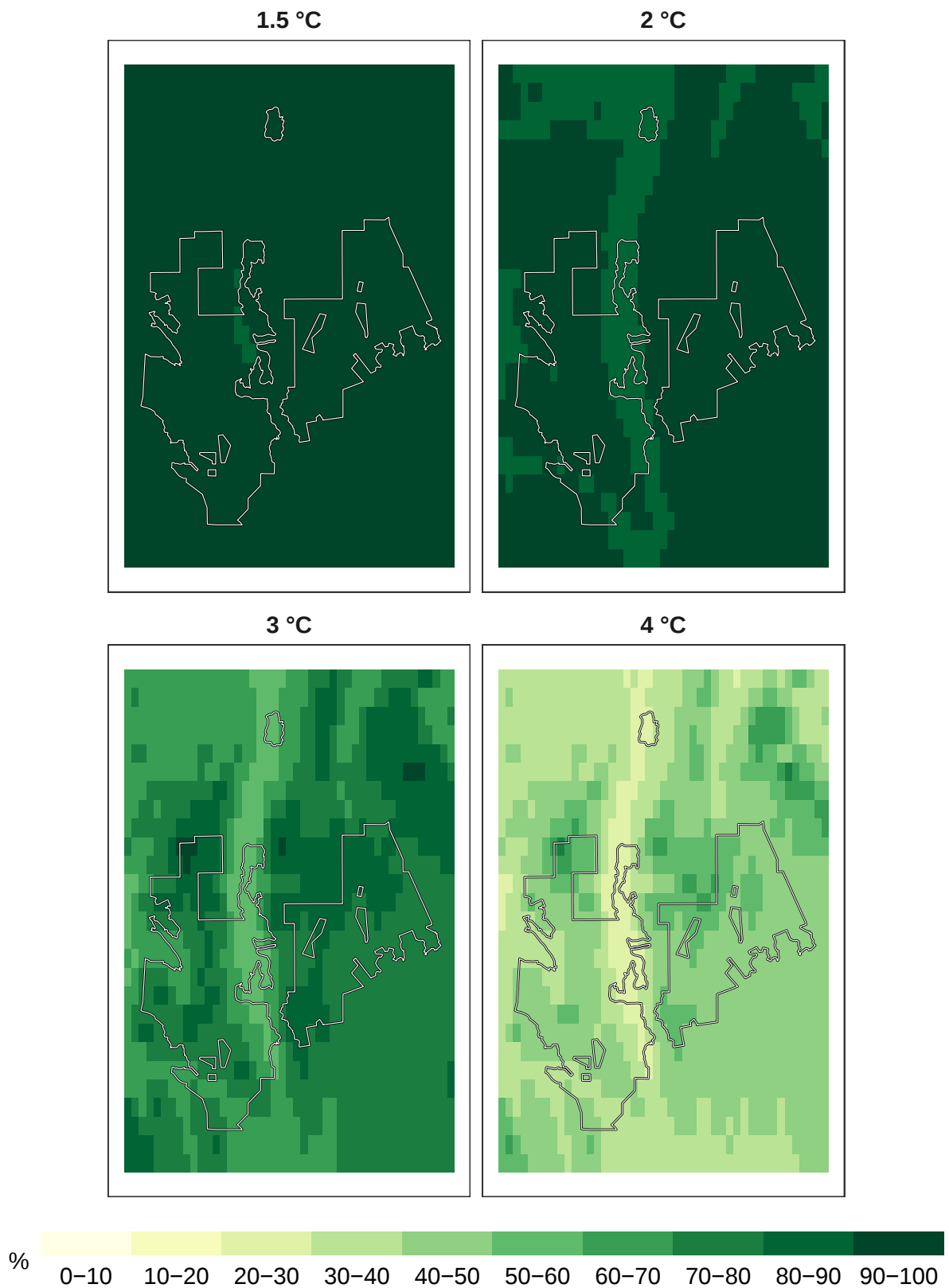
Figure 5: Percent insects remaining at 1 km resolution.
