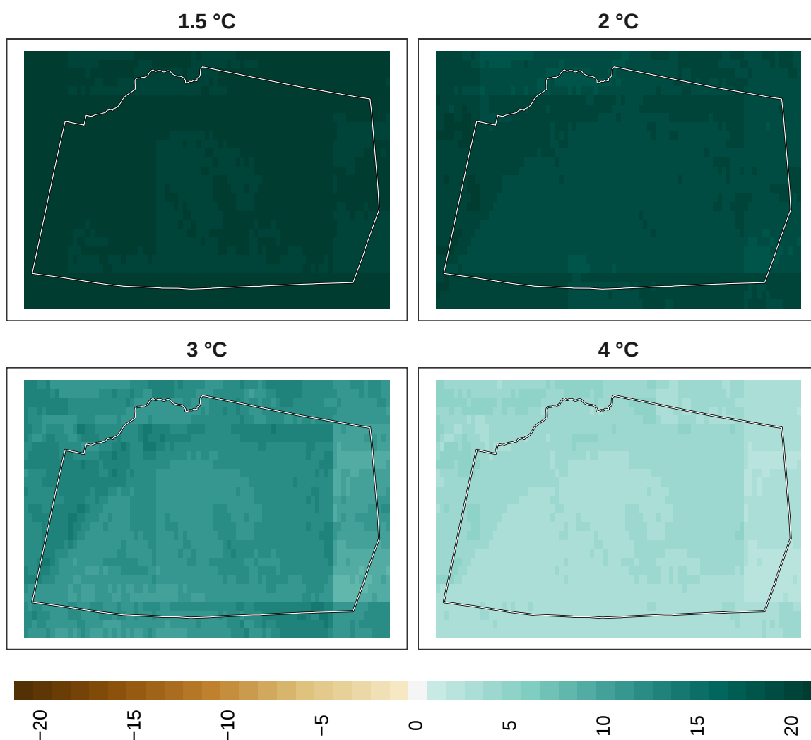
Figure 16: Adaptation effort for mammals at 1 km resolution.
