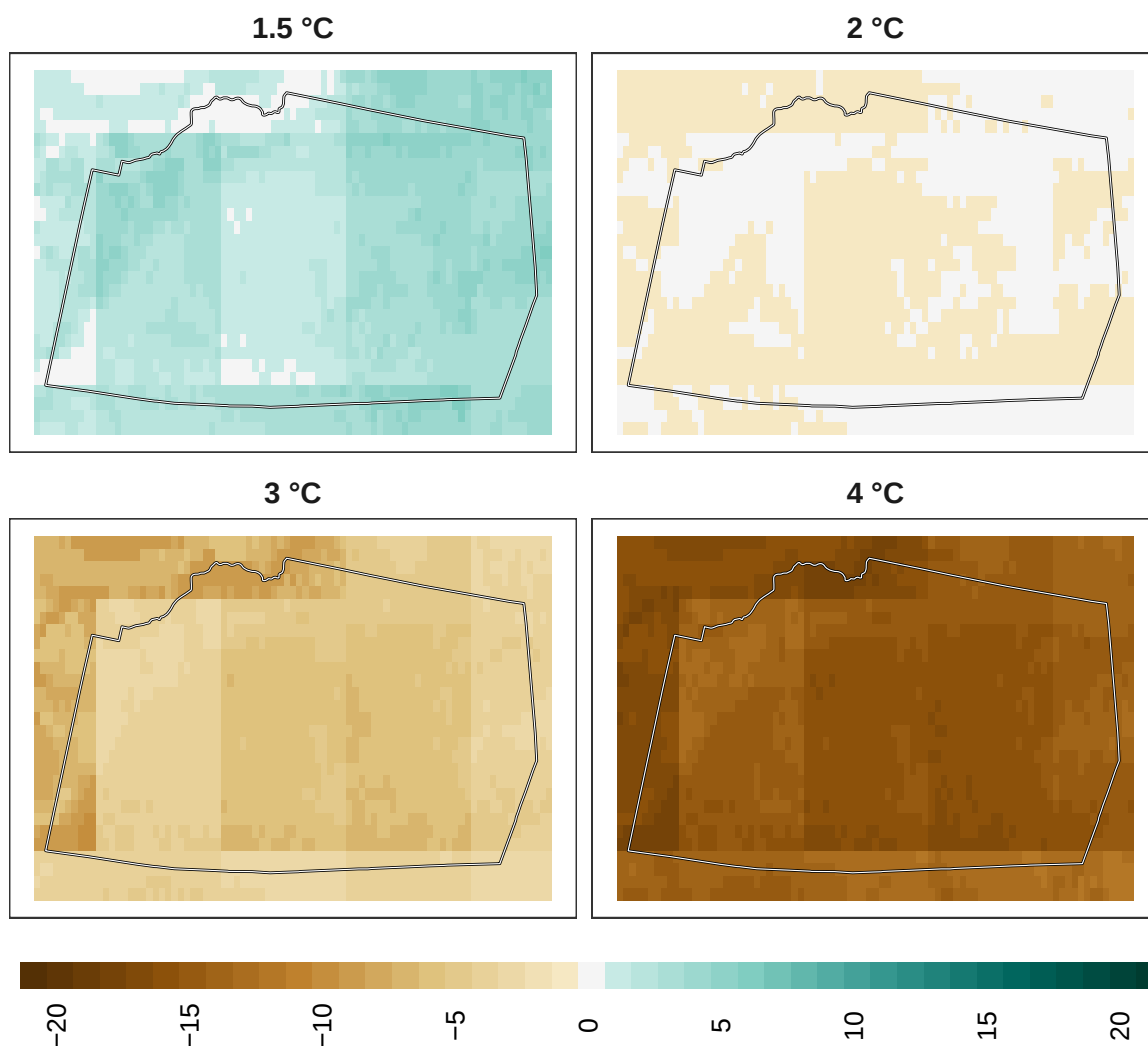
Figure 17: Adaptation effort for insects at 1 km resolution.
