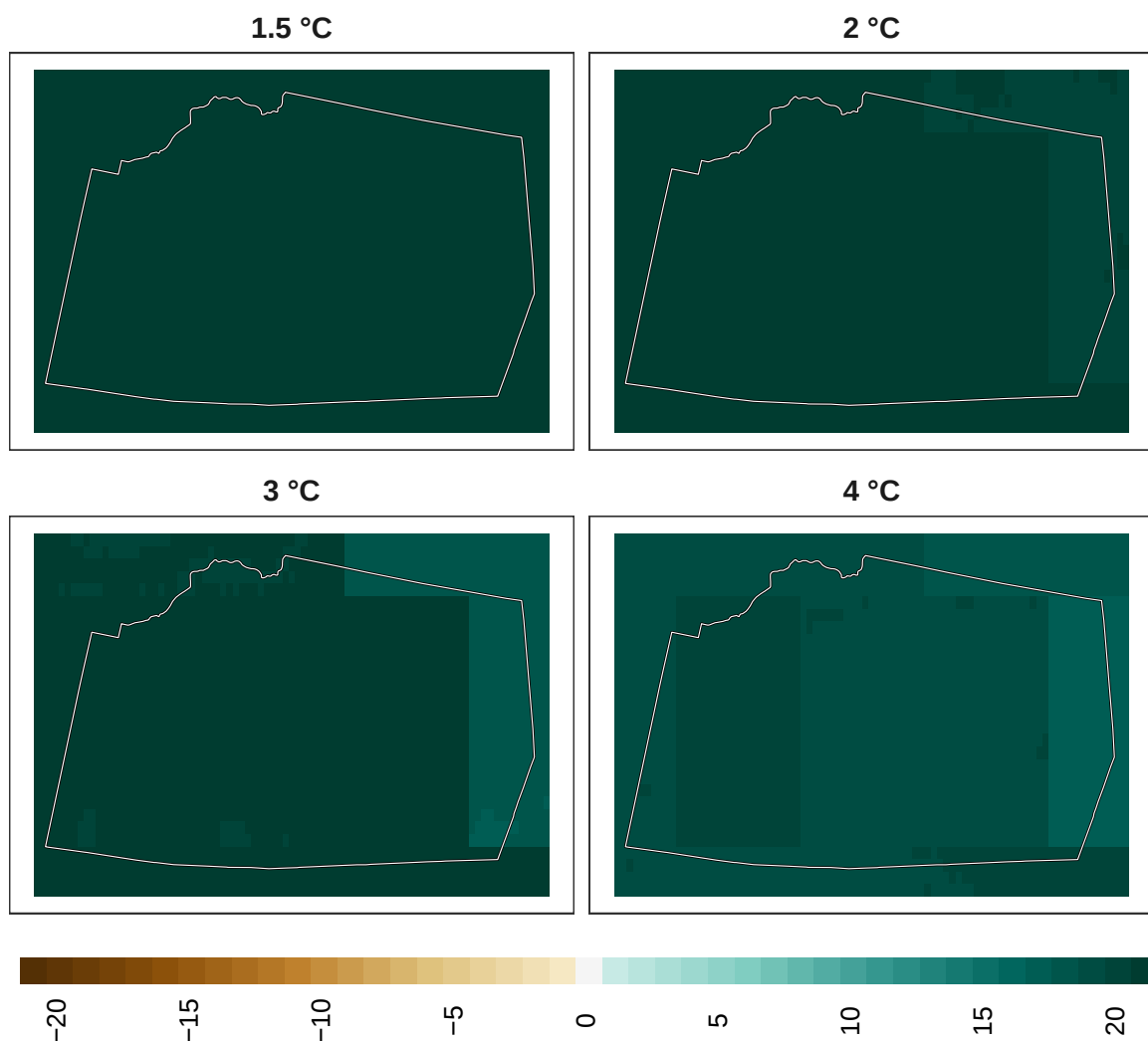
Figure 15: Adaptation effort for birds at 1 km resolution.
