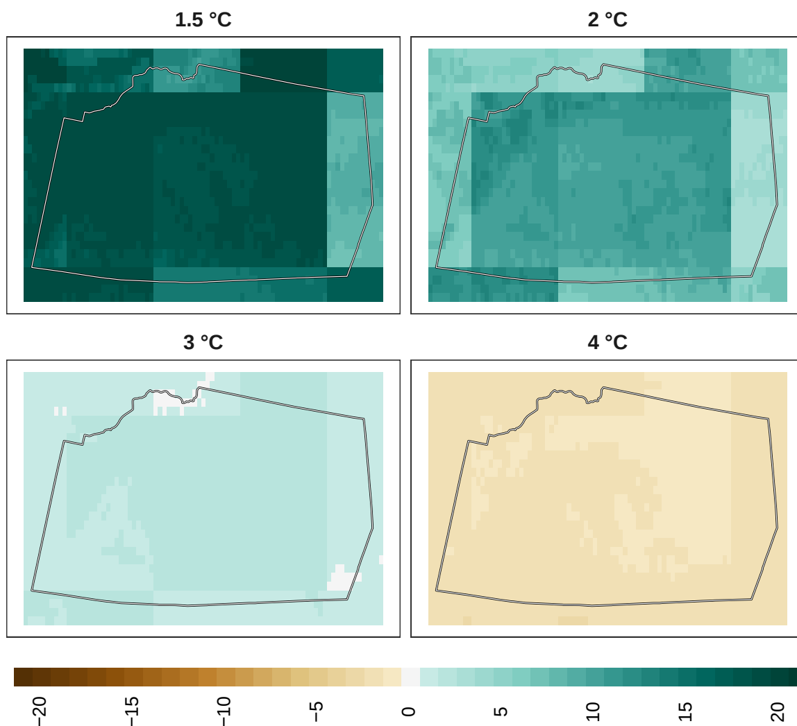
Figure 14: Adaptation effort for plants at 1 km resolution.
