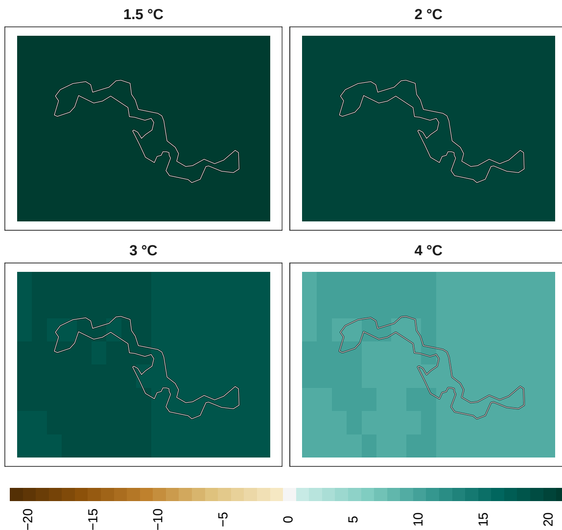
Figure 15: Adaptation effort for birds at 1 km resolution.
