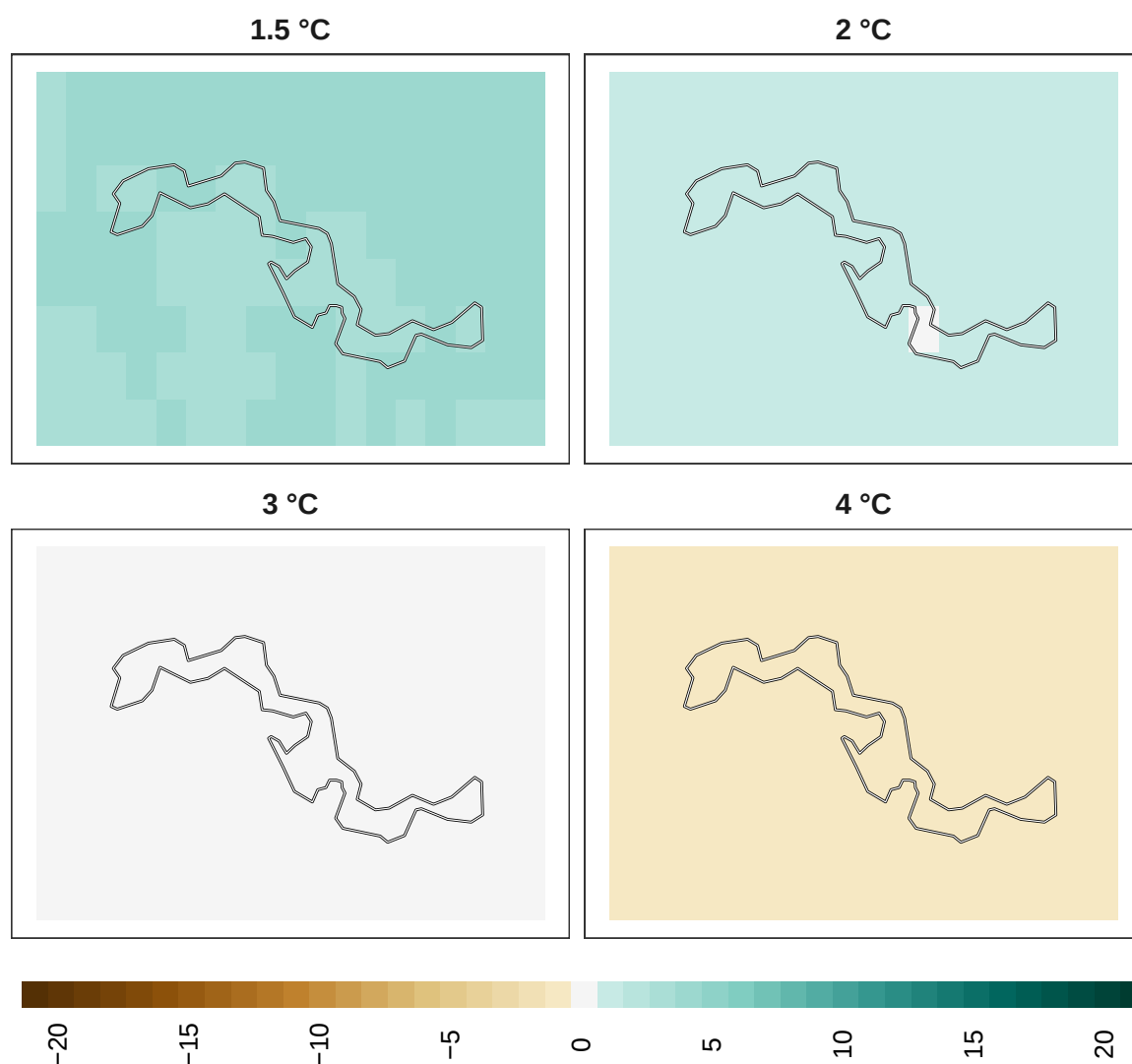
Figure 13: Adaptation effort for overall biodiversity at 1 km resolution.
