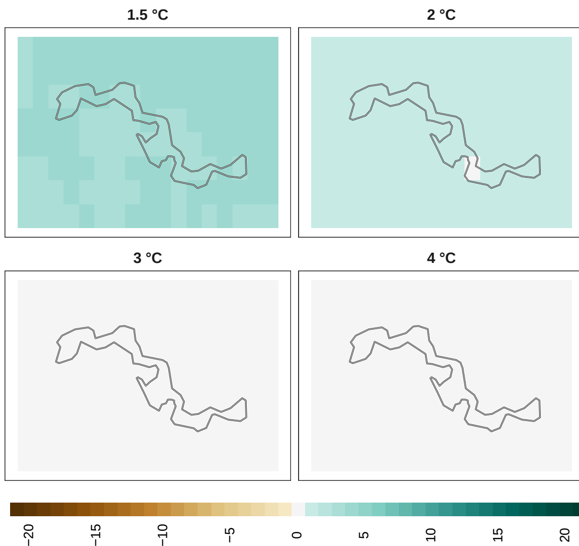
Figure 14: Adaptation effort for plants at 1 km resolution.
