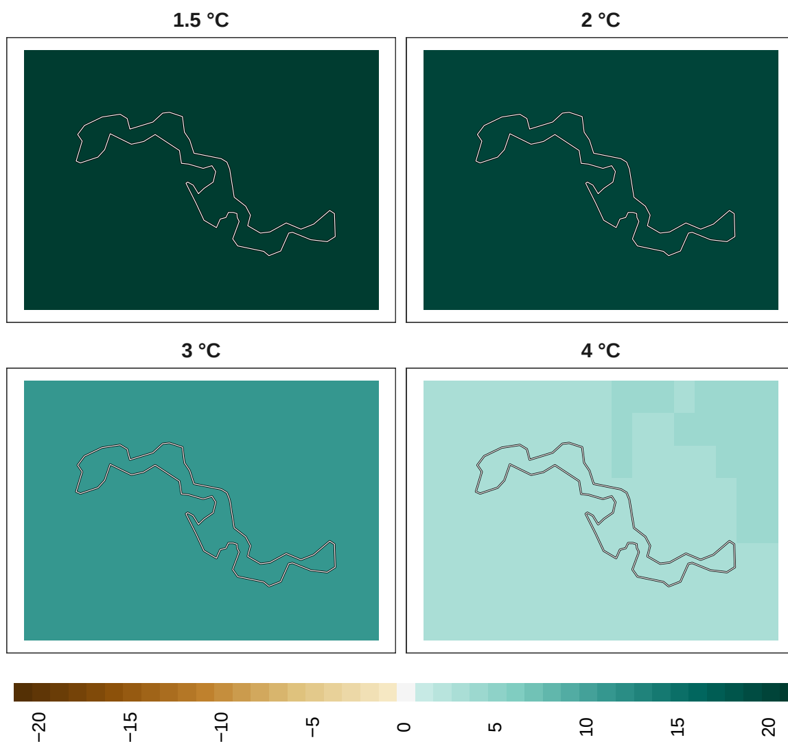
Figure 16: Adaptation effort for mammals at 1 km resolution.
