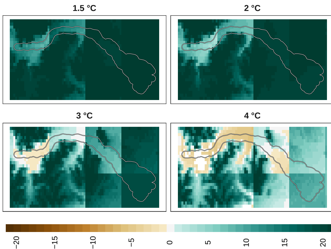
Figure 18: Adaptation effort for insects at 1 km resolution.
