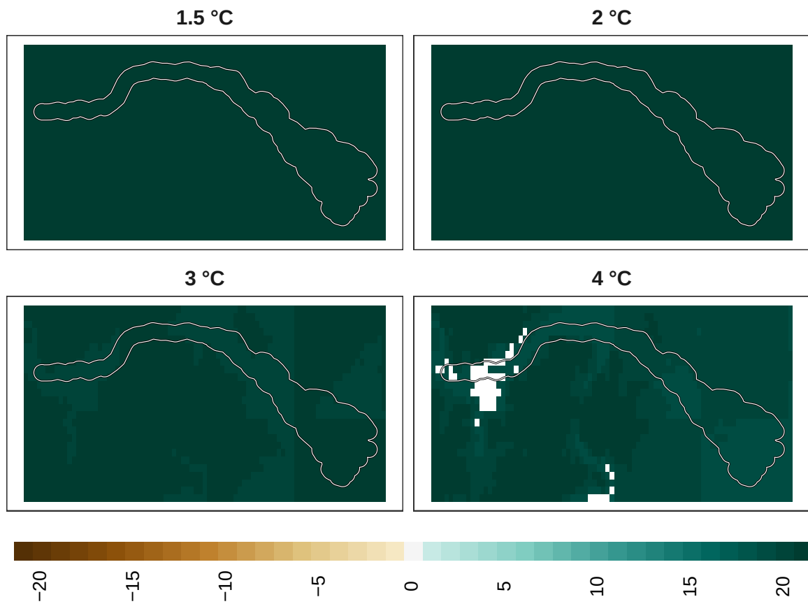
Figure 16: Adaptation effort for birds at 1 km resolution.
