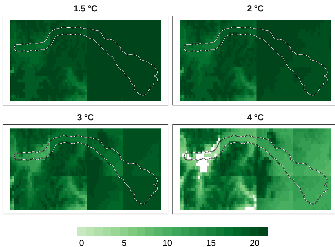
Figure 11: Number of models in agreement for mammal refugia at 1 km resolution.
