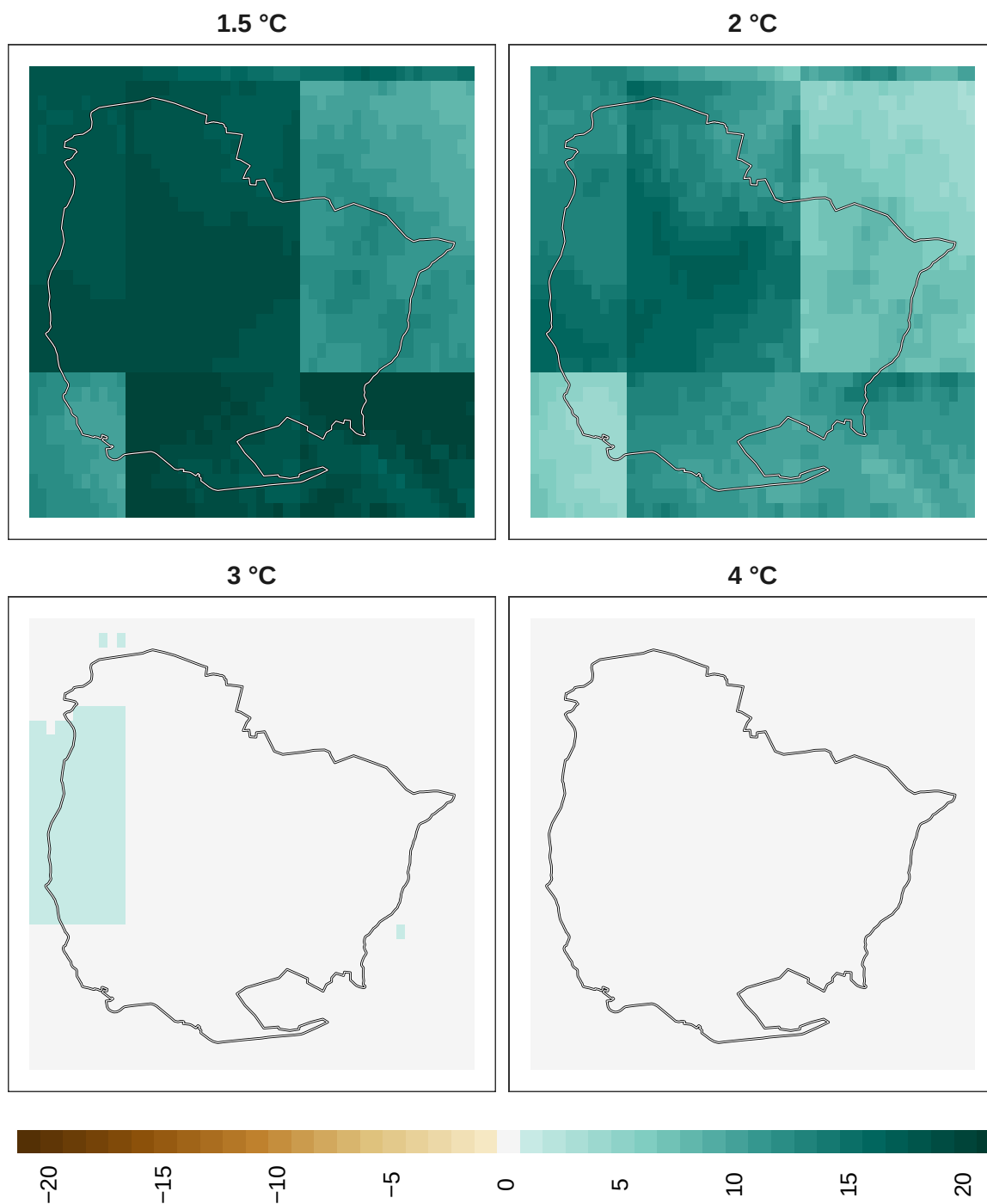
Figure 15: Adaptation effort for birds at 1 km resolution.
