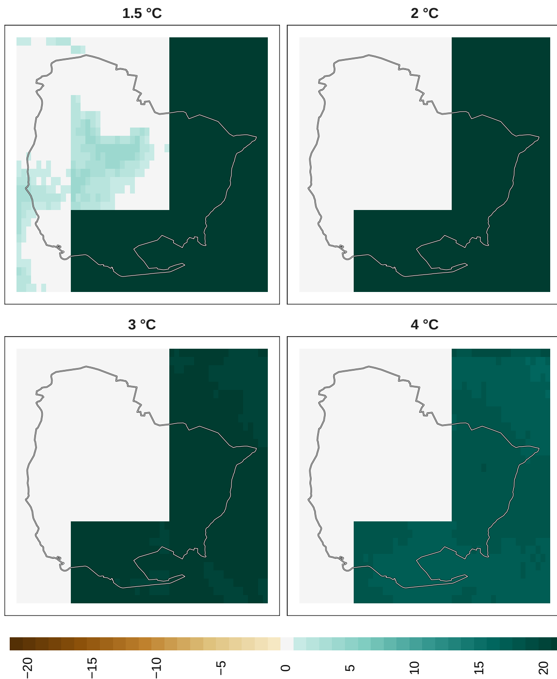
Figure 16: Adaptation effort for mammals at 1 km resolution.
