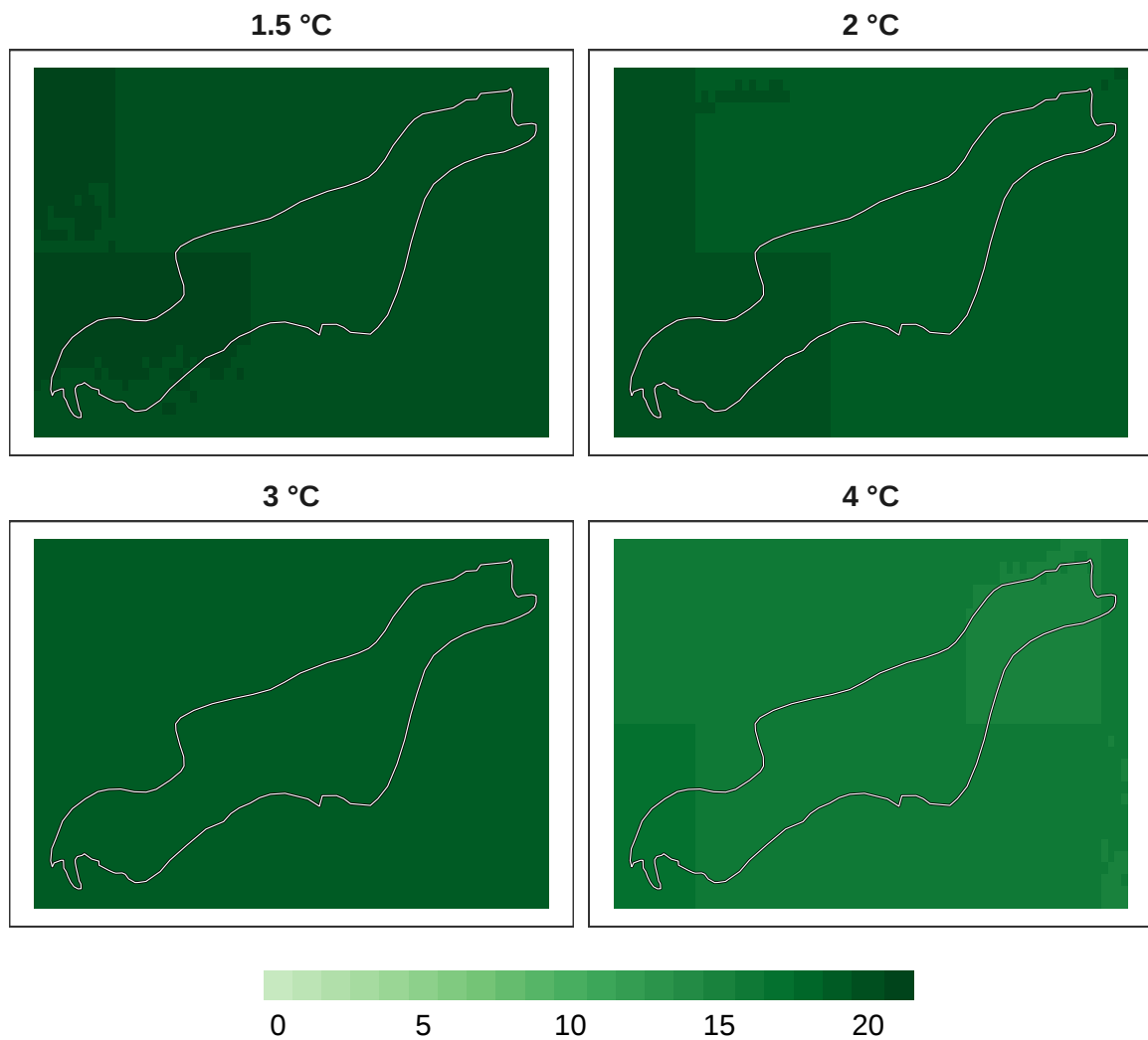
Figure 11: Number of models in agreement for reptile refugia at 1 km resolution.
