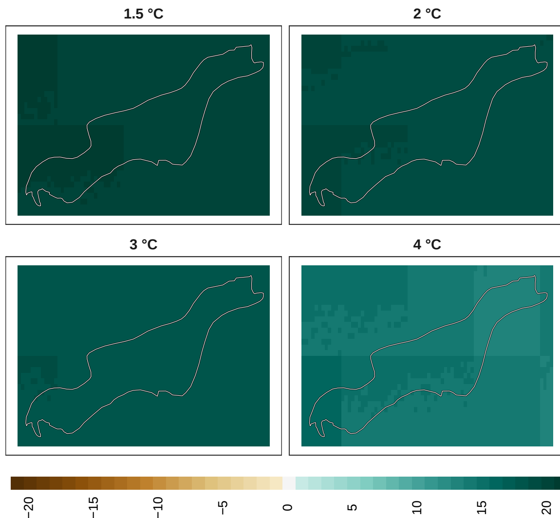
Figure 17: Adaptation effort for reptiles at 1 km resolution.
