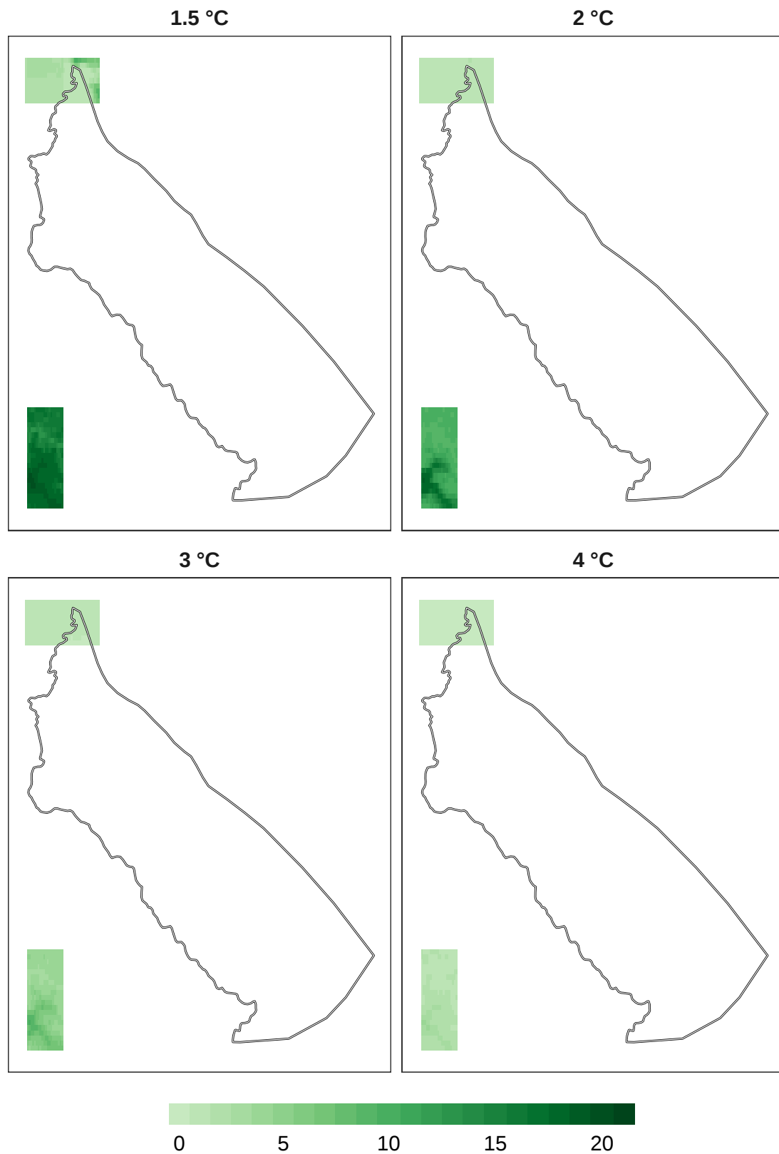
Figure 7: Number of models in agreement for mammal refugia at 1 km resolution.
