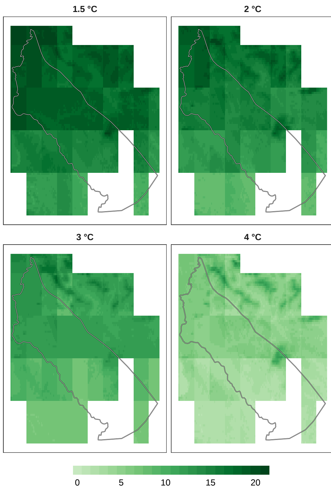
Figure 8: Number of models in agreement for insect refugia at 1 km resolution.
