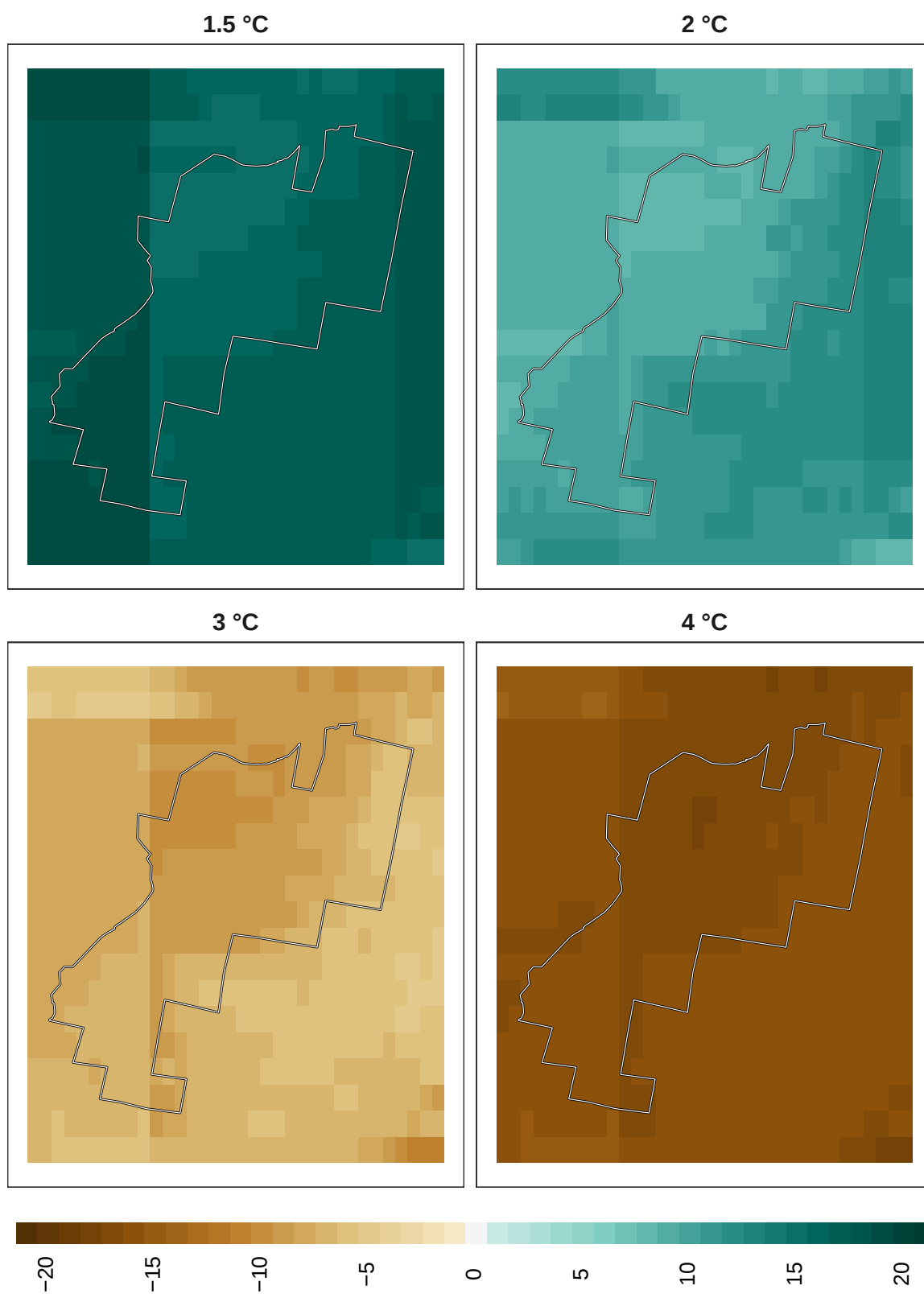
Figure 15: Adaptation effort for pollinators at 1 km resolution.
