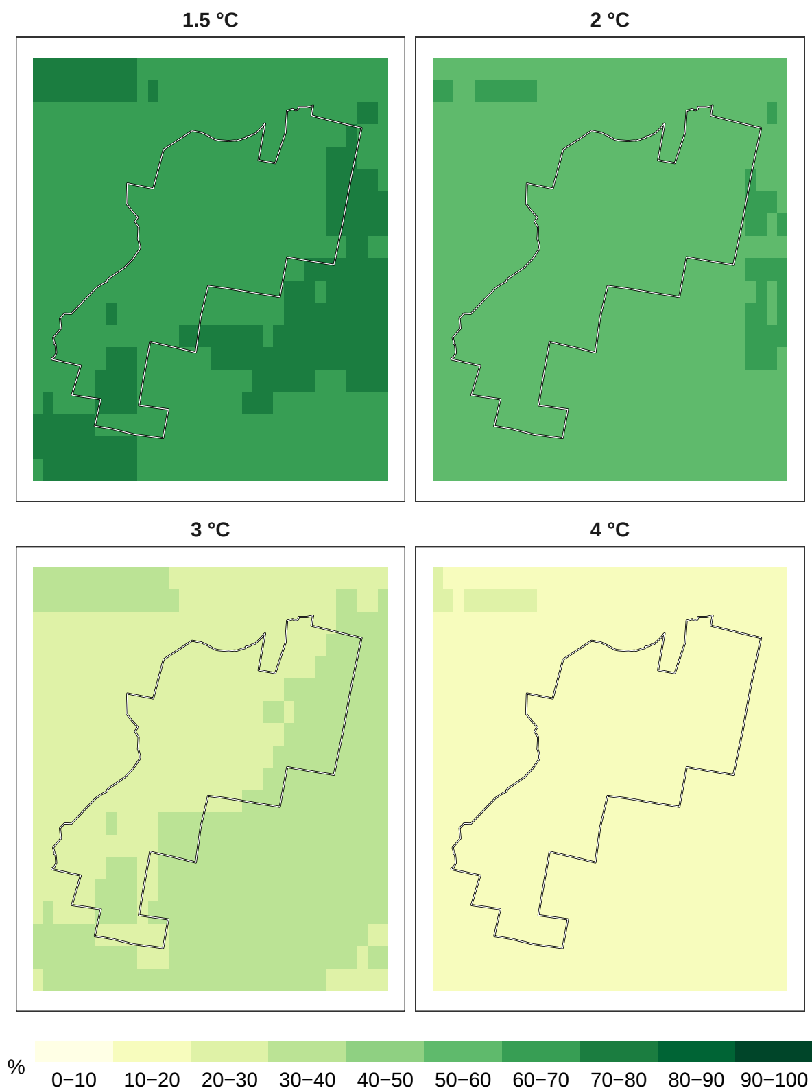
Figure 4: Percent insects remaining at 1 km resolution.
