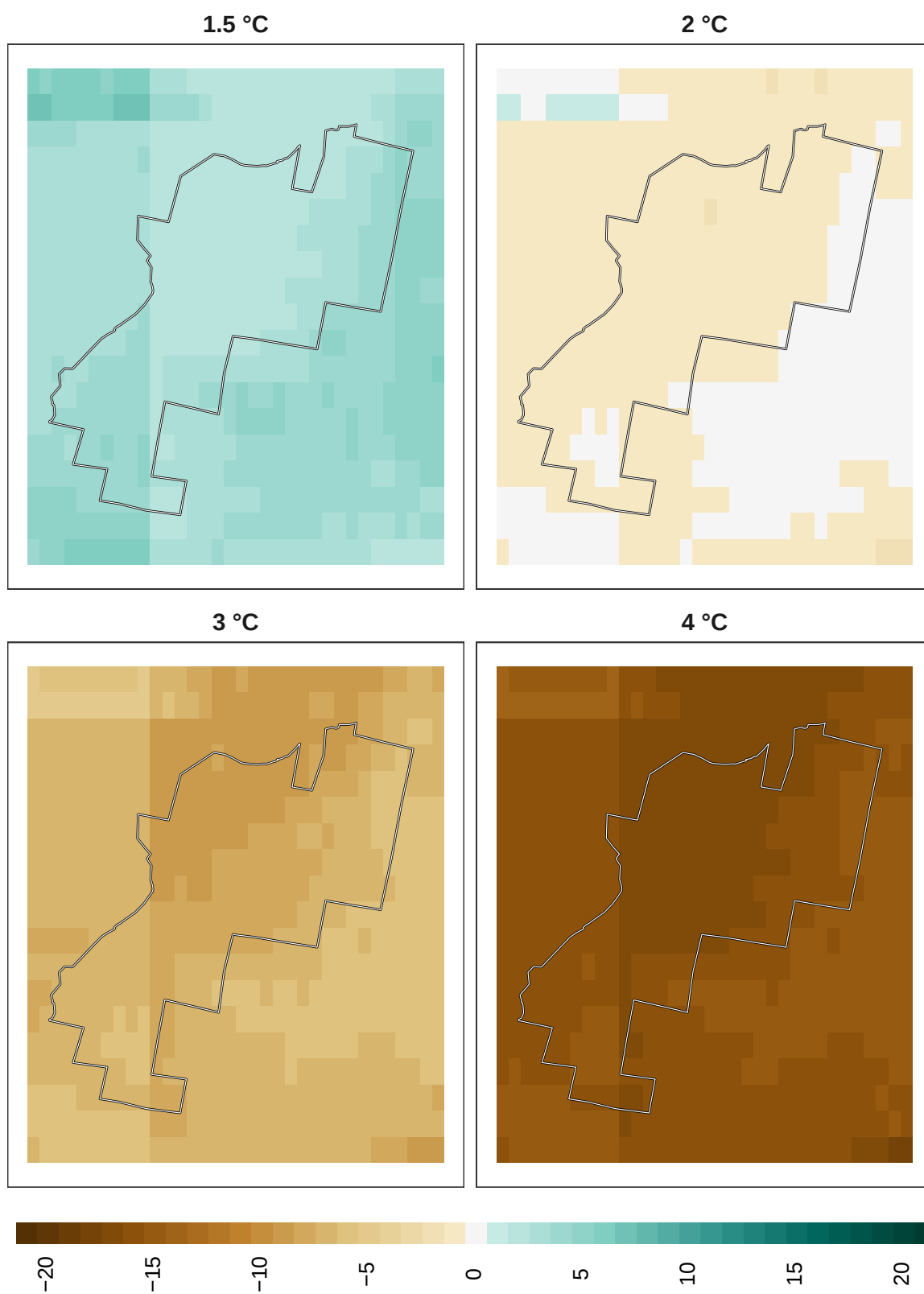
Figure 14: Adaptation effort for insects at 1 km resolution.
