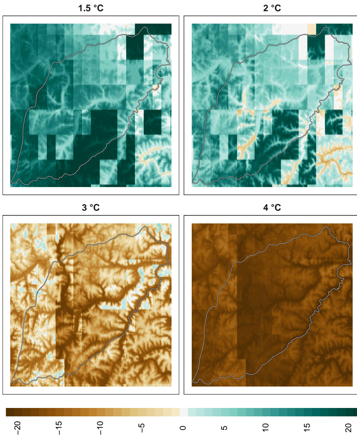
Figure 5: Adaptation effort for overall biodiversity at 1 km resolution.
