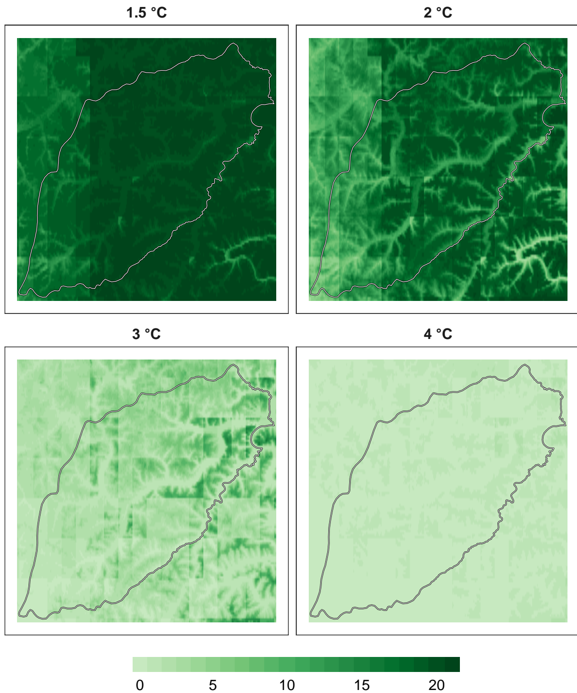
Figure 4: Number of models in agreement for plant refugia at 1 km resolution.
