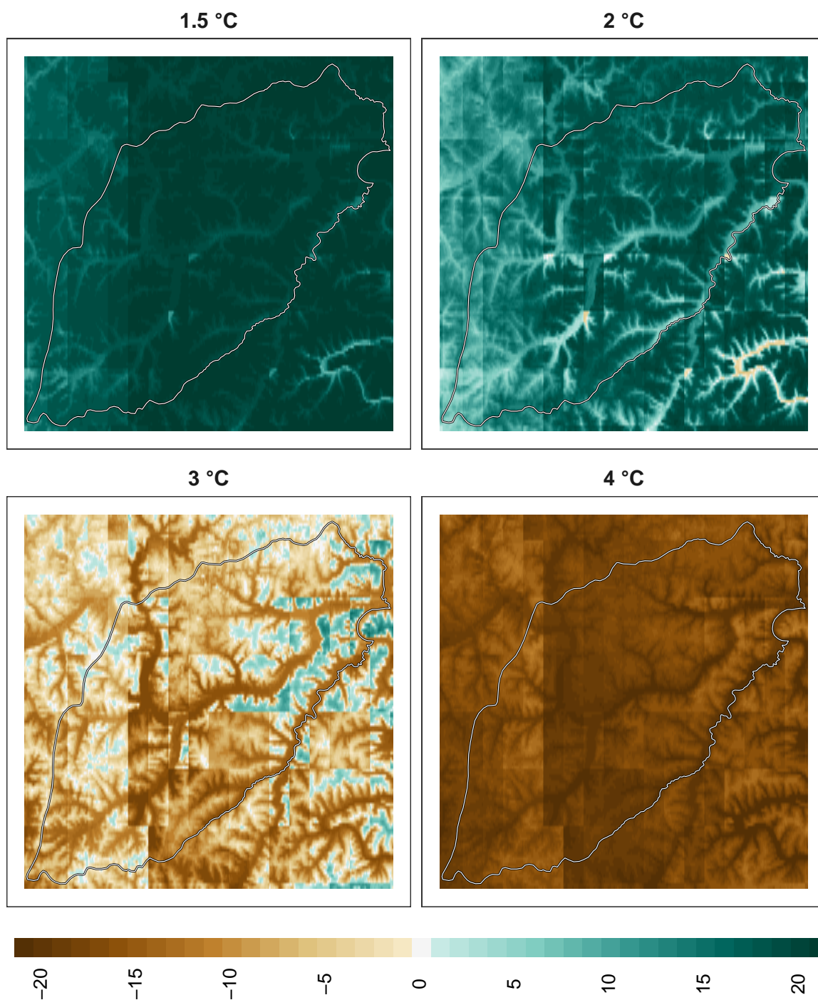
Figure 6: Adaptation effort for plants at 1 km resolution.
