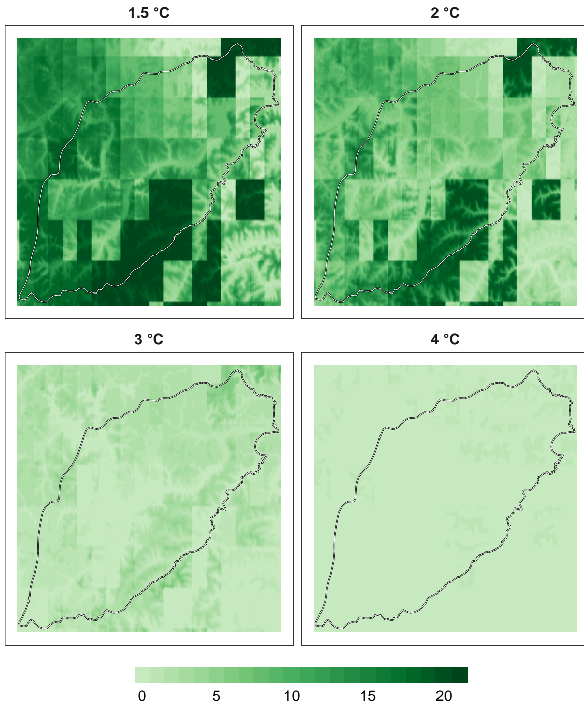
Figure 3: Number of models in agreement for overall biodiversity refugia at 1 km resolution.
