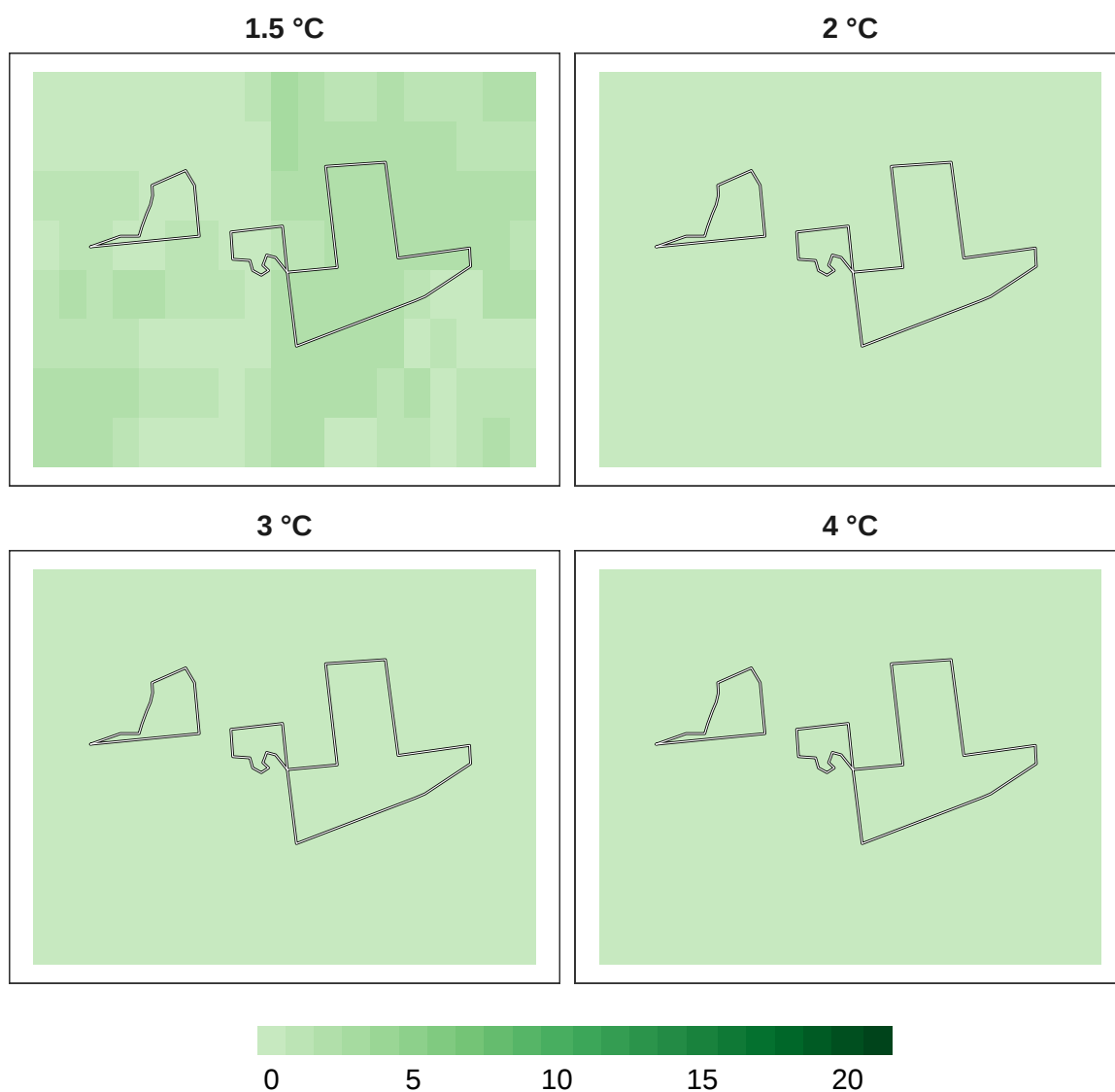
Figure 12: Number of models in agreement for insect refugia at 1 km resolution.
