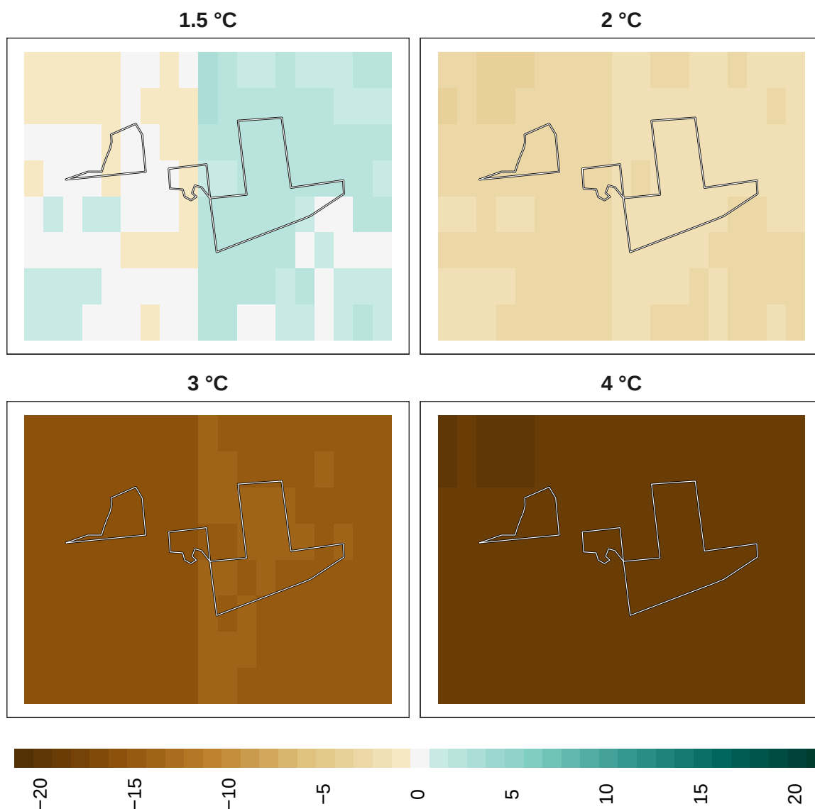
Figure 18: Adaptation effort for insects at 1 km resolution.
