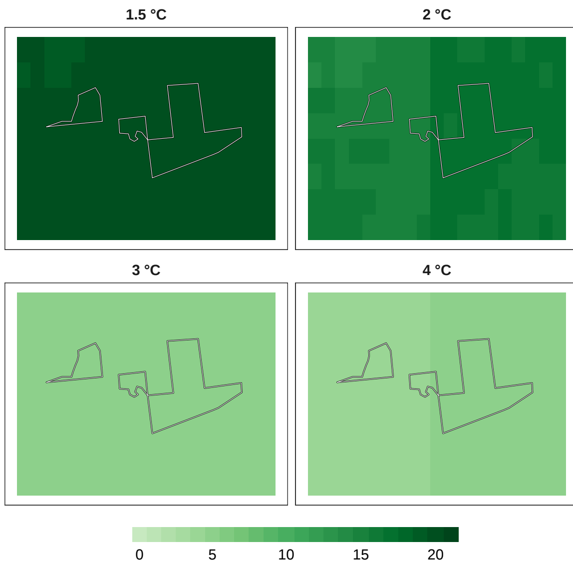
Figure 10: Number of models in agreement for bird refugia.
