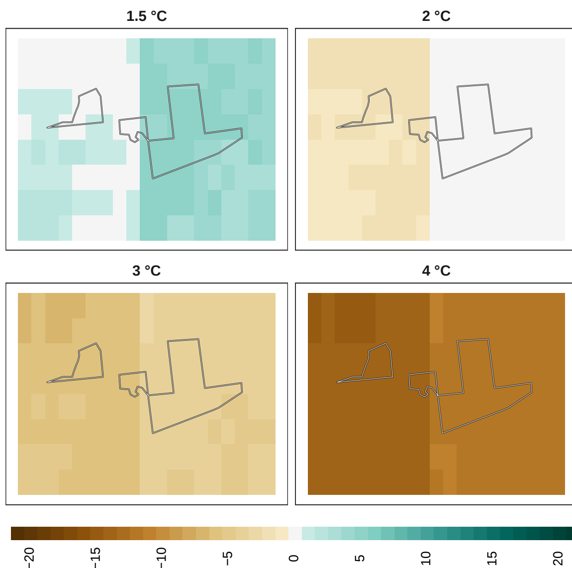
Figure 14: Adaptation effort for overall biodiversity at 1 km resolution.
