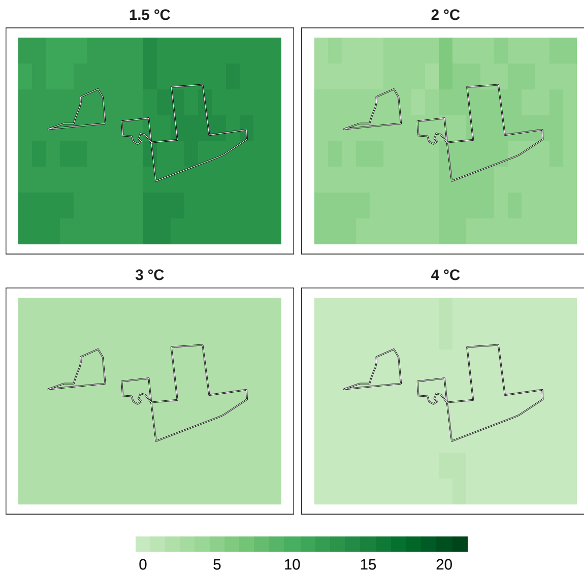
Figure 9: Number of models in agreement for plant refugia at 1 km resolution.
