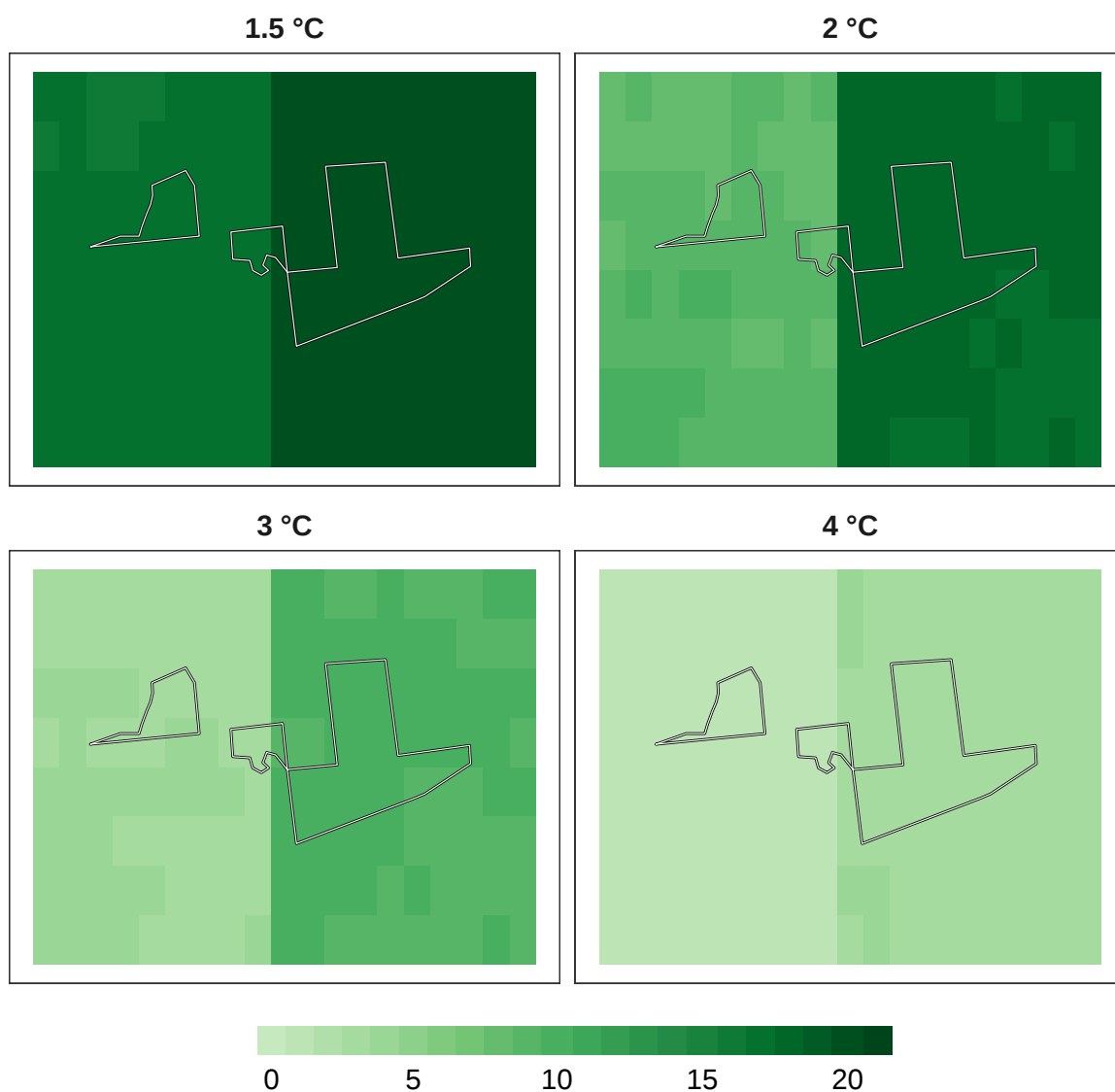
Figure 11: Number of models in agreement for mammal refugia at 1 km resolution.
