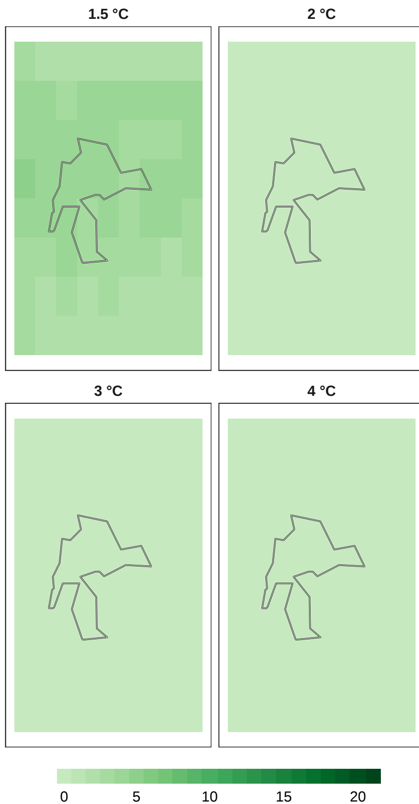
Figure 13: Number of models in agreement for pollinator refugia at 1 km resolution.
