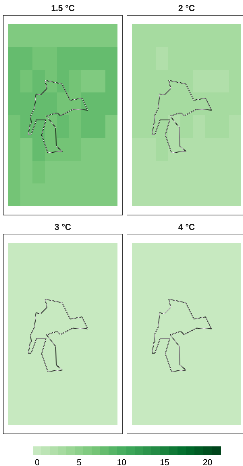
Figure 8: Number of models in agreement for overall biodiversity refugia at 1 km resolution.
