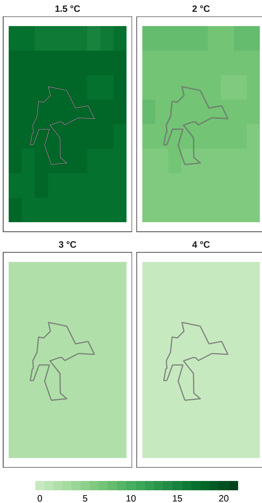
Figure 9: Number of models in agreement for plant refugia at 1 km resolution.
