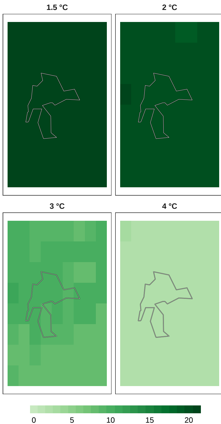
Figure 11: Number of models in agreement for mammal refugia at 1 km resolution.
