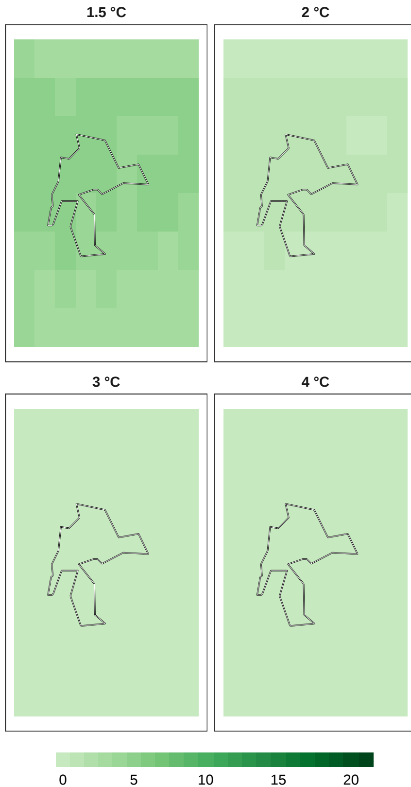
Figure 12: Number of models in agreement for insect refugia at 1 km resolution.
