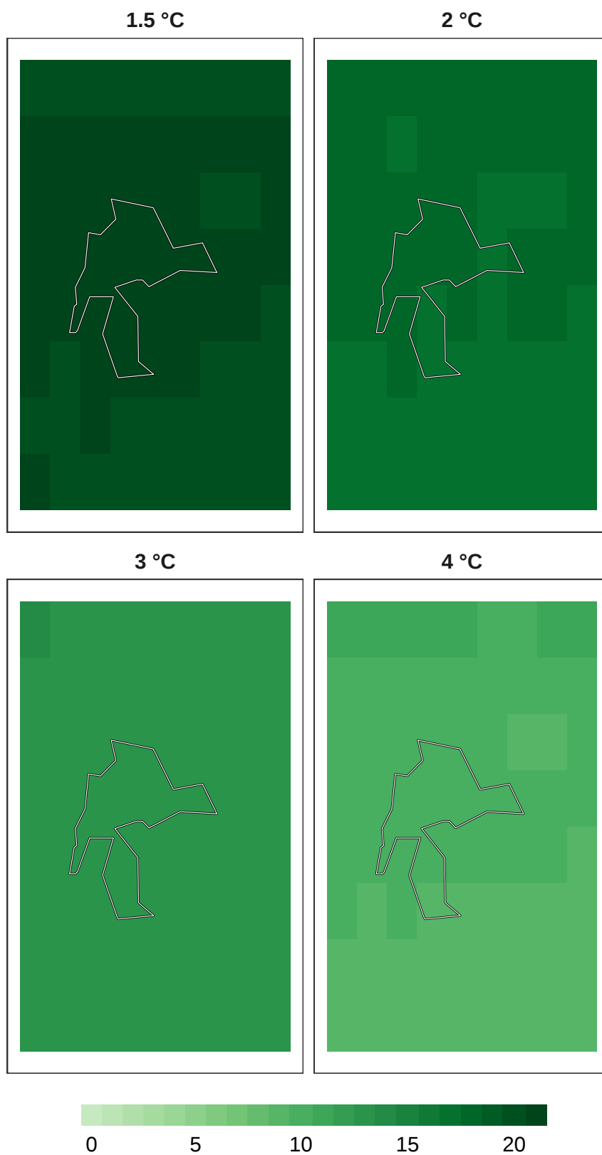
Figure 10: Number of models in agreement for bird refugia.
