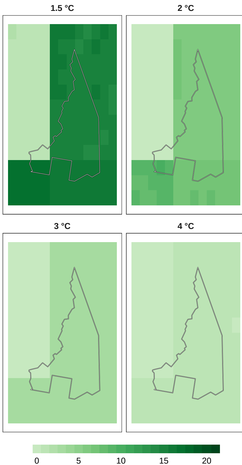
Figure 10: Number of models in agreement for plant refugia at 1 km resolution.
