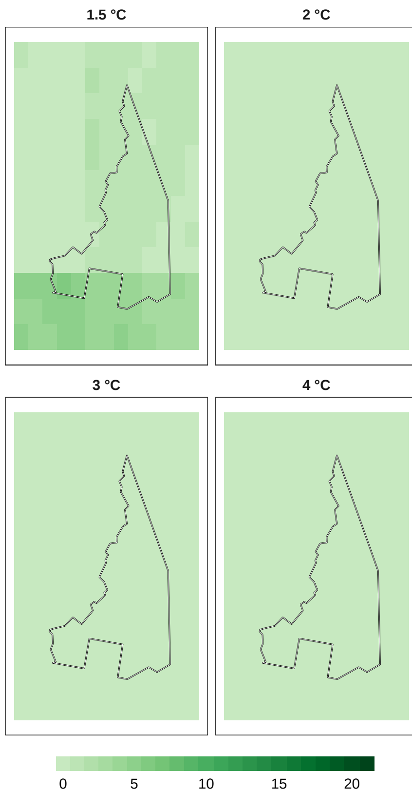
Figure 14: Number of models in agreement for insect refugia at 1 km resolution.
