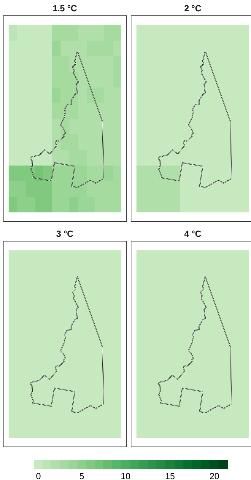
Figure 9: Number of models in agreement for overall biodiversity refugia at 1 km resolution.
