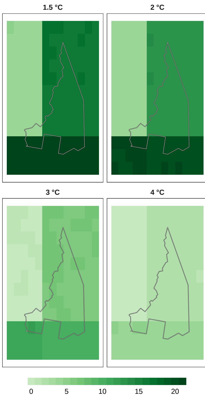
Figure 12: Number of models in agreement for mammal refugia at 1 km resolution.
