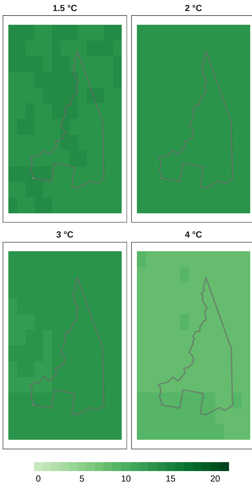
Figure 13: Number of models in agreement for reptile refugia at 1 km resolution.
