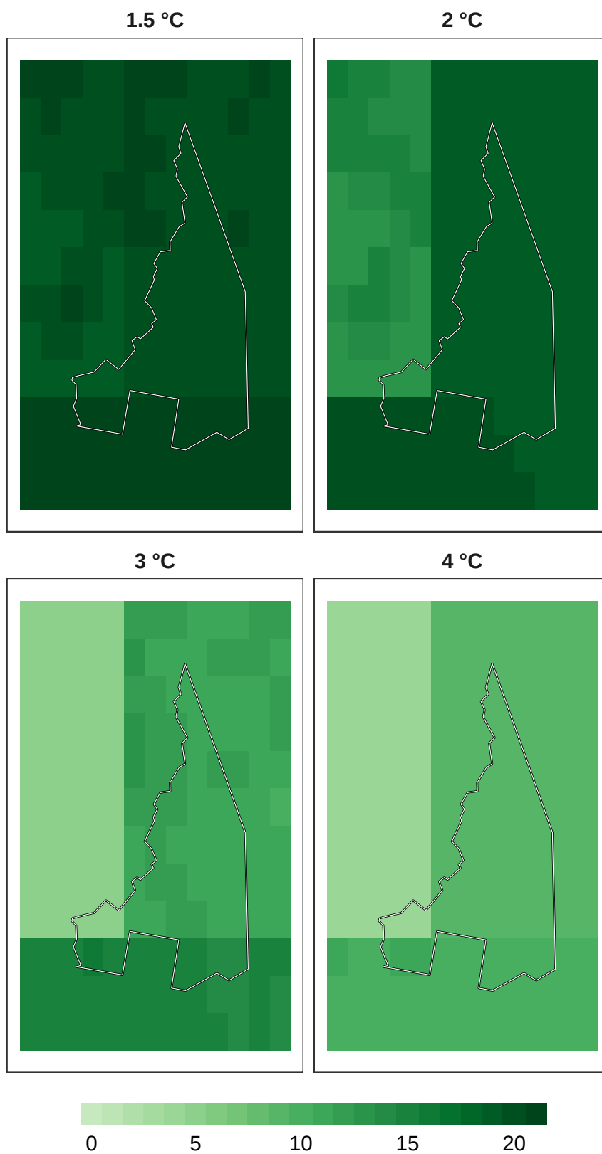
Figure 11: Number of models in agreement for bird refugia.
