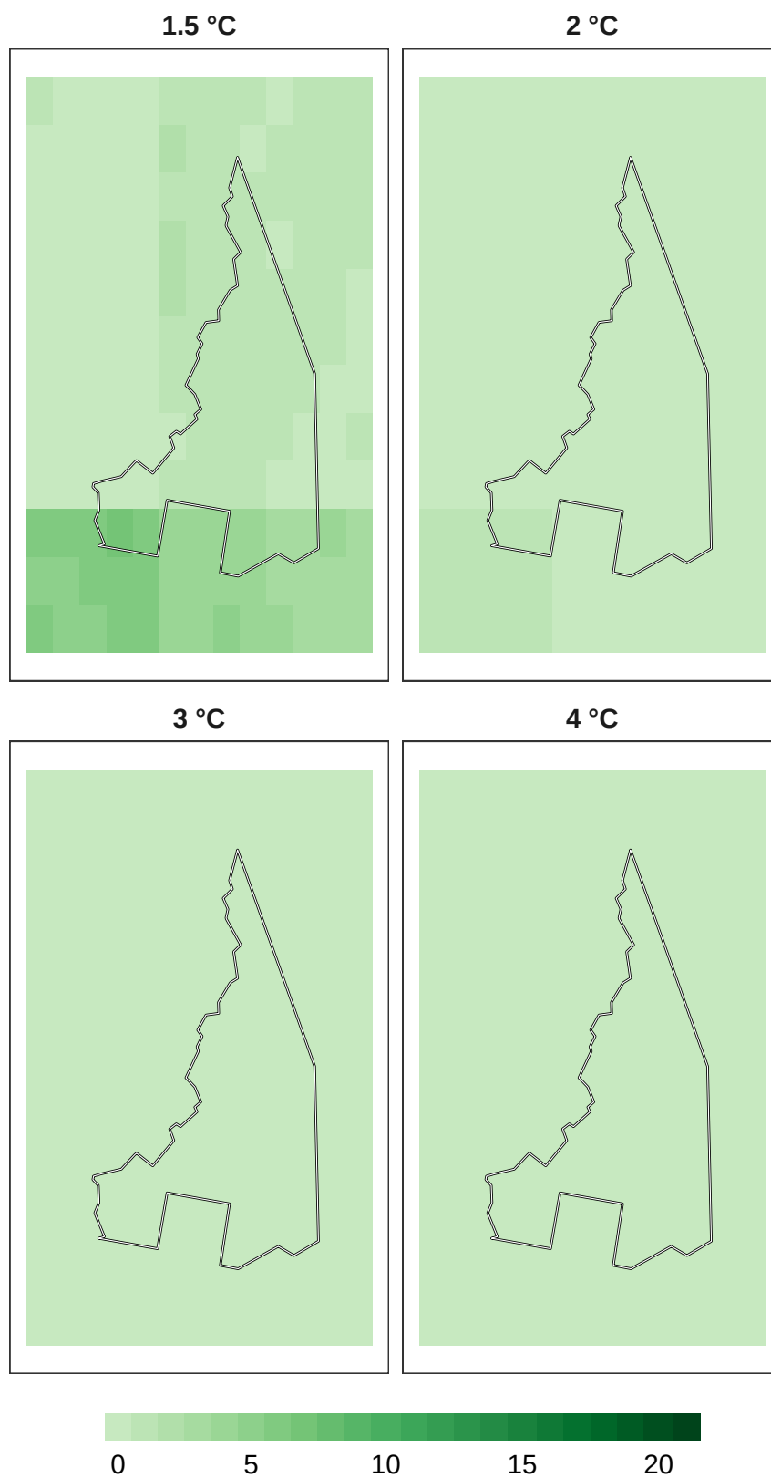
Figure 15: Number of models in agreement for pollinator refugia at 1 km resolution.
