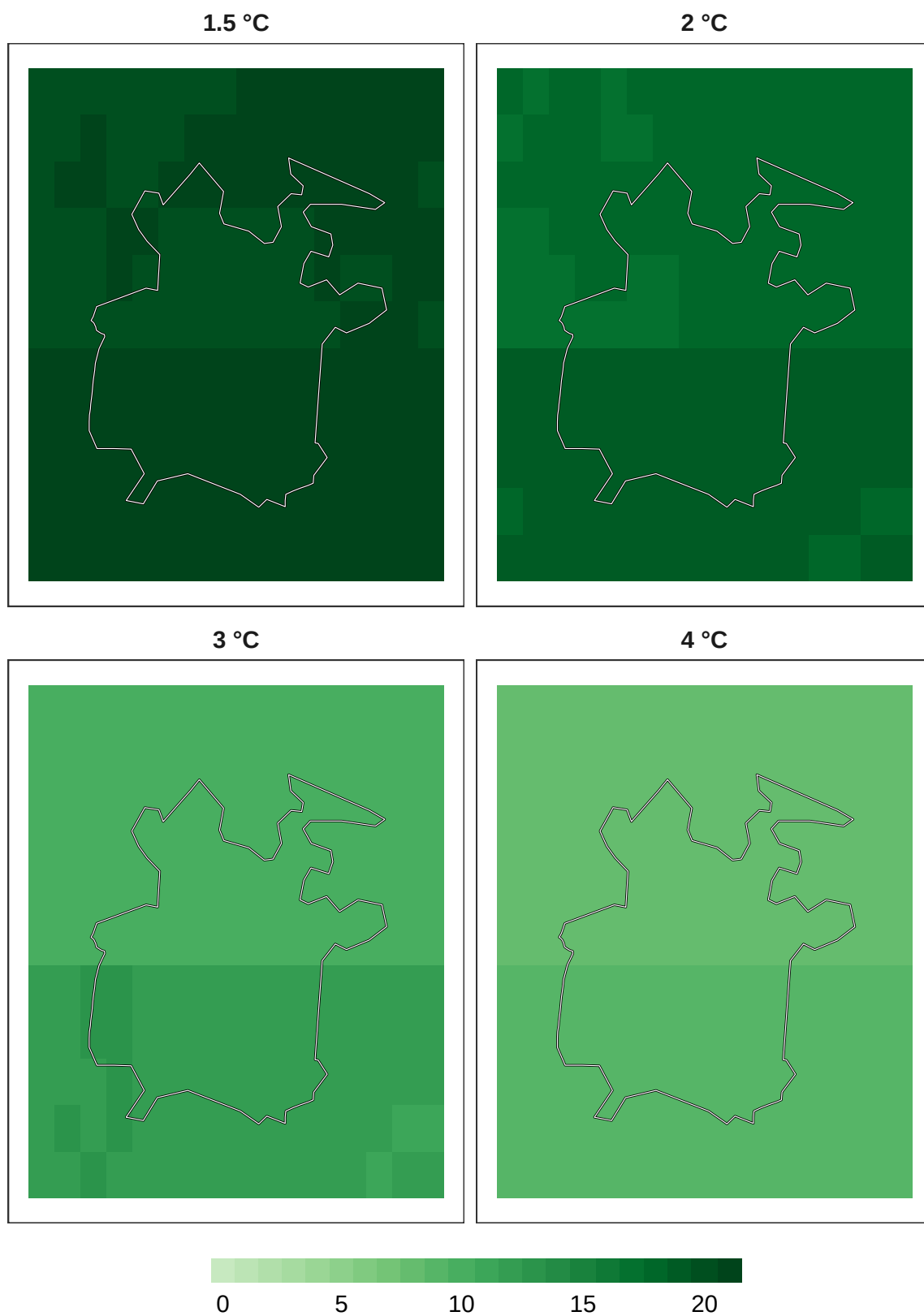
Figure 11: Number of models in agreement for bird refugia.
