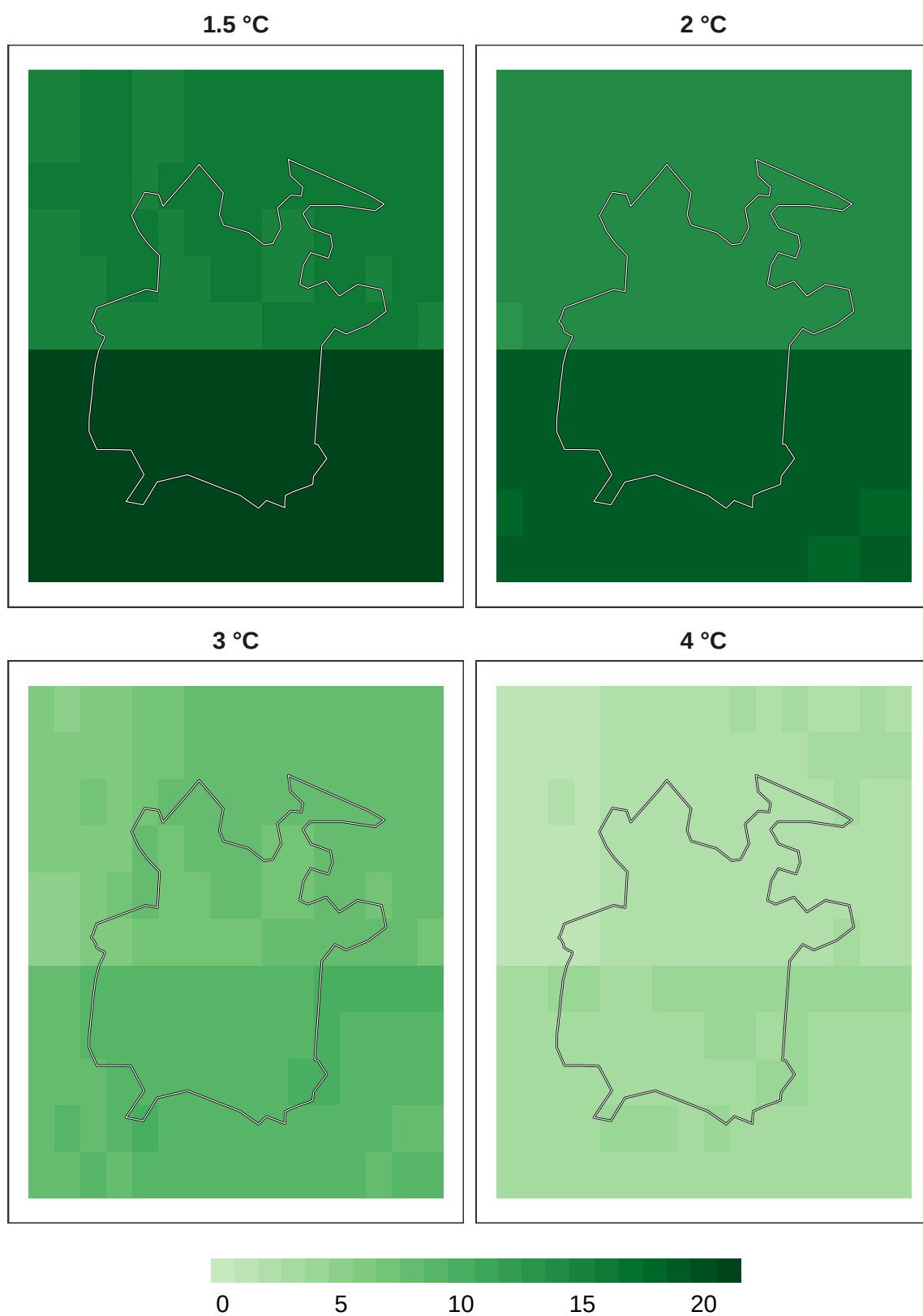
Figure 12: Number of models in agreement for mammal refugia at 1 km resolution.
