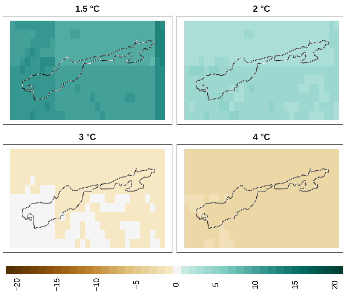
Figure 15: Adaptation effort for plants at 1 km resolution.
