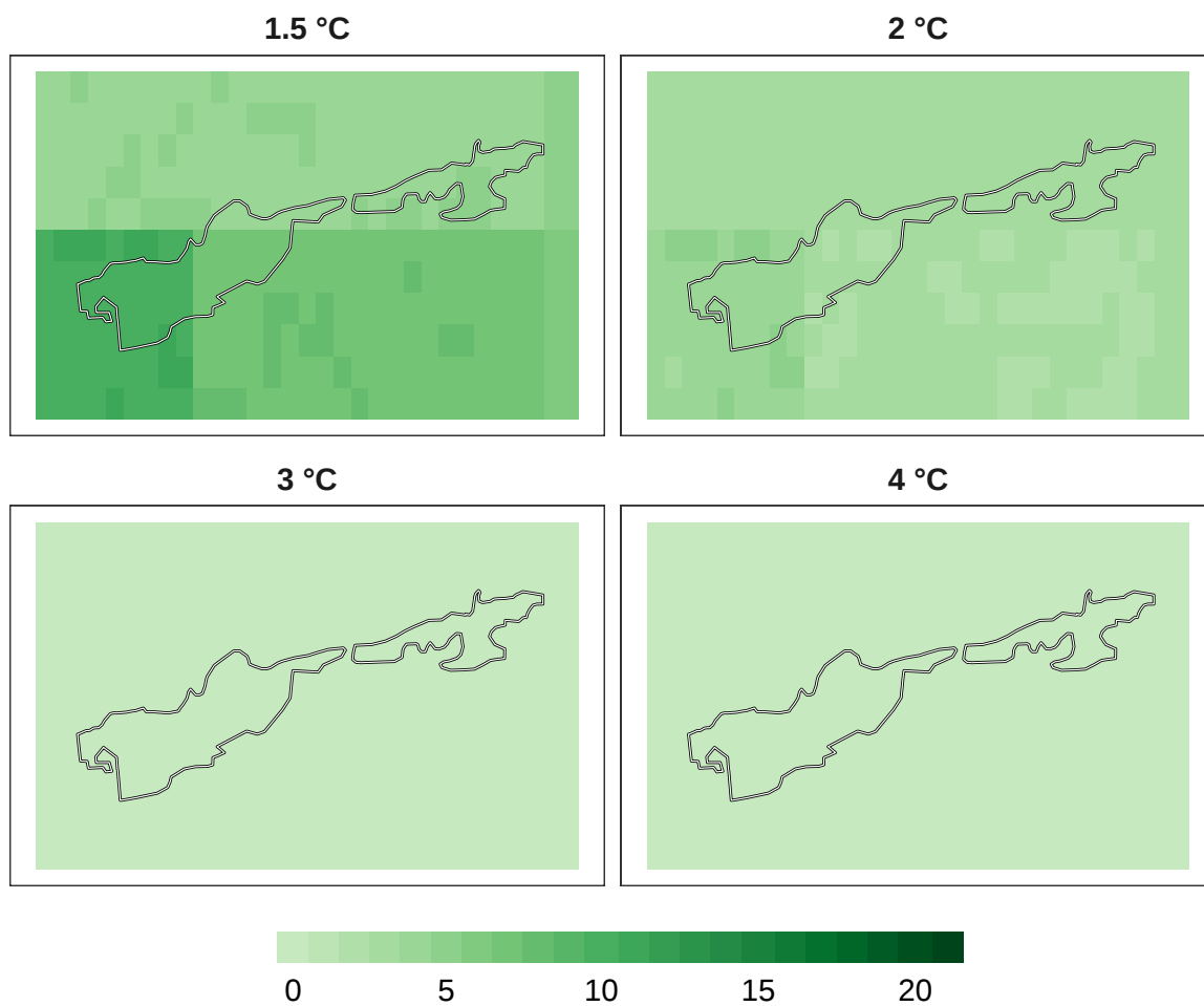
Figure 8: Number of models in agreement for overall biodiversity refugia at 1 km resolution.
