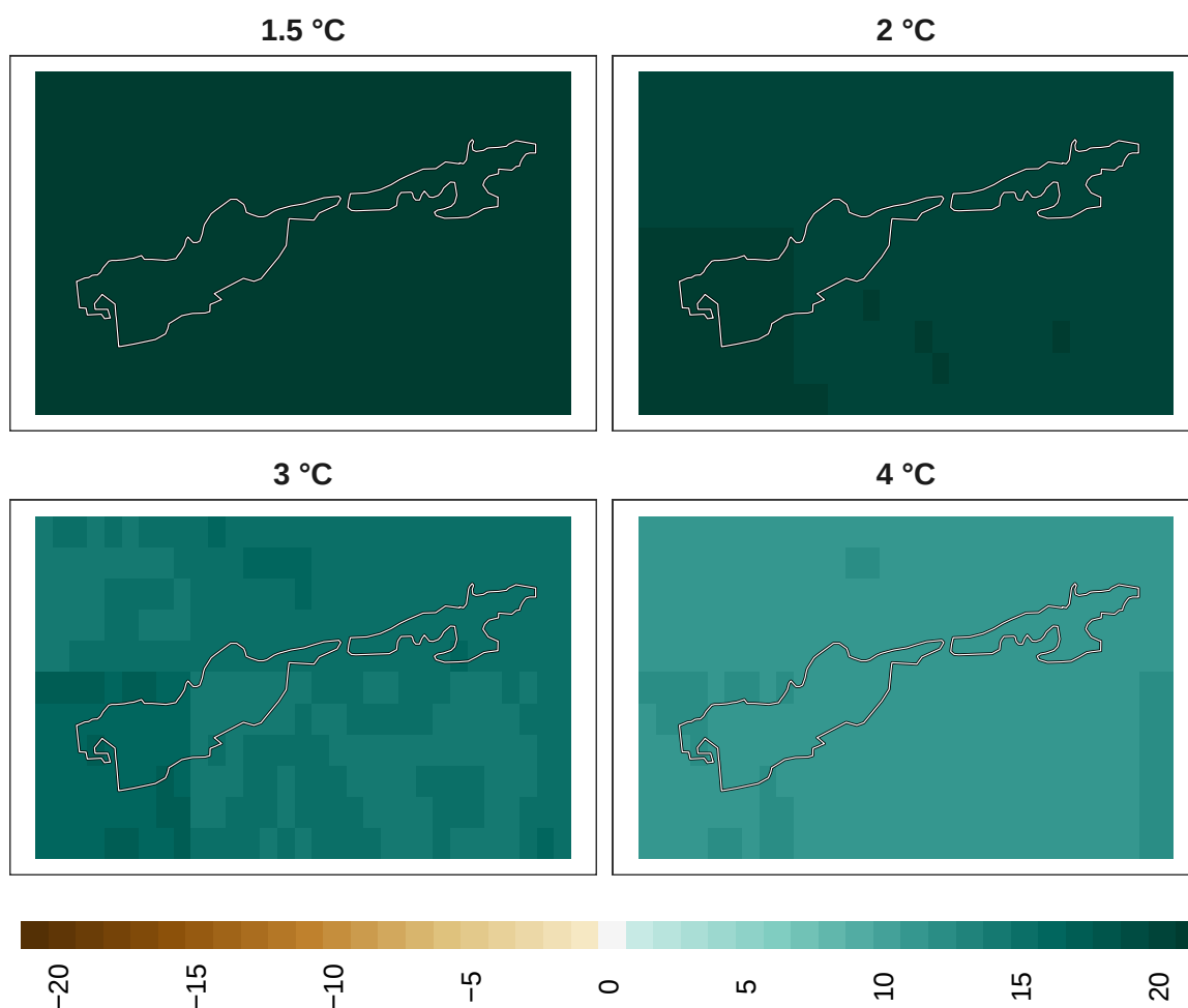
Figure 16: Adaptation effort for birds at 1 km resolution.
