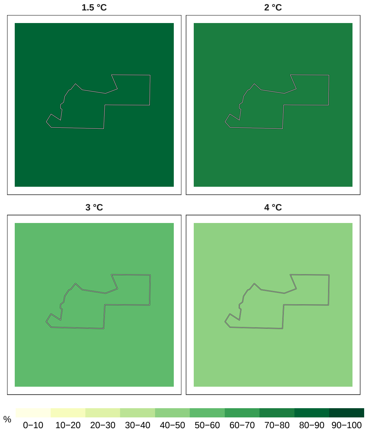
Figure 2: Percent plants remaining at 1 km resolution.
