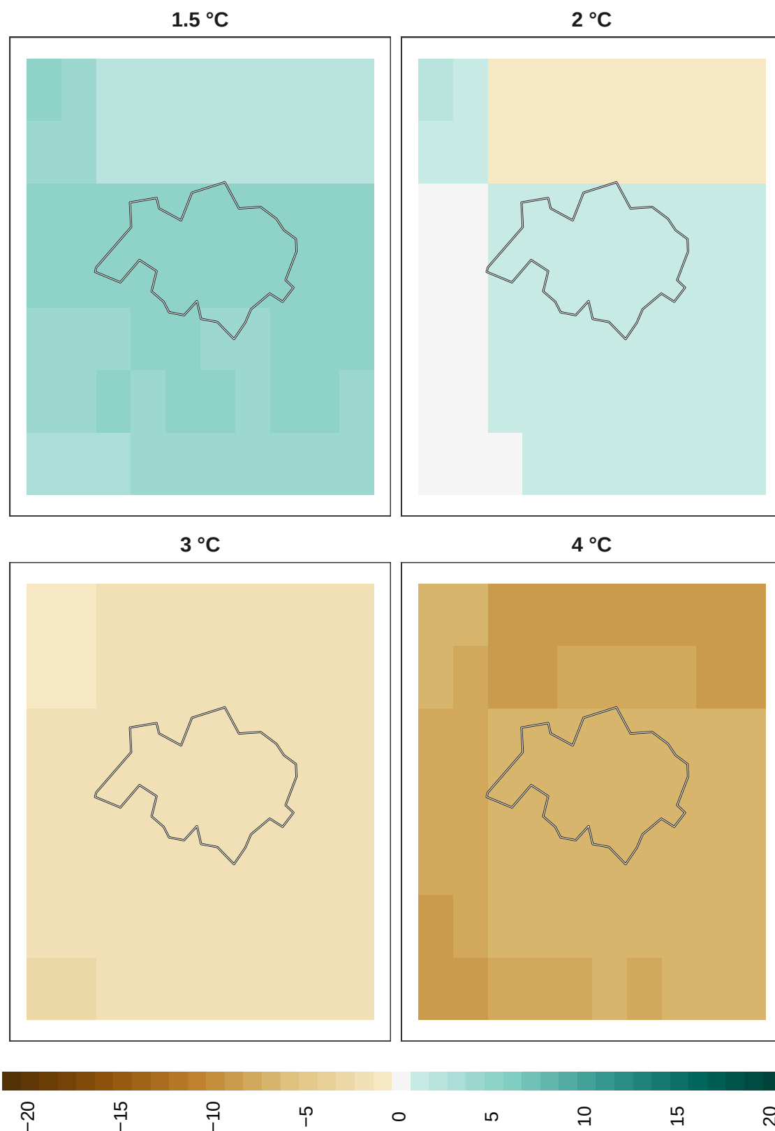
Figure 16: Adaptation effort for overall biodiversity at 1 km resolution.
