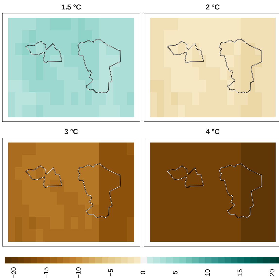
Figure 22: Adaptation effort for pollinators at 1 km resolution.
