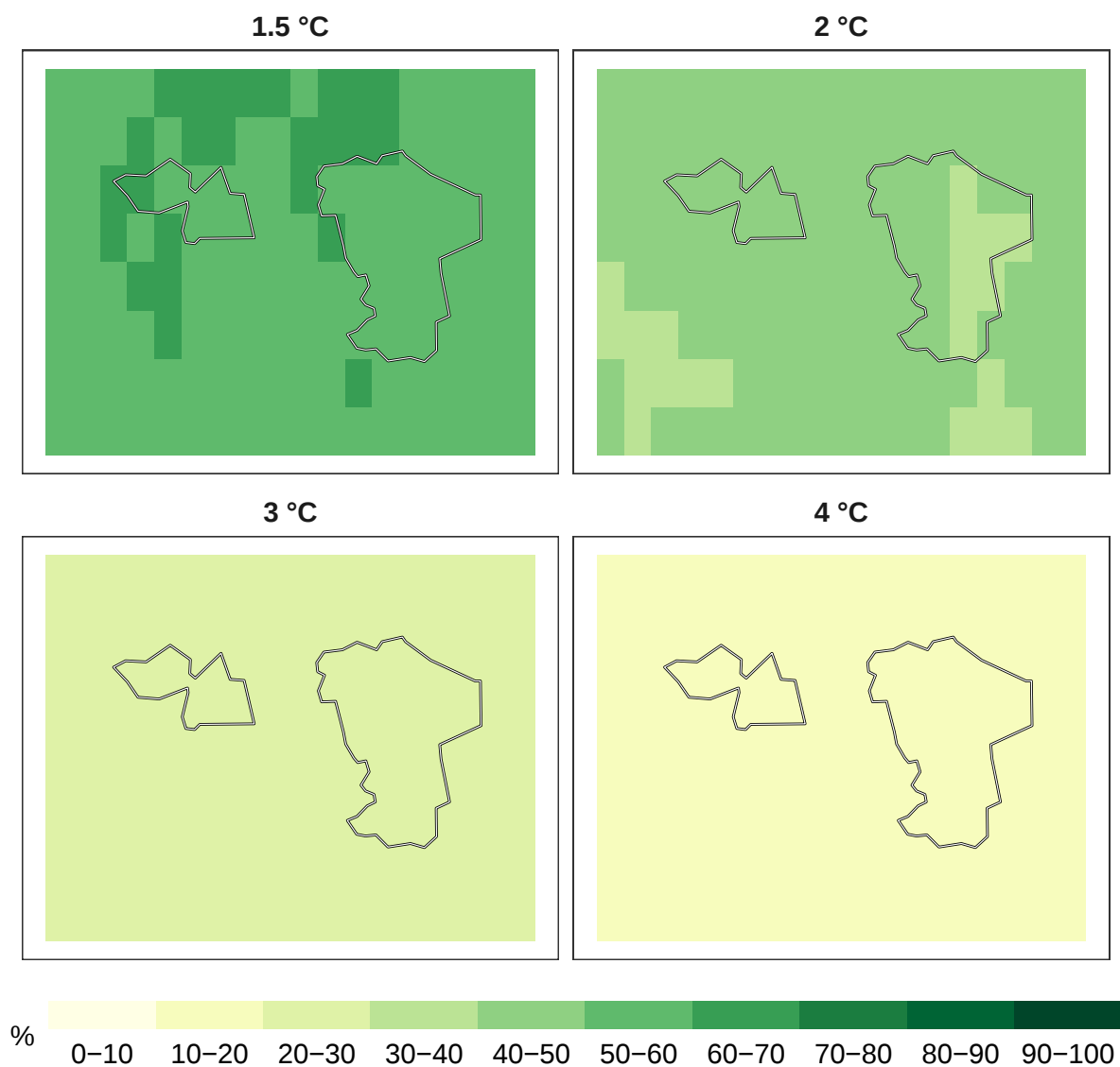
Figure 7: Percent pollinators remaining at 1 km resolution.
