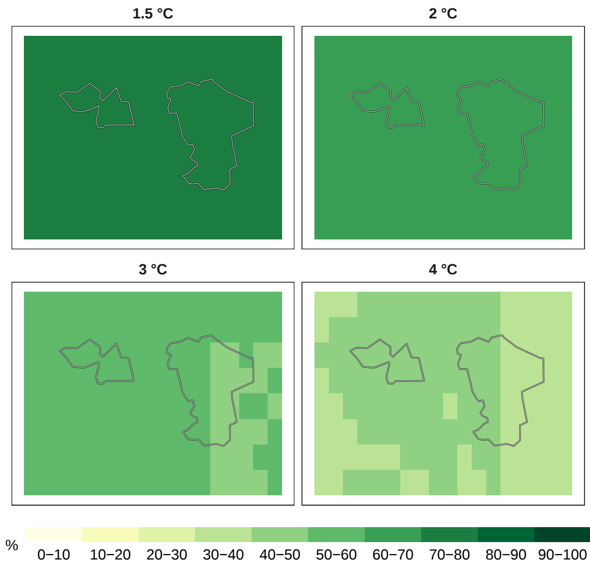
Figure 1: Percent overall biodiversity remaining at 1 km resolution.
