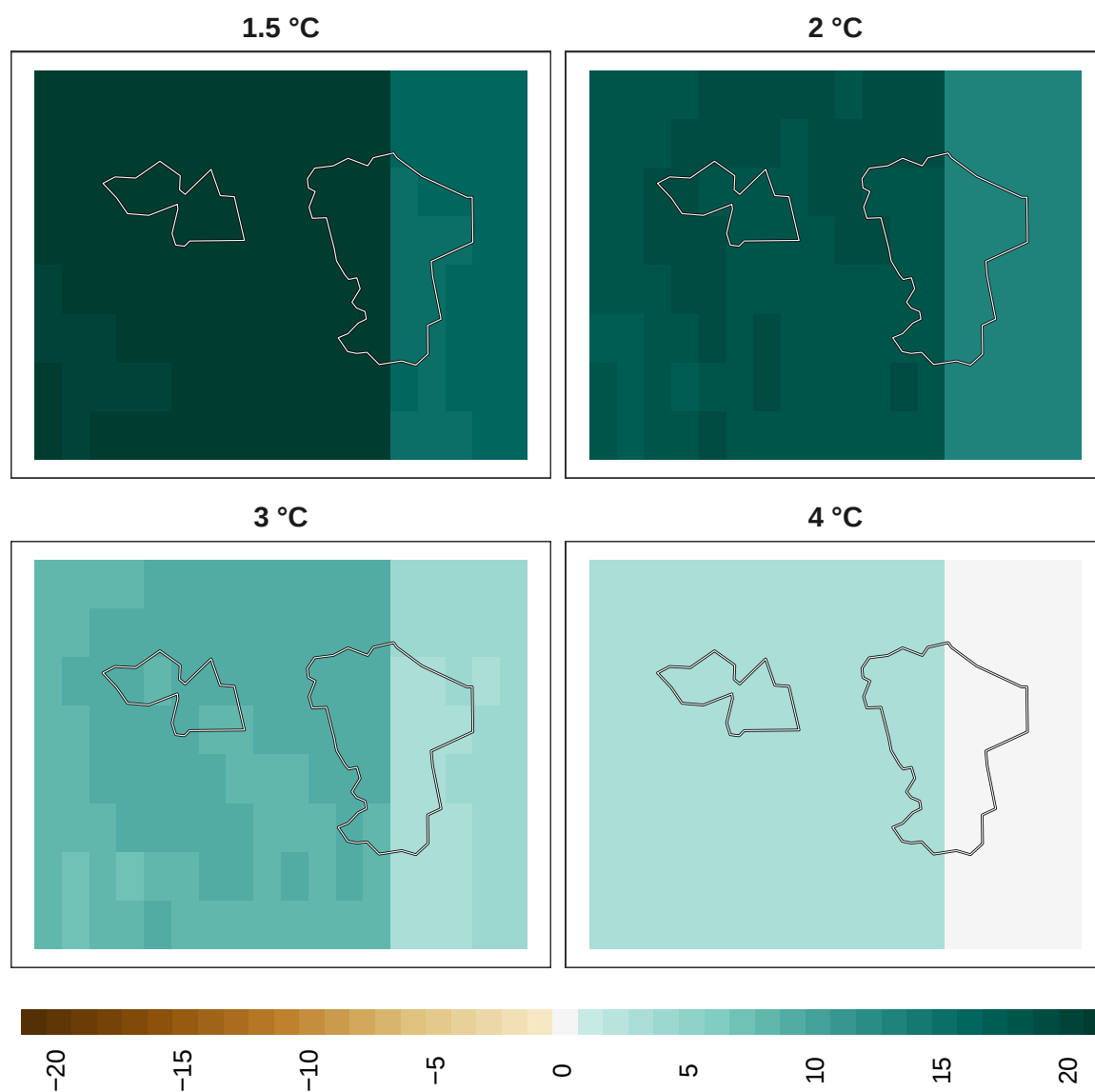
Figure 19: Adaptation effort for mammals at 1 km resolution.
