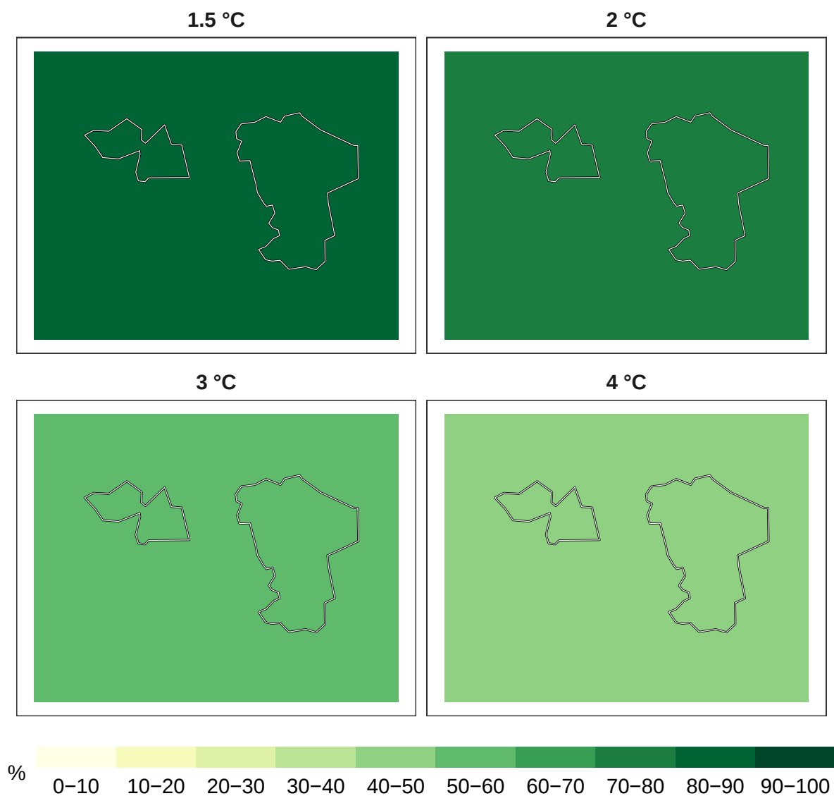
Figure 2: Percent plants remaining at 1 km resolution.
