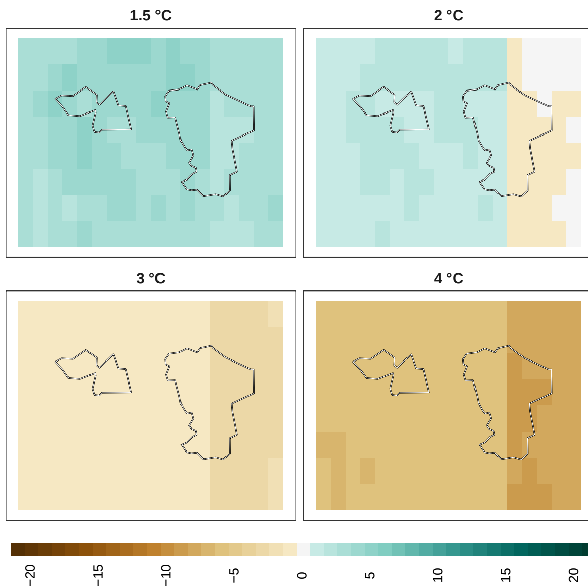
Figure 16: Adaptation effort for overall biodiversity at 1 km resolution.
