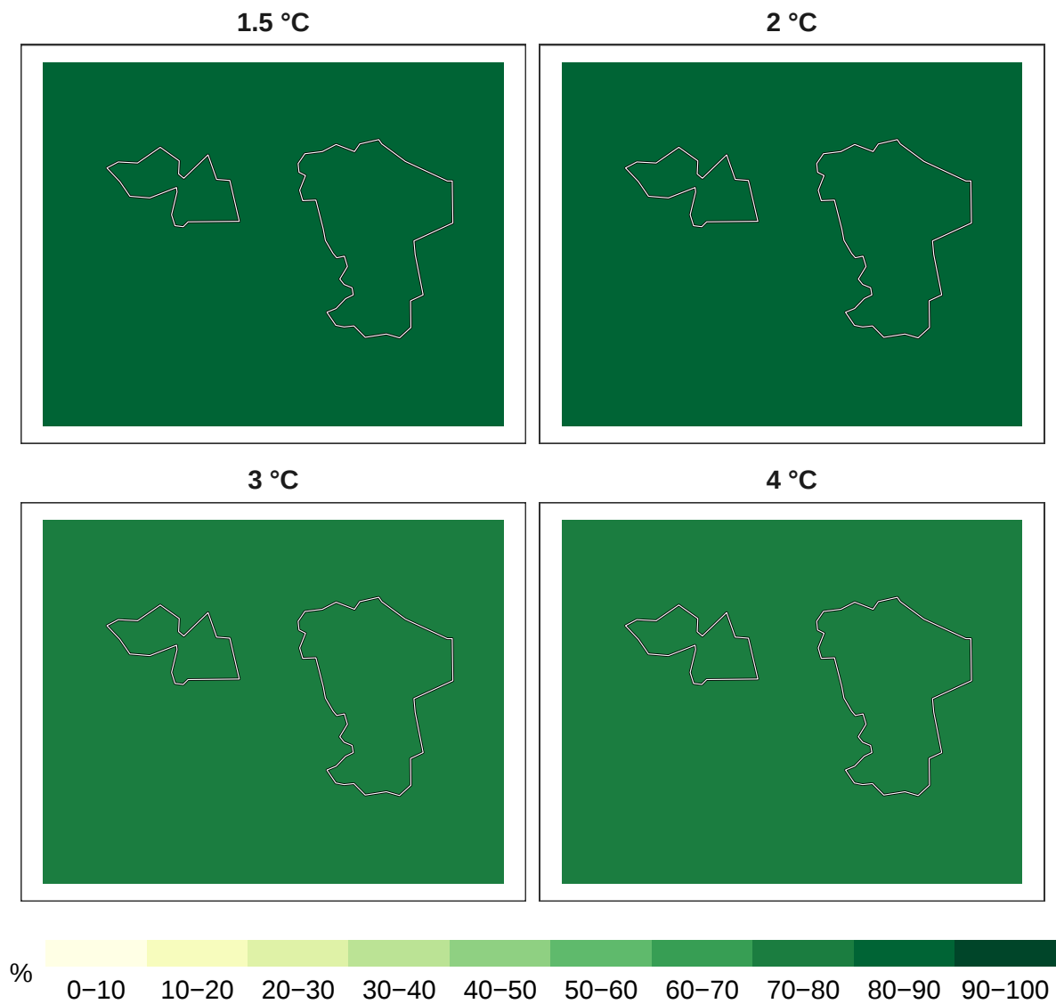
Figure 3: Percent birds remaining at 1 km resolution.
