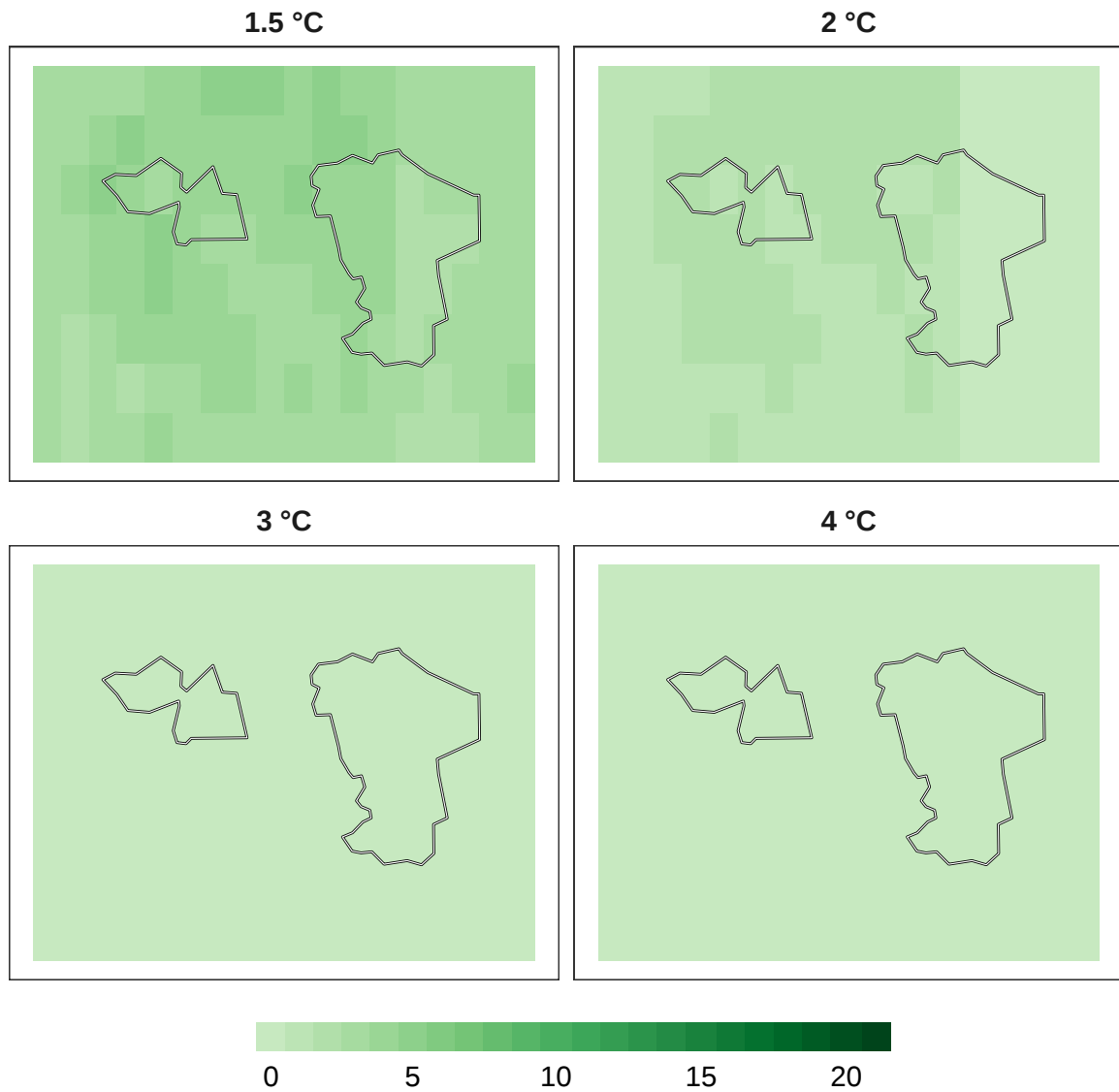
Figure 9: Number of models in agreement for overall biodiversity refugia at 1 km resolution.
