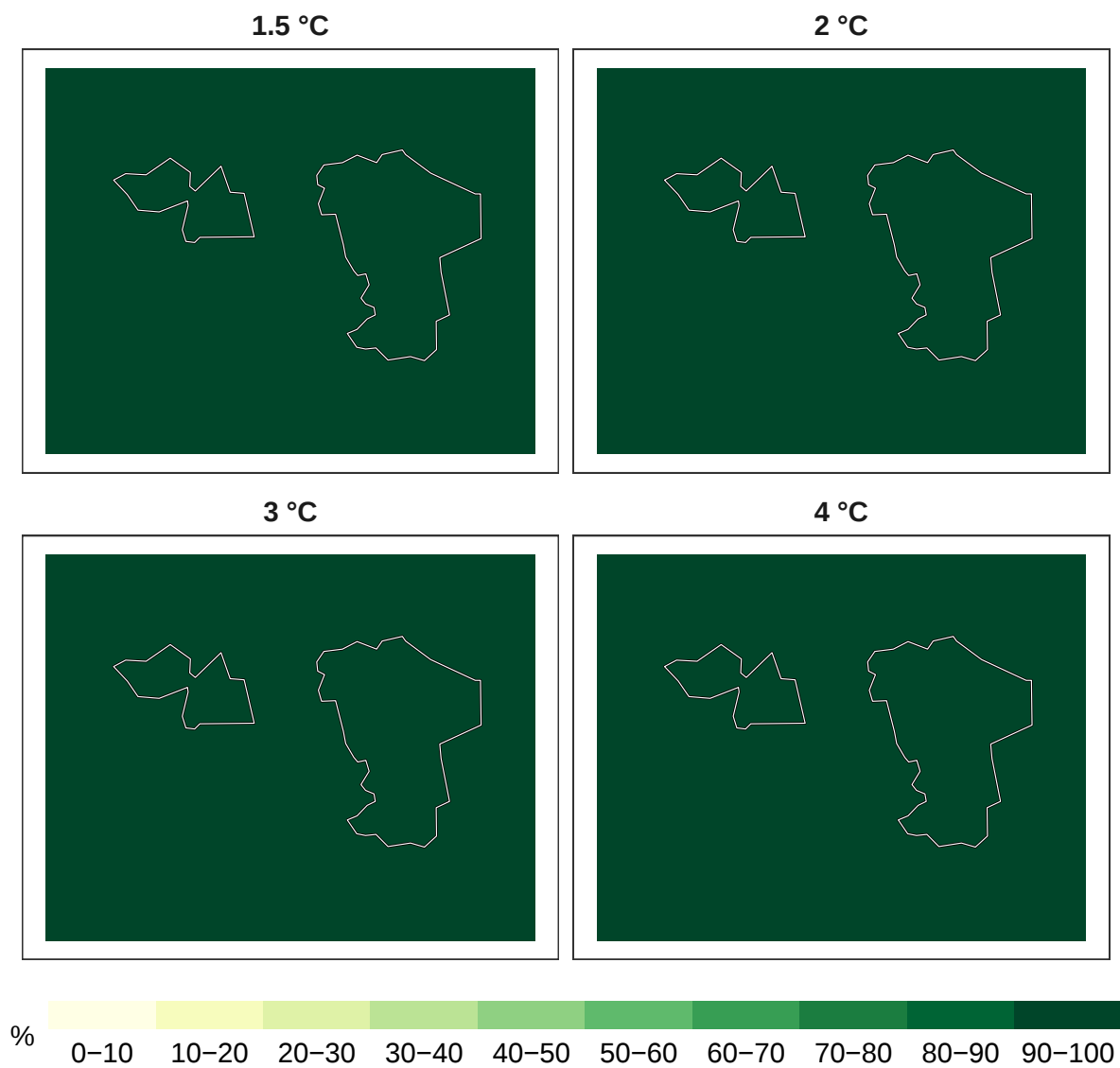
Figure 5: Percent reptiles remaining at 1 km resolution.
