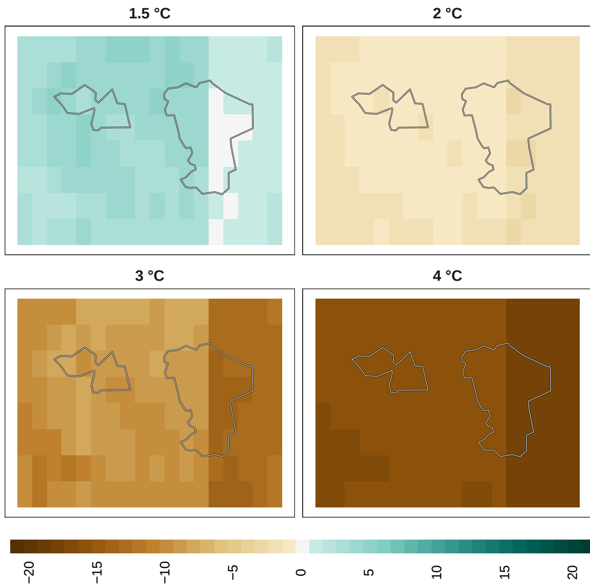
Figure 21: Adaptation effort for insects at 1 km resolution.
