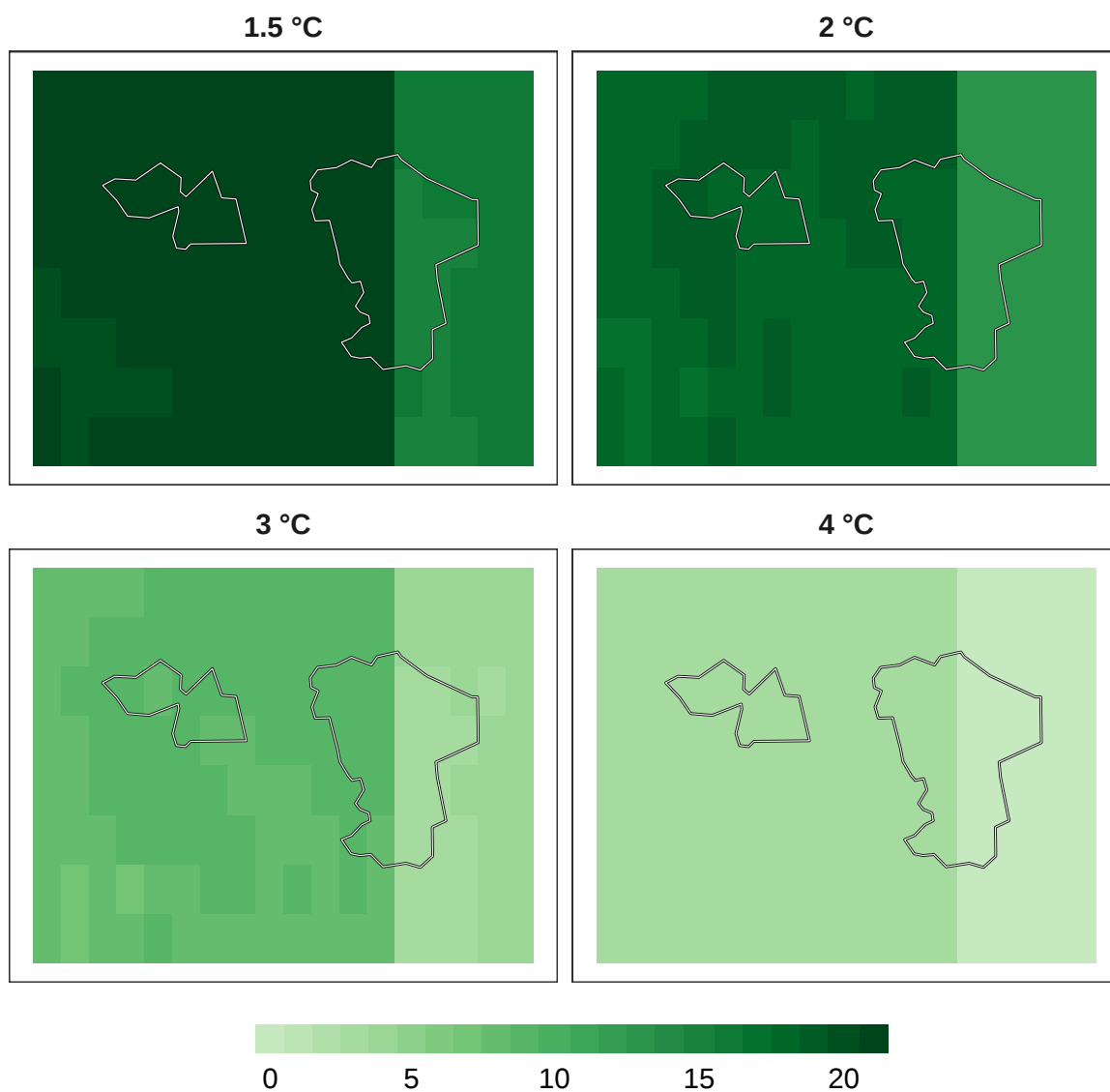
Figure 12: Number of models in agreement for mammal refugia at 1 km resolution.
