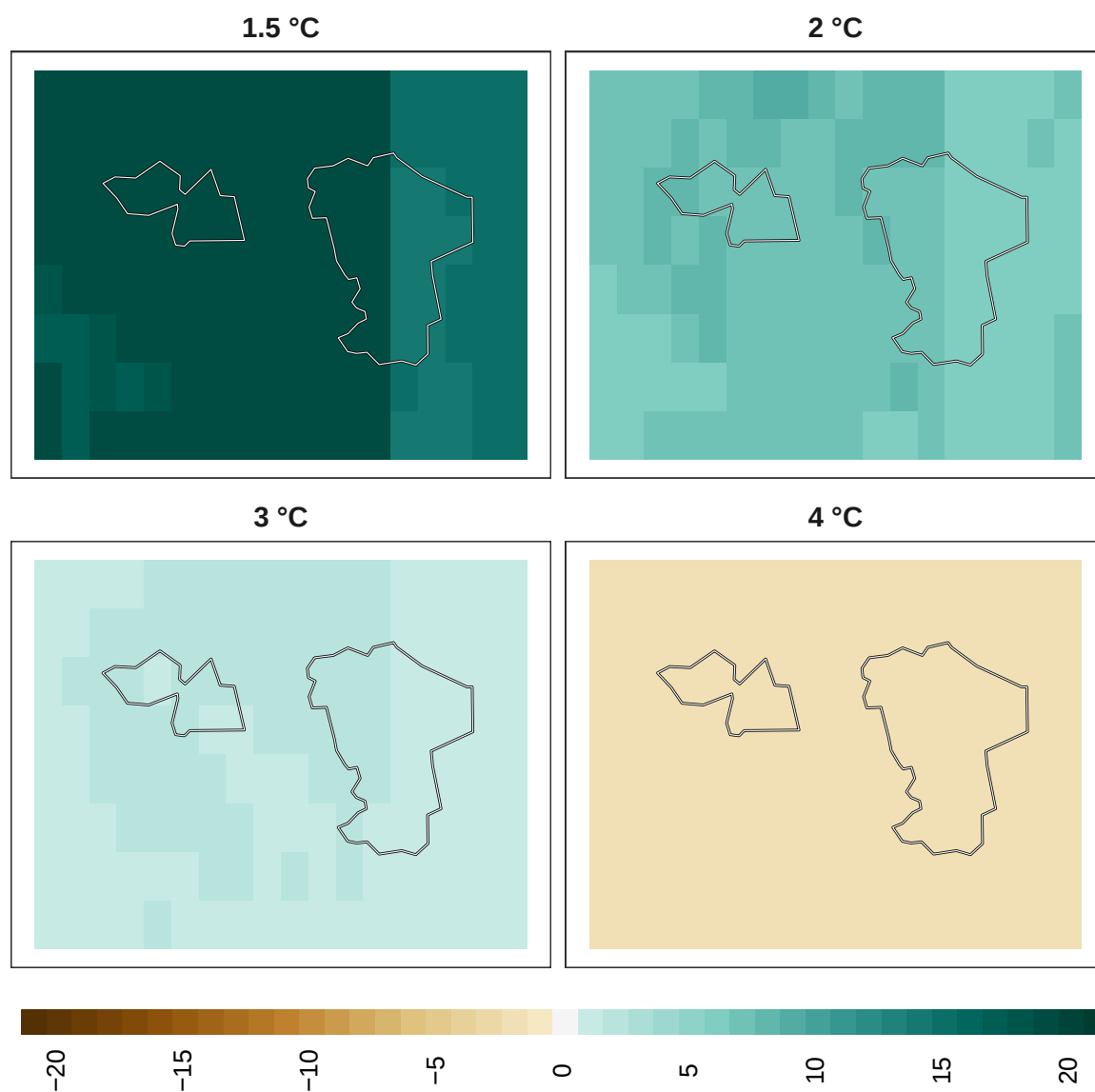
Figure 17: Adaptation effort for plants at 1 km resolution.
