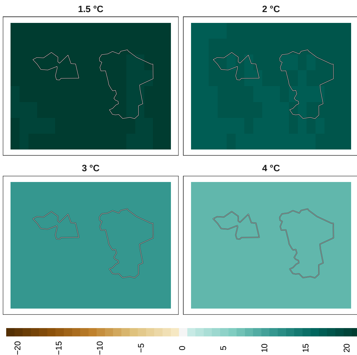
Figure 18: Adaptation effort for birds at 1 km resolution.
