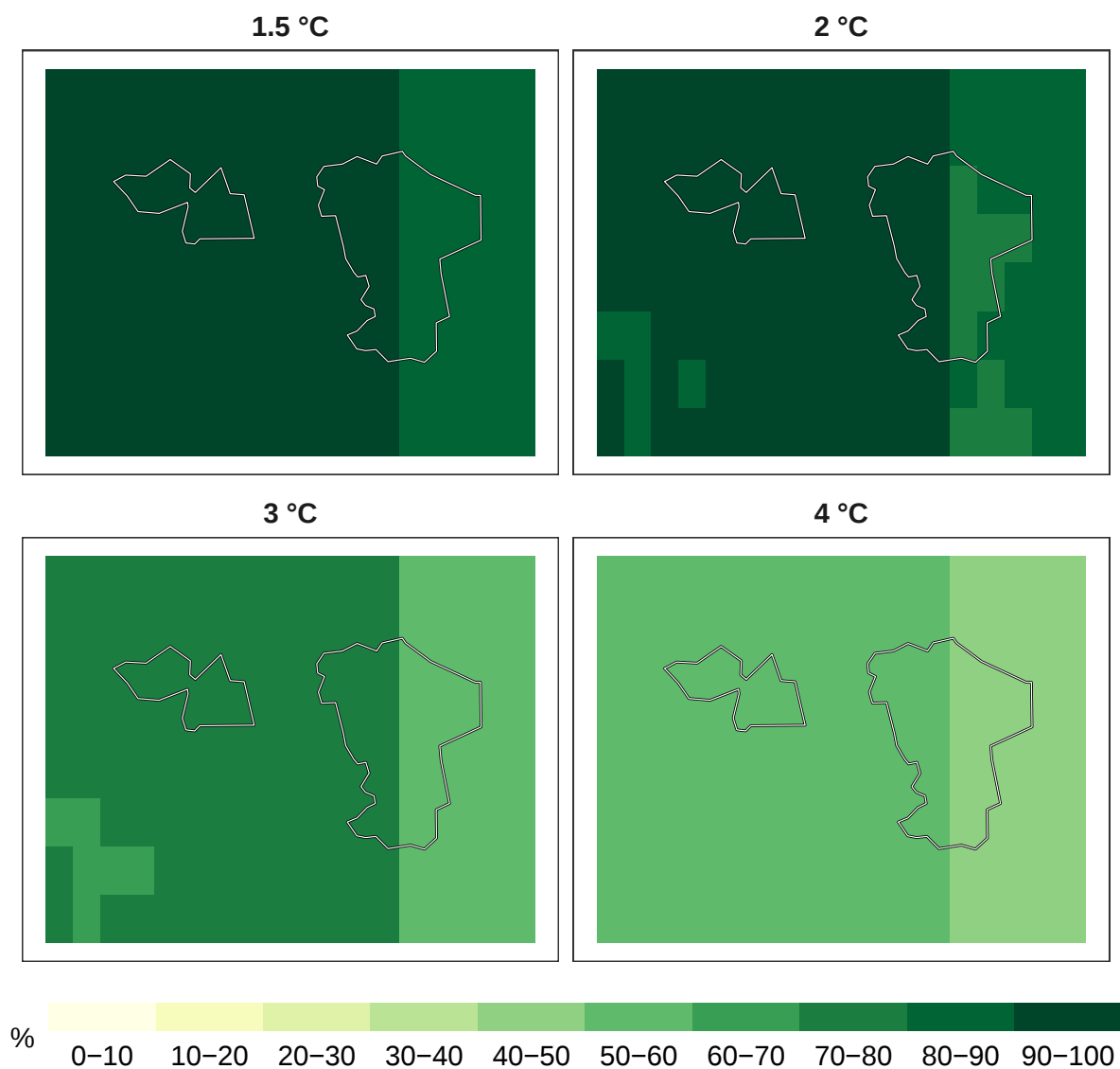
Figure 4: Percent mammals remaining at 1 km resolution.
