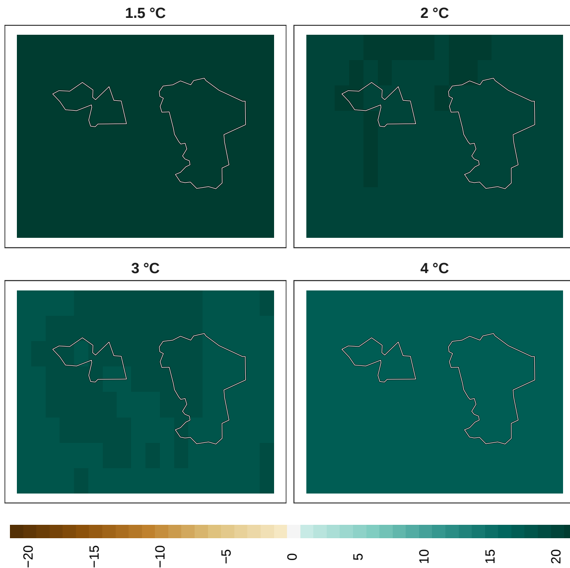
Figure 20: Adaptation effort for reptiles at 1 km resolution.
