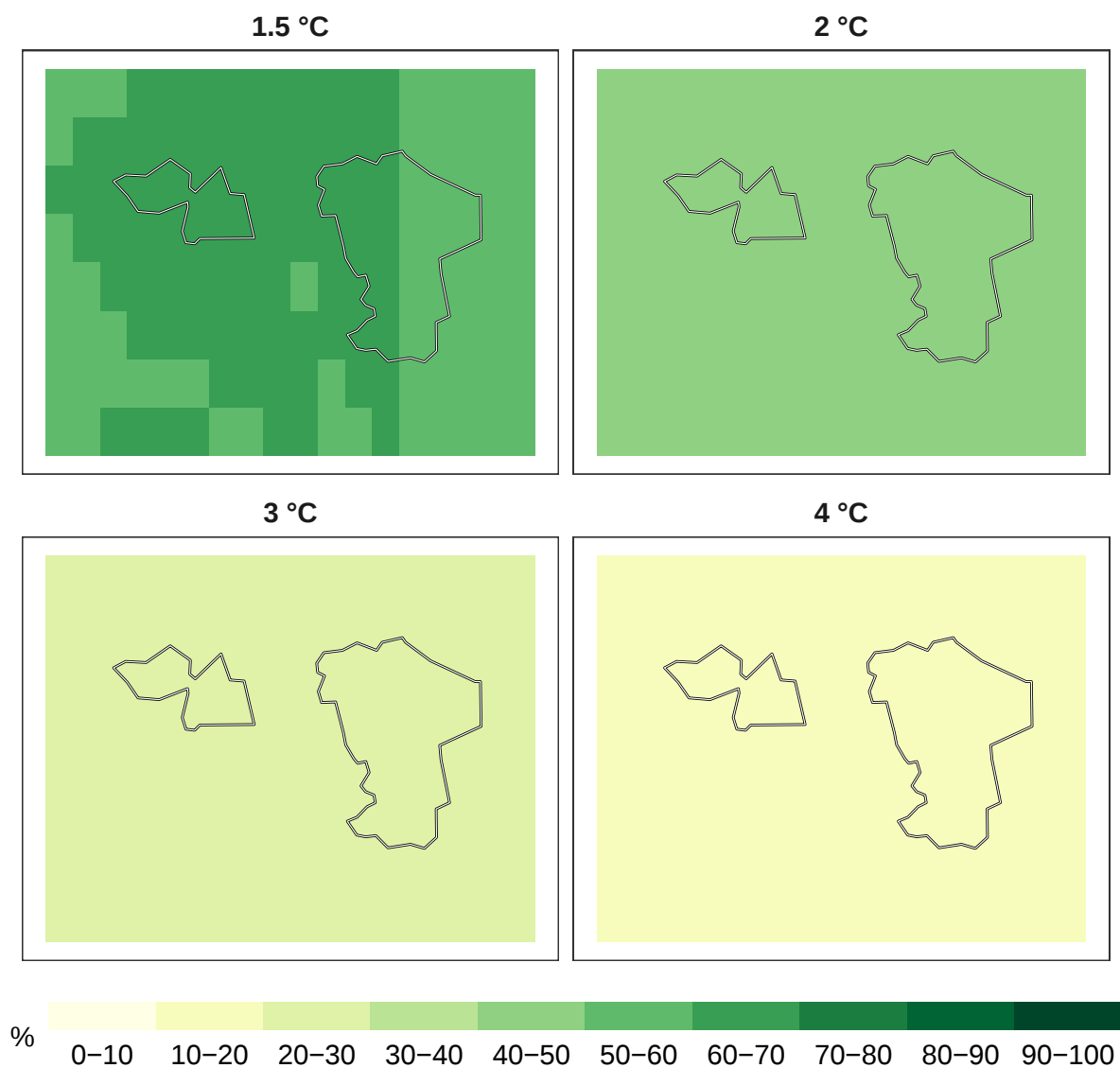
Figure 6: Percent insects remaining at 1 km resolution.
