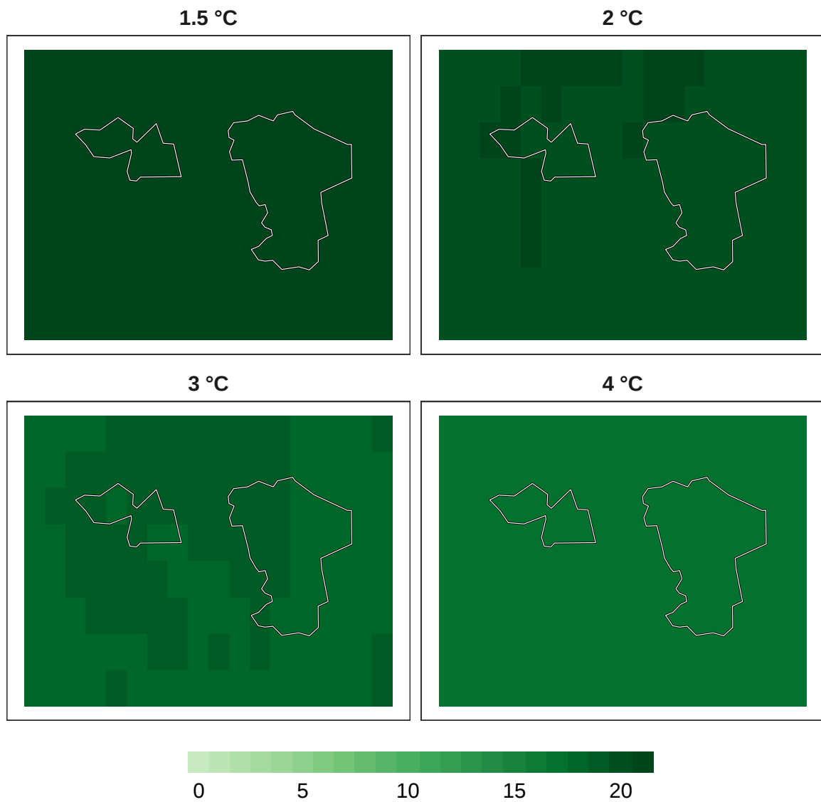
Figure 13: Number of models in agreement for reptile refugia at 1 km resolution.
