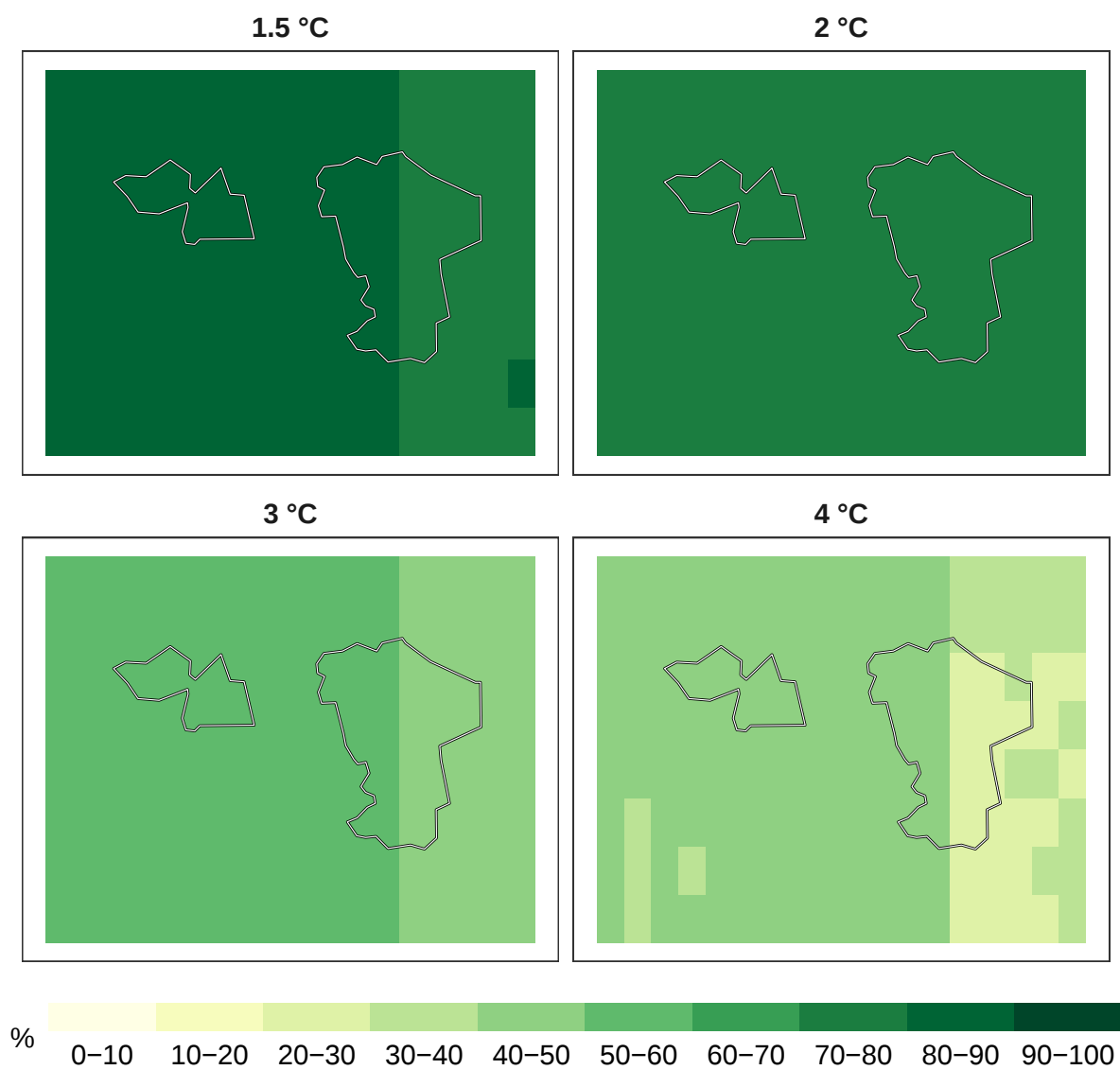
Figure 8: Percent timber species remaining at 1 km resolution.
