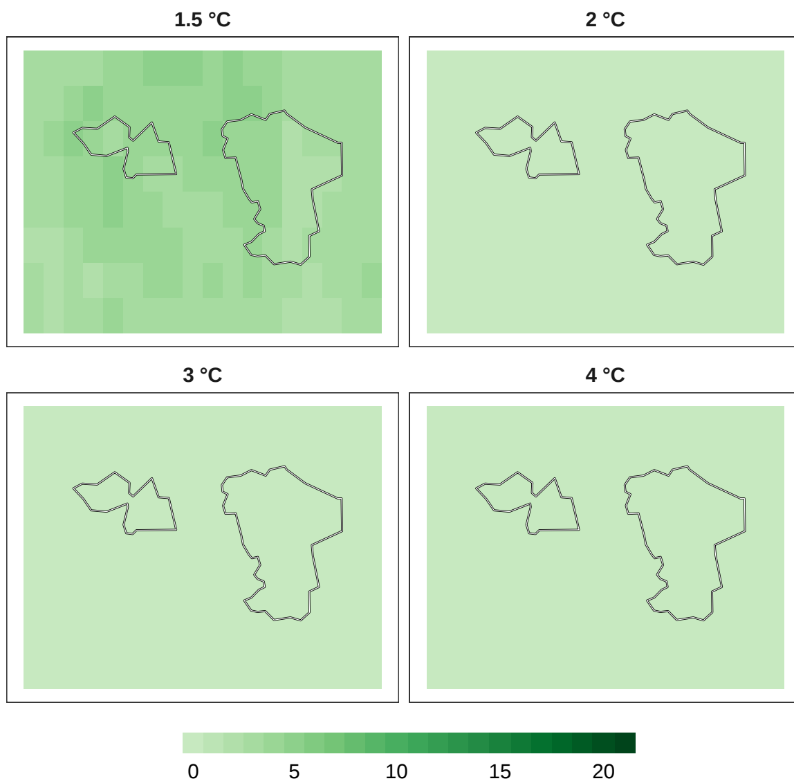
Figure 15: Number of models in agreement for pollinator refugia at 1 km resolution.
