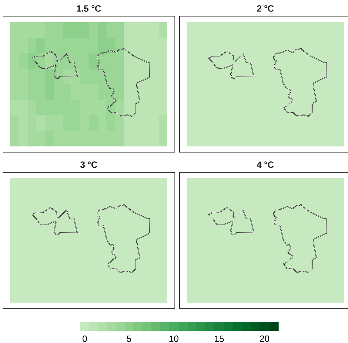
Figure 14: Number of models in agreement for insect refugia at 1 km resolution.
