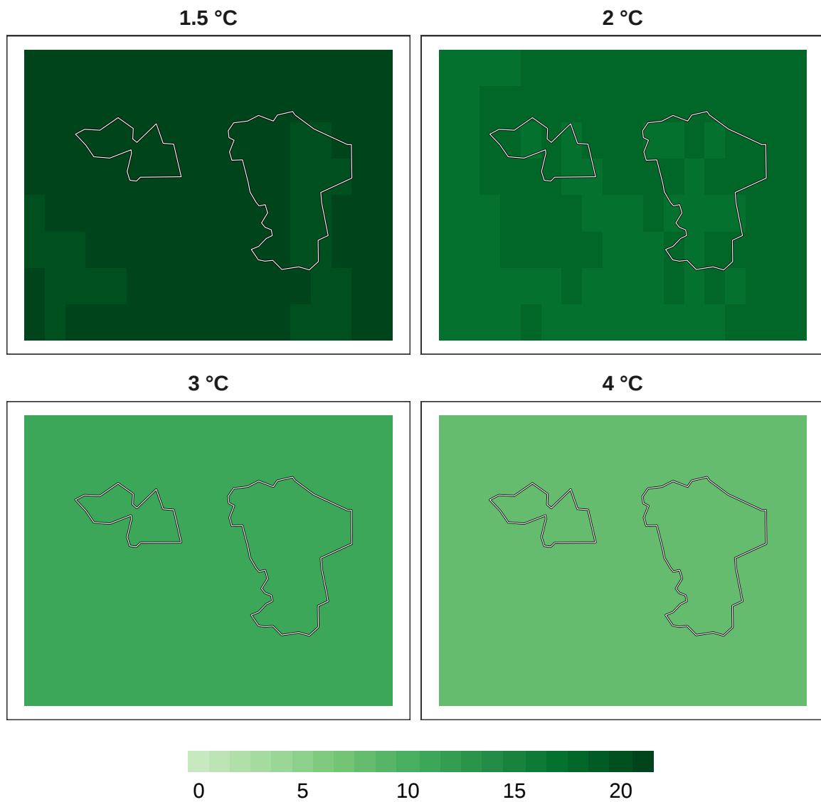
Figure 11: Number of models in agreement for bird refugia.
