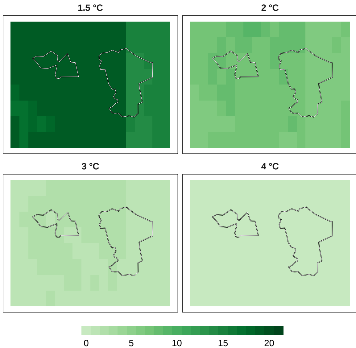
Figure 10: Number of models in agreement for plant refugia at 1 km resolution.
