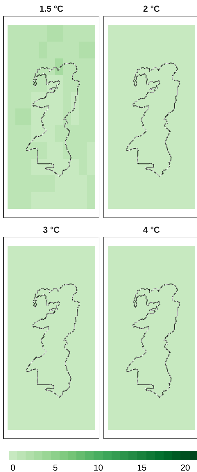
Figure 9: Number of models in agreement for plant refugia at 1 km resolution.
