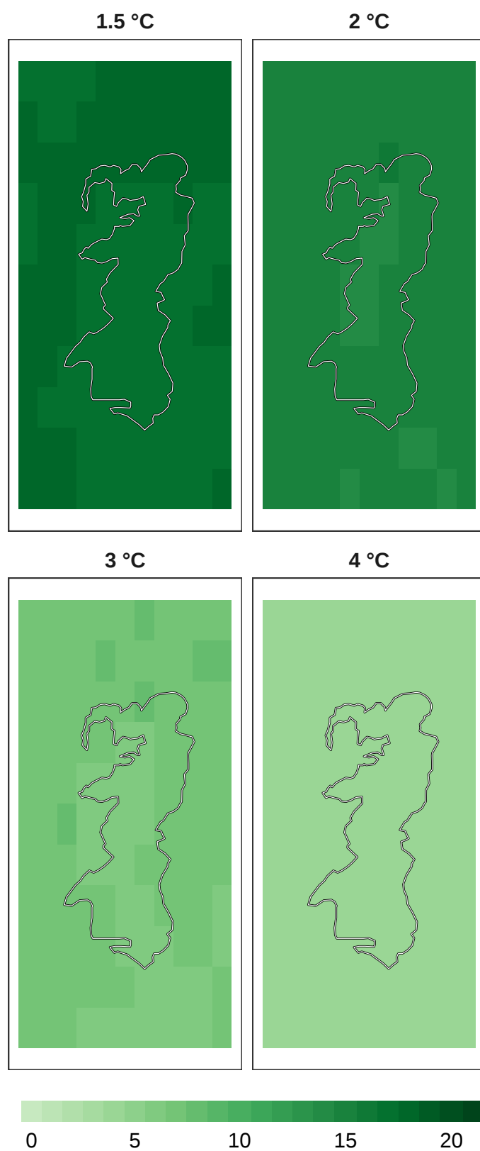
Figure 10: Number of models in agreement for bird refugia.
