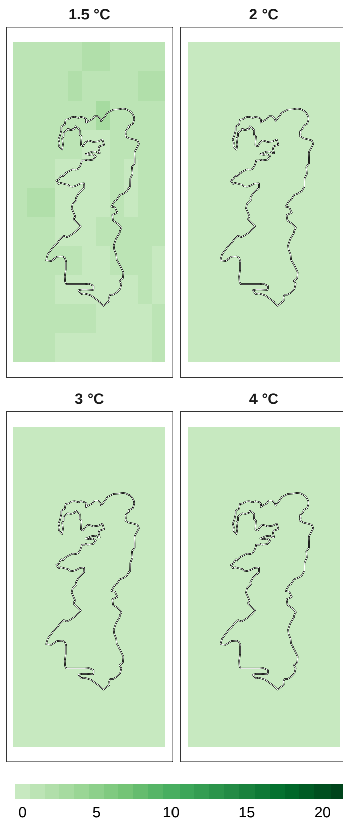
Figure 12: Number of models in agreement for insect refugia at 1 km resolution.
