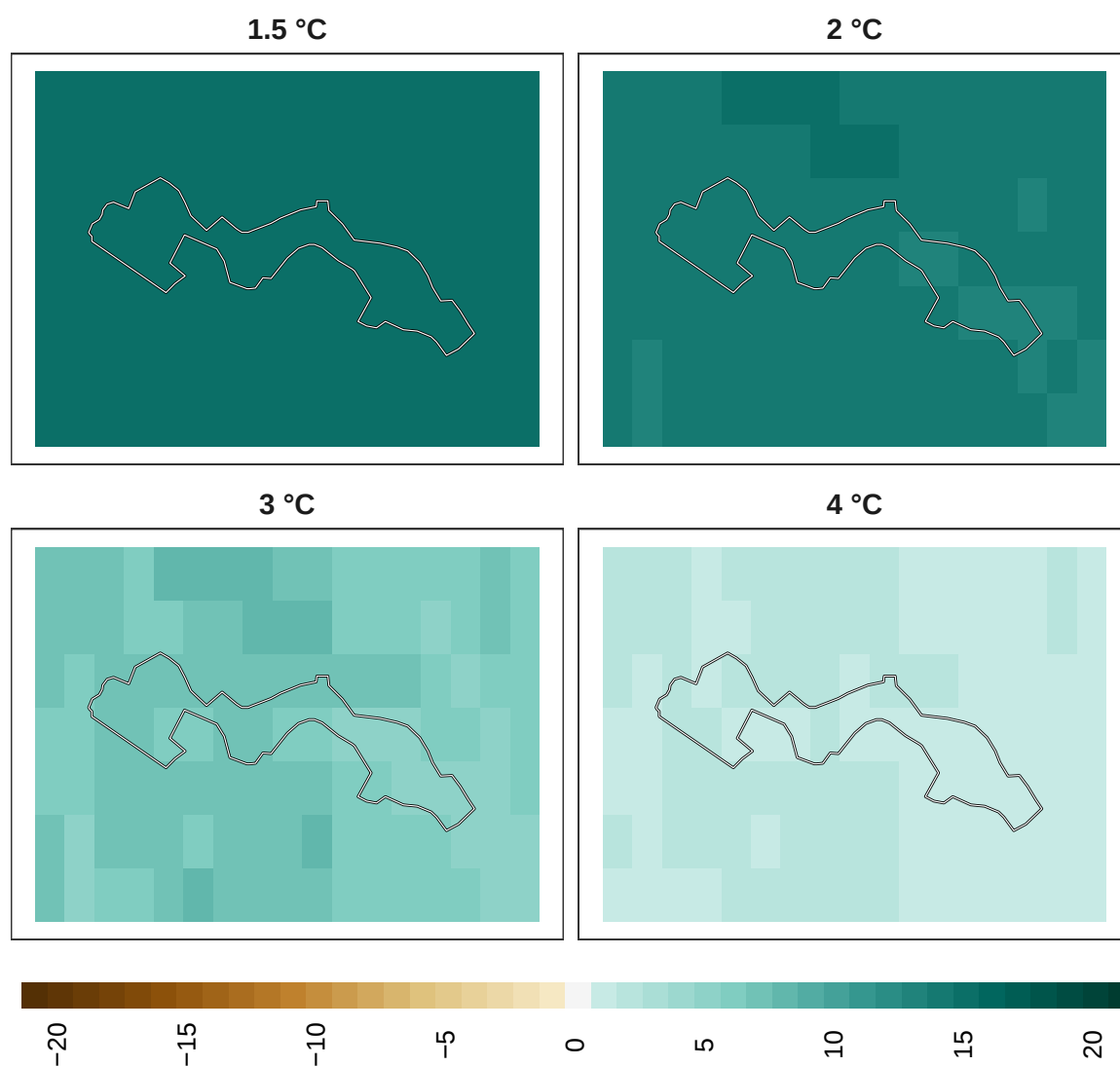
Figure 19: Adaptation effort for mammals at 1 km resolution.
