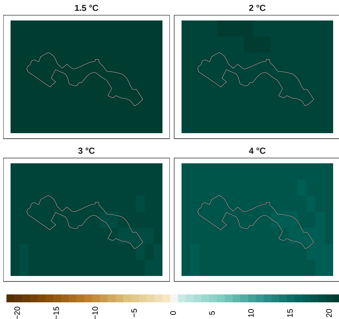
Figure 20: Adaptation effort for reptiles at 1 km resolution.
