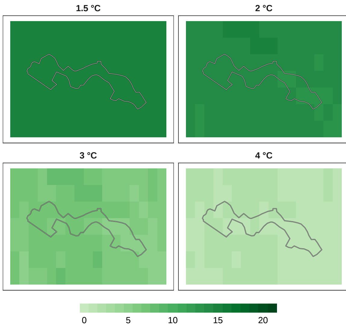
Figure 12: Number of models in agreement for mammal refugia at 1 km resolution.
