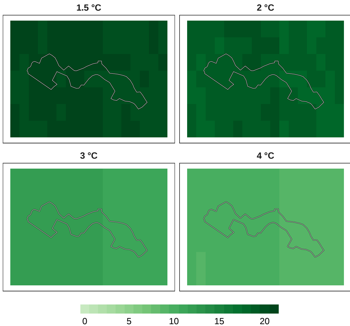
Figure 11: Number of models in agreement for bird refugia.
