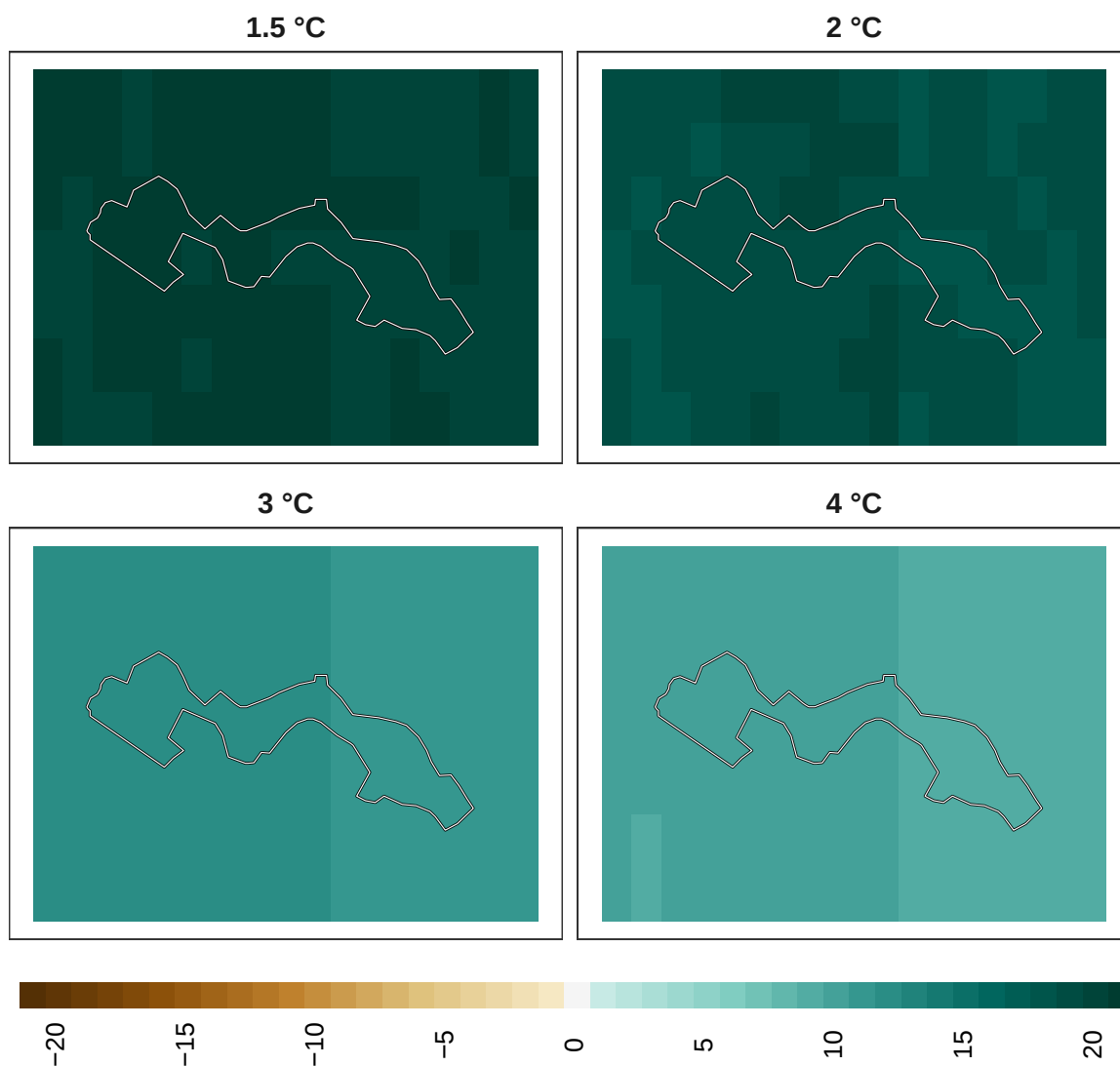
Figure 18: Adaptation effort for birds at 1 km resolution.
