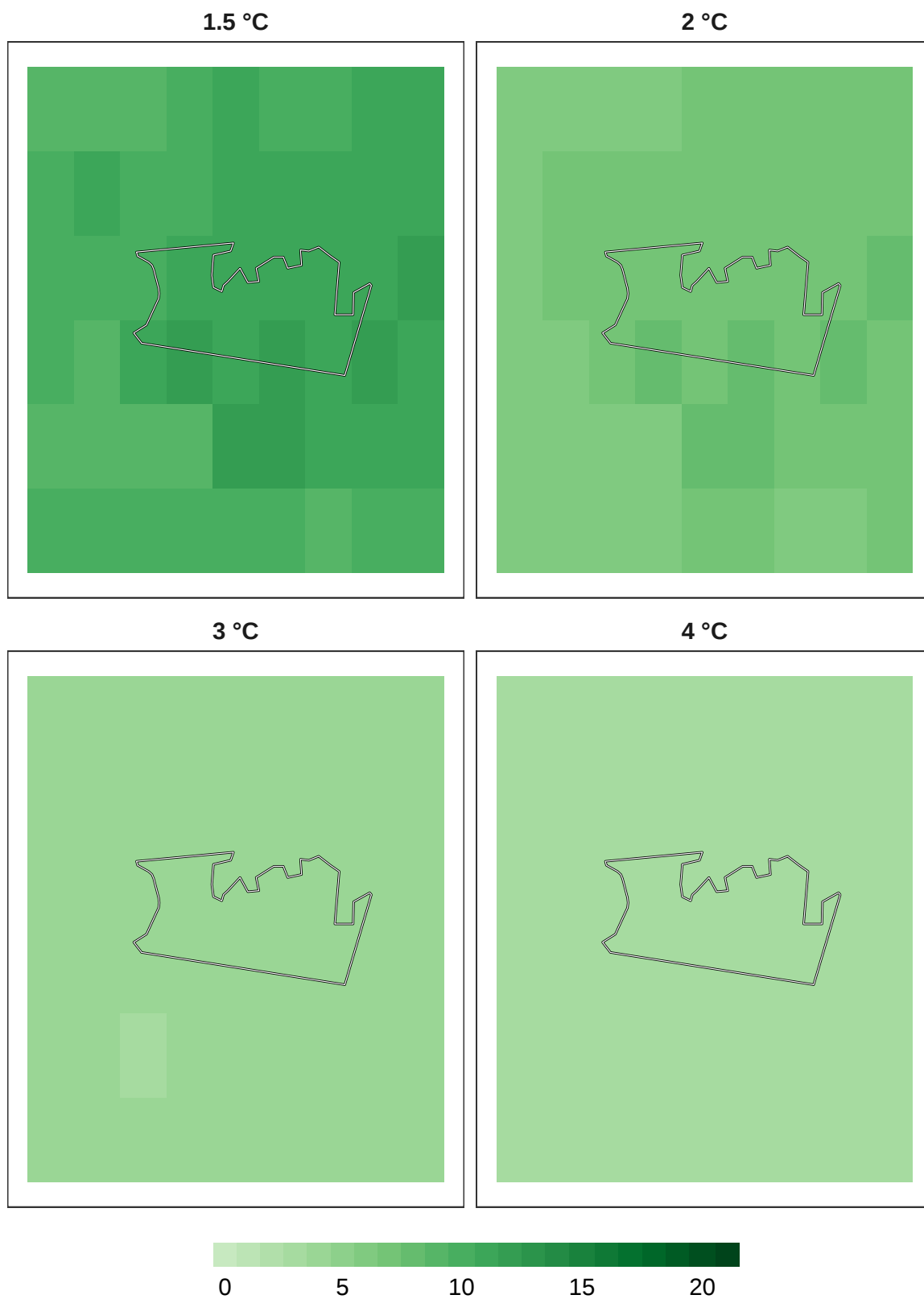
Figure 13: Number of models in agreement for reptile refugia at 1 km resolution.
