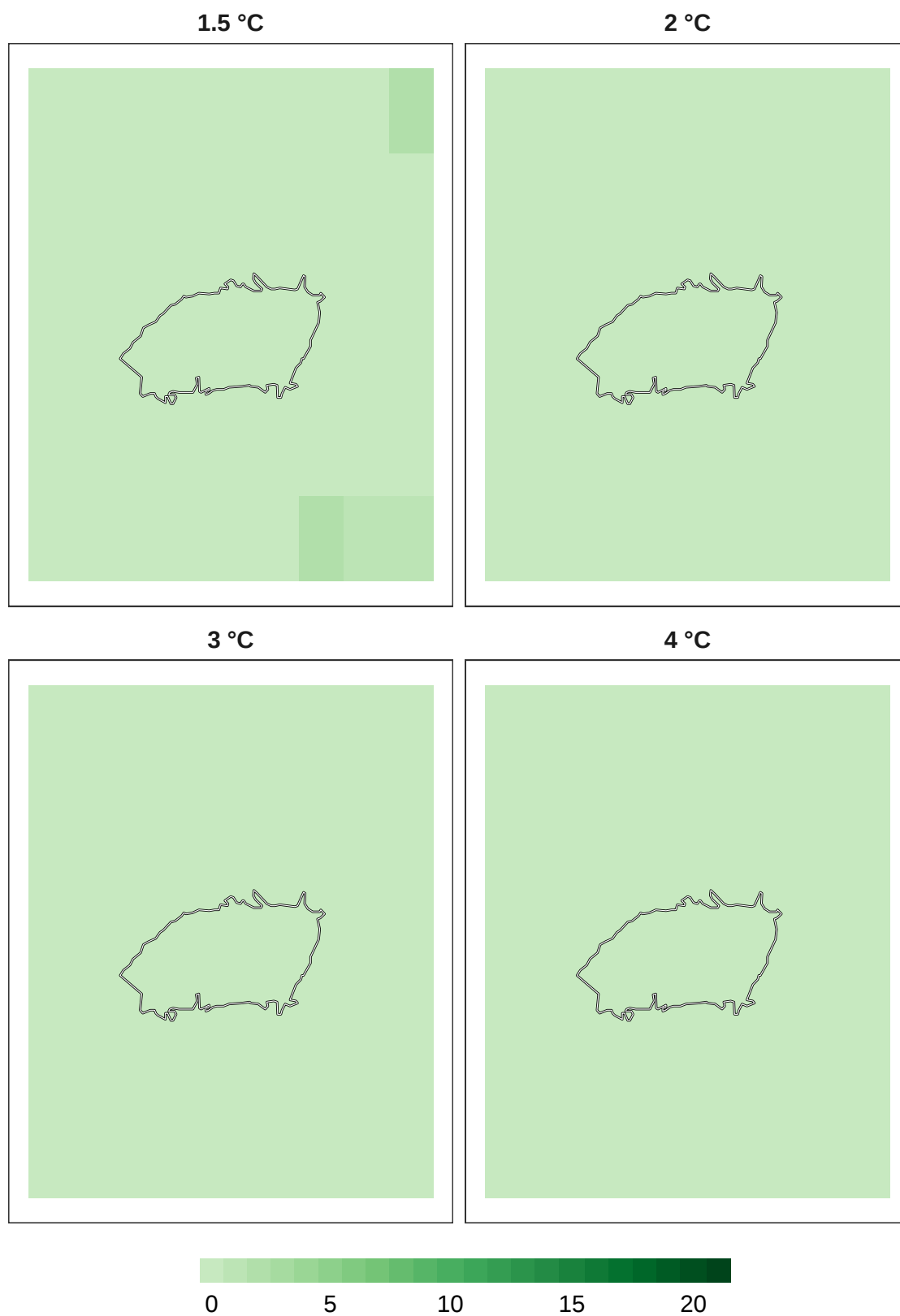
Figure 12: Number of models in agreement for pollinator refugia at 1 km resolution.
