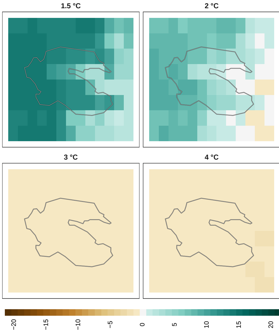
Figure 18: Adaptation effort for reptiles at 1 km resolution.
