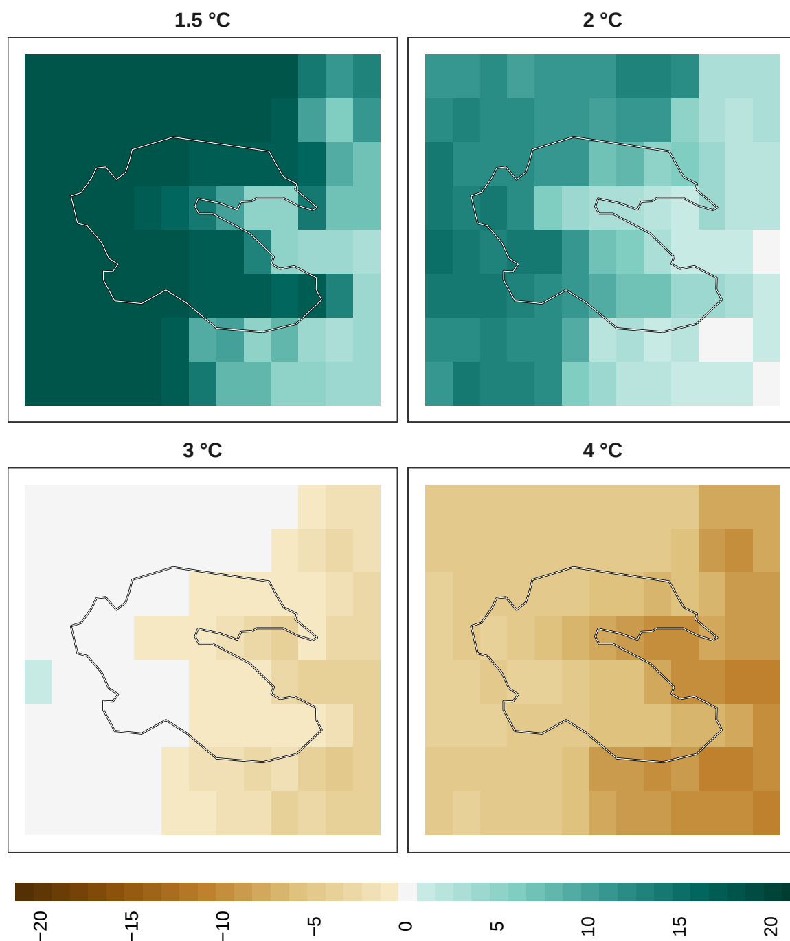
Figure 19: Adaptation effort for insects at 1 km resolution.
